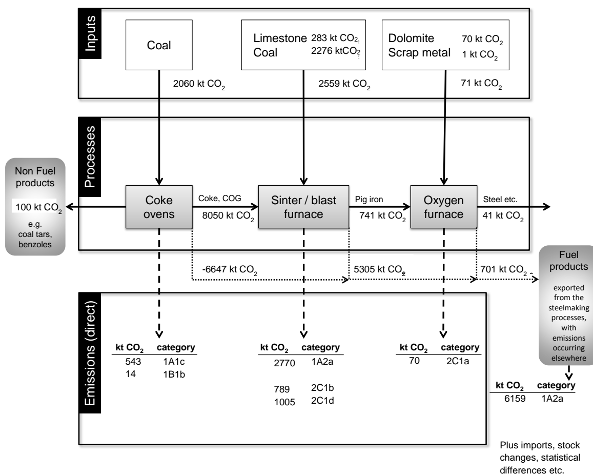
Figure 3.1 Carbon balance model for 2023 a
