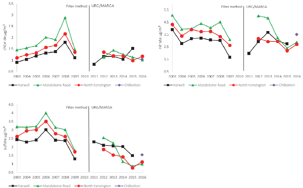
Figure 4-4 Anion long-term annual trends (clockwise chloride, nitrate and sulphate). The 2012 - 2016 data for Harwell have been derived from the MARGA measurements.
