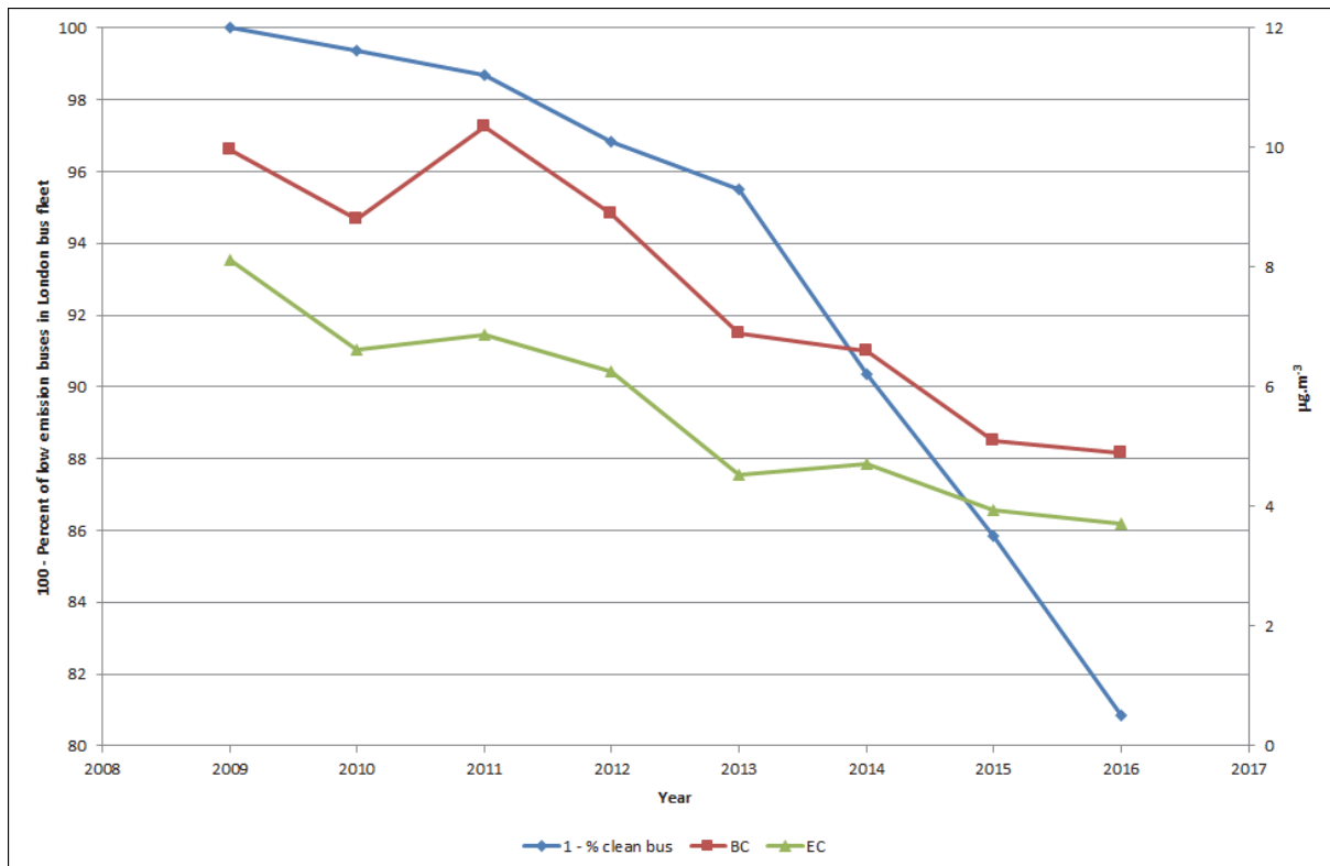
Figure 4-3 Annual Average Black Carbon, Elemental Carbon and [100 – percentage of low emission buses in the London bus fleet] for the period 2009 – 2016.
