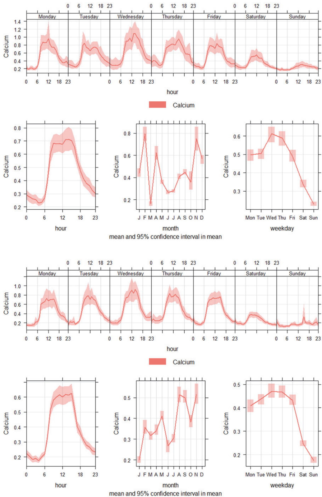
Figure 4-25 Diurnal, weekly and monthly profiles for Ca 2+ during 2016 at North Kensington (top) and Marylebone Road (bottom).
