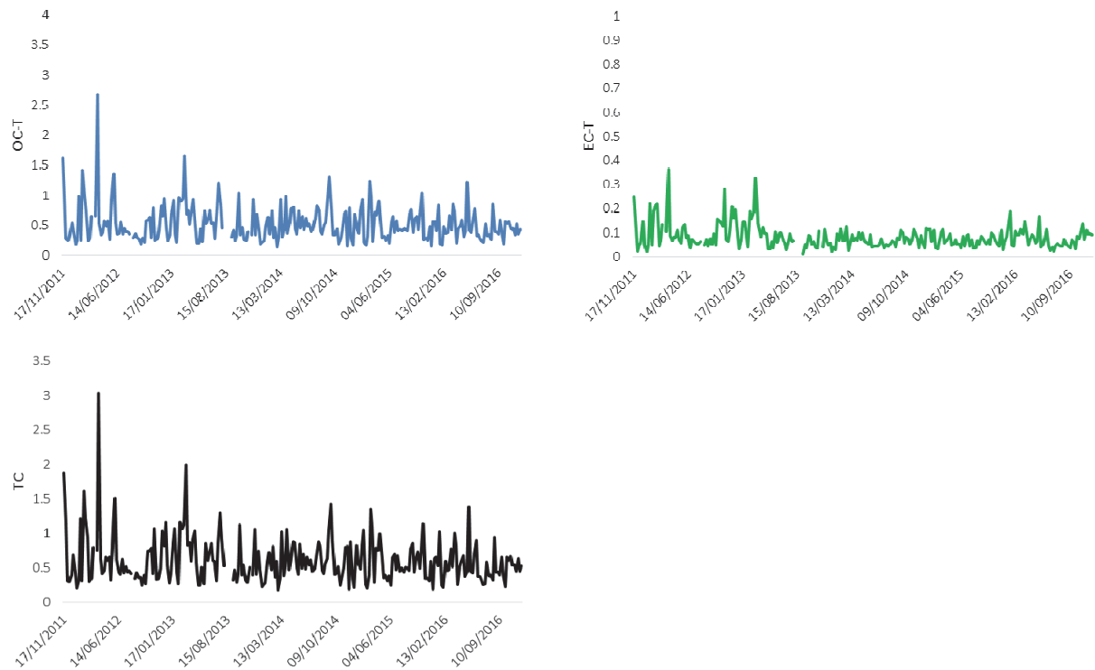
Figure 4-5 Time series of OC, EC and TC in the PM 2.5 fraction at Auchencorth Moss since the installation of the sampler (weekly samples) ( \mu\text{g}/\text{m}^3 )
