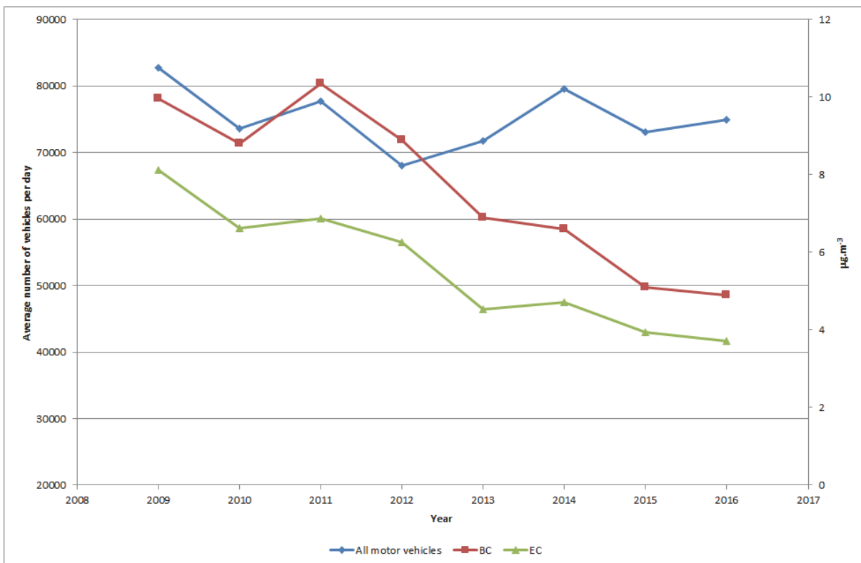
Figure 4-19 Annual Average Black Carbon, Elemental Carbon and Motor Vehicles per day at Marylebone Road for the period 2009 – 2016
