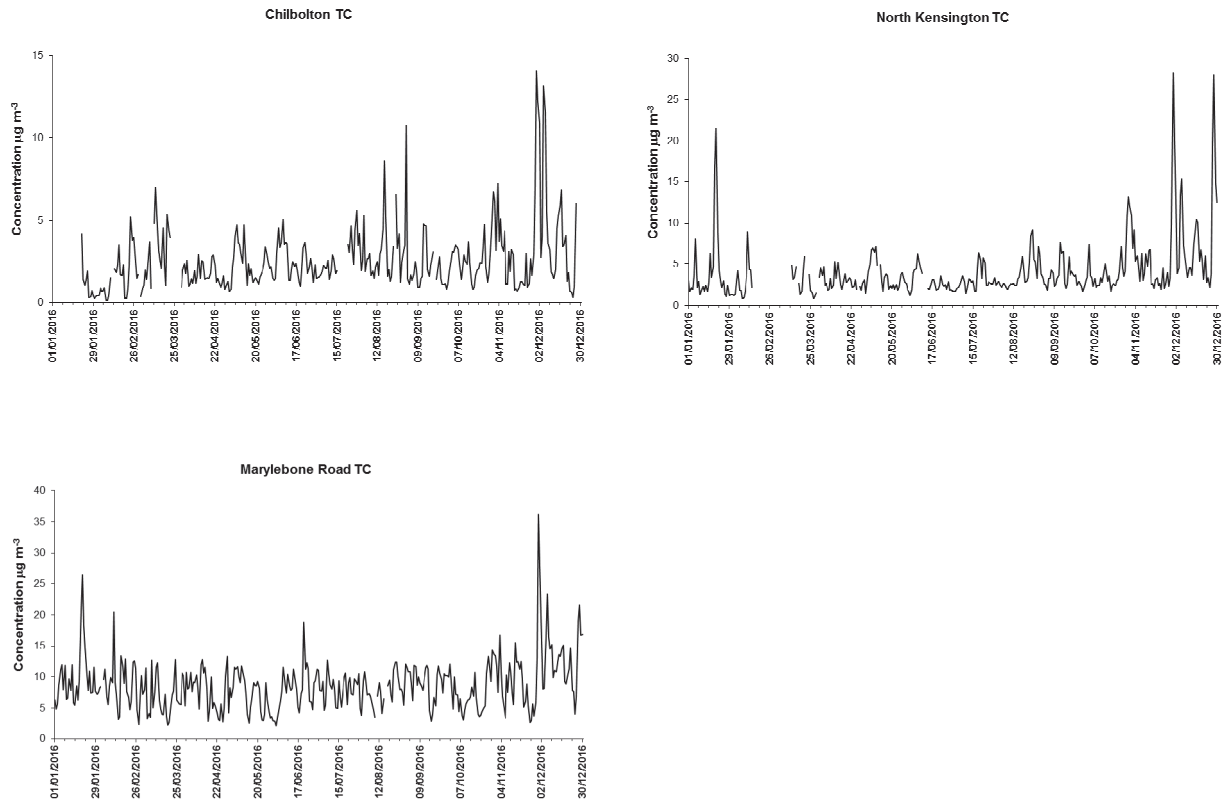
Figure 4-2 PM 10 TC concentrations at Chilbolton, North Kensington and Marylebone Road during 2016
