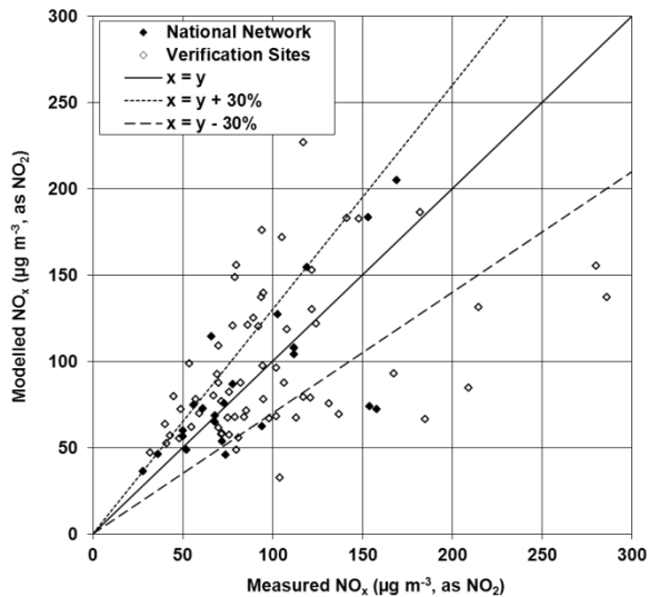
Figure 3.19 - Verification of roadside annual mean NO x model 2011
