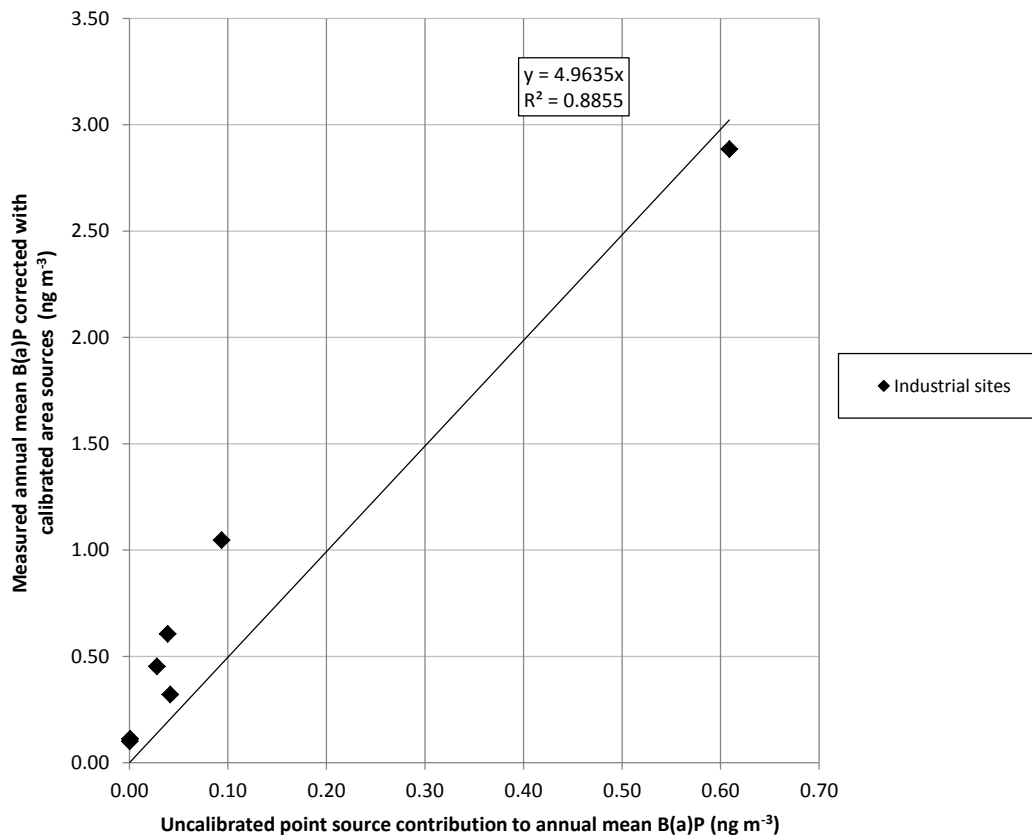
Figure 11.5 - Calibration of point source model for B(a)P
