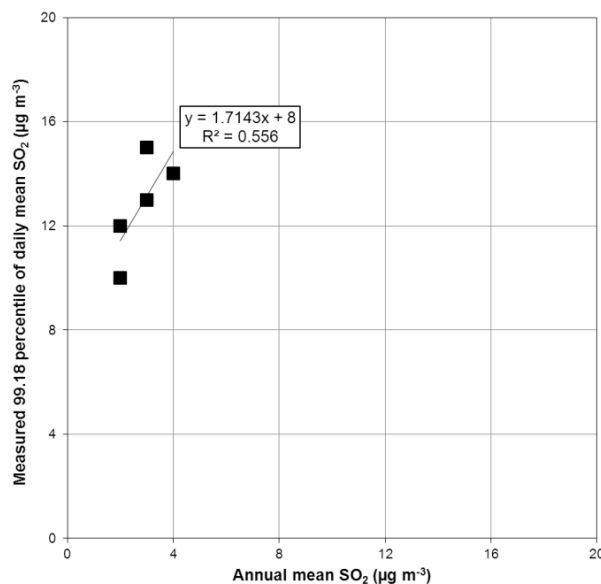
Figure 4.10 - Relationship between mean concentration and 99.18 percentile of 24-hour concentrations at sampling sites in Northern Ireland, 2011
