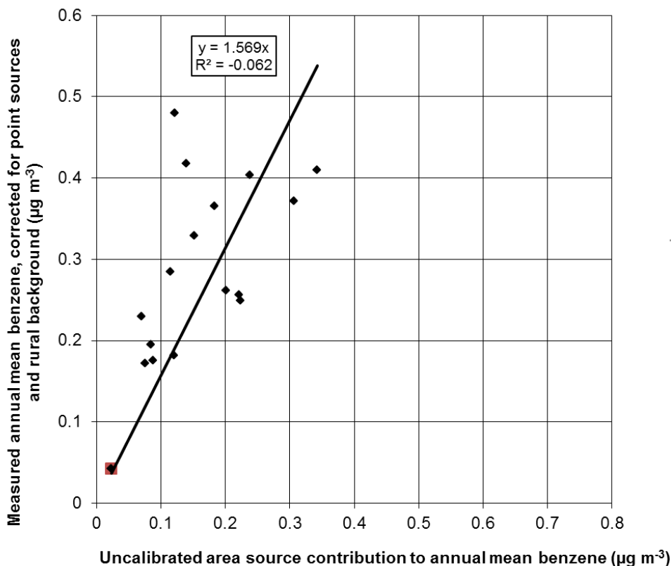
Figure 7.4 - Calibration of area source benzene model, 2011 ( \mu\text{g m}^{-3} )
