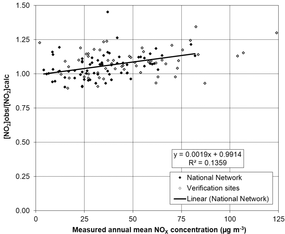
Figure 3.15 - Background NO 2 calibration curve (NB verification sites are shown for reference here, but were not used in calculating the calibration), 2011
