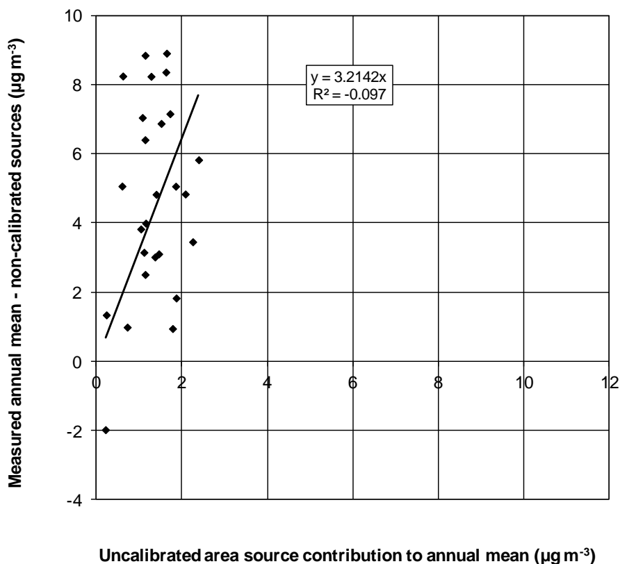
Figure 5.8 - Calibration of PM 10 area source model 2011 ( \mu\text{g m}^{-3} , gravimetric)
