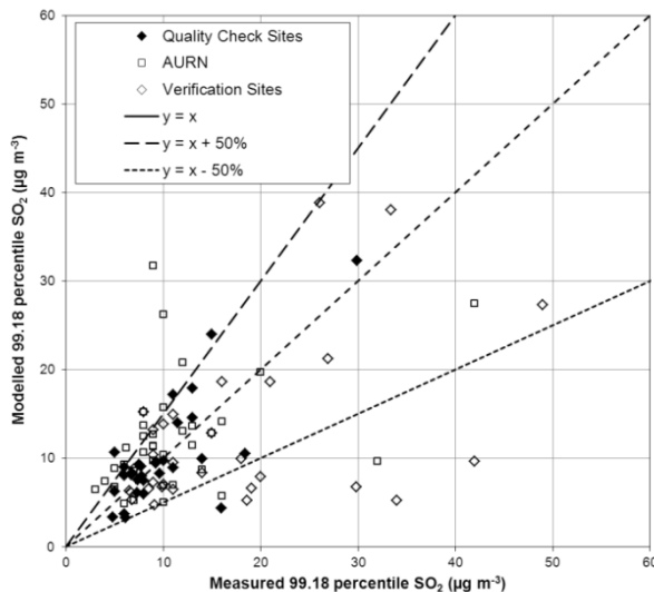
Figure 4.13 - Verification of 99.18 percentile of 24-hour mean SO 2 model, 2011
