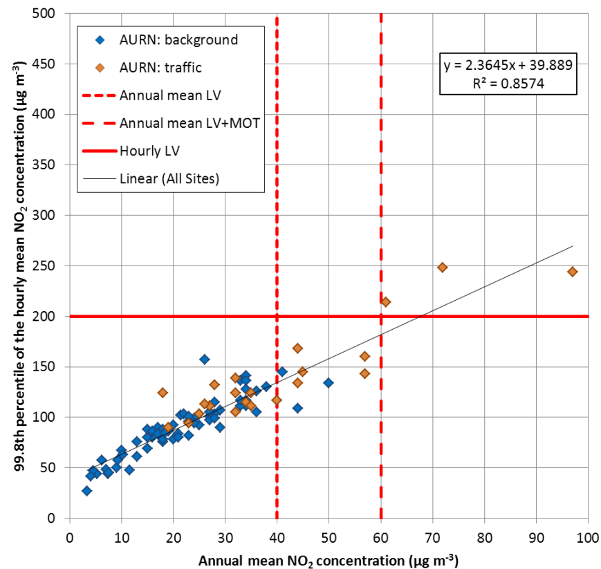
Figure 3.4 - Plot of annual mean against 99.8th percentile hourly NO 2 concentrations in 2011
