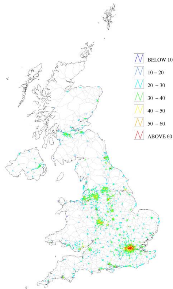
Figure 3.2 - Urban major roads, annual mean roadside \text{NO}_2 concentration, 2011 ( \mu\text{g m}^{-3} )
