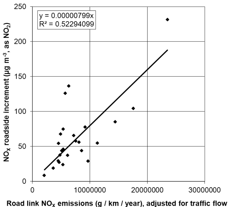
Figure 3.8 - Calibration of NO x roadside increment model, 2011 ( \mu\text{g m}^{-3} , as NO 2 )
