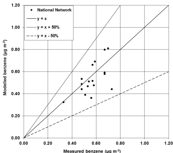
Figure 7.6 - Verification of background annual mean benzene model 2011
