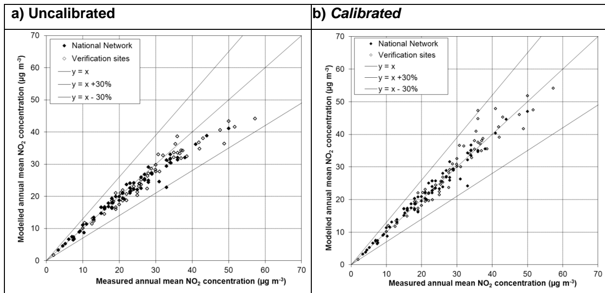
Figure 3.16 - Verification of category 4 (IIIa) relationship at background locations in 2011
