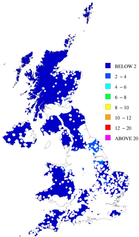
Figure 4.1 - Annual mean SO 2 concentration, 2011 ( \mu\text{g m}^{-3} ) in vegetation areas
