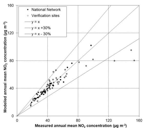
Figure 3.14 - Verification of category 4 (IIIa) relationship at roadside locations in 2011
