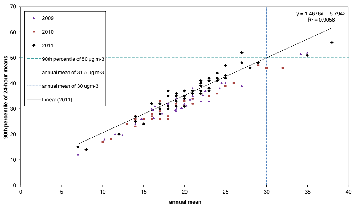
Figure 5.3 - The relationship between the 90th percentile of 24-hour mean \text{PM}_{10} concentration and annual mean concentration ( \mu\text{g m}^{-3} ) for 2011
