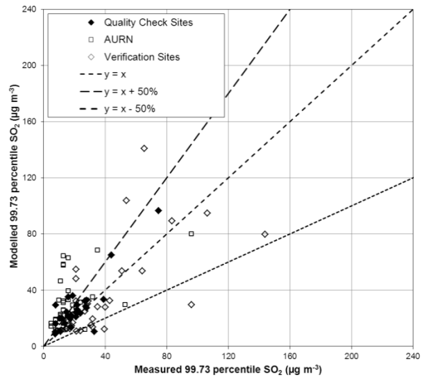
Figure 4.12 - Verification of 99.73 percentile of 1-hour mean SO 2 model, 2011
