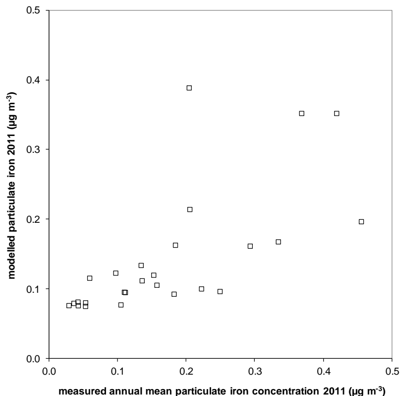
Figure 5.7 - Comparison of modelled and measured annual mean elemental Fe concentrations 2011 ( \mu\text{g m}^{-3} )
