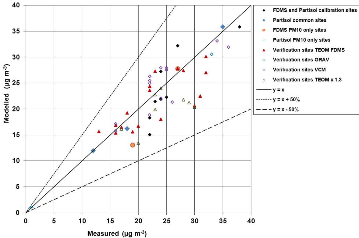
Figure 5.11 - Verification of roadside annual mean PM_{10} model 2011
