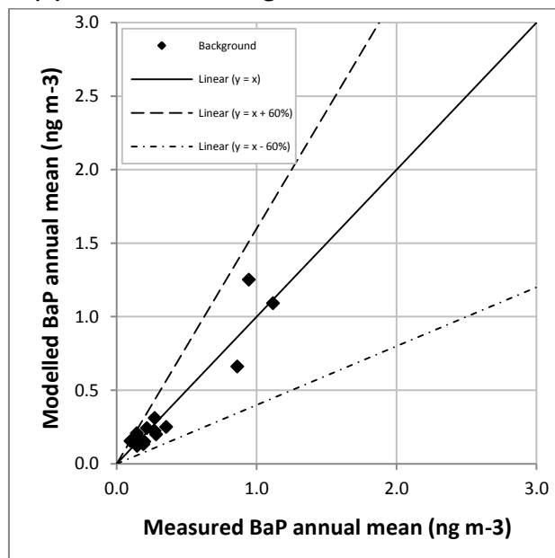
Figure 11.7 - Verification of annual mean B(a)P at urban background sites
