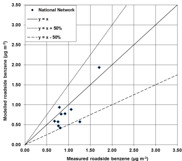
Figure 7.7 - Verification of roadside annual mean benzene model 2011
