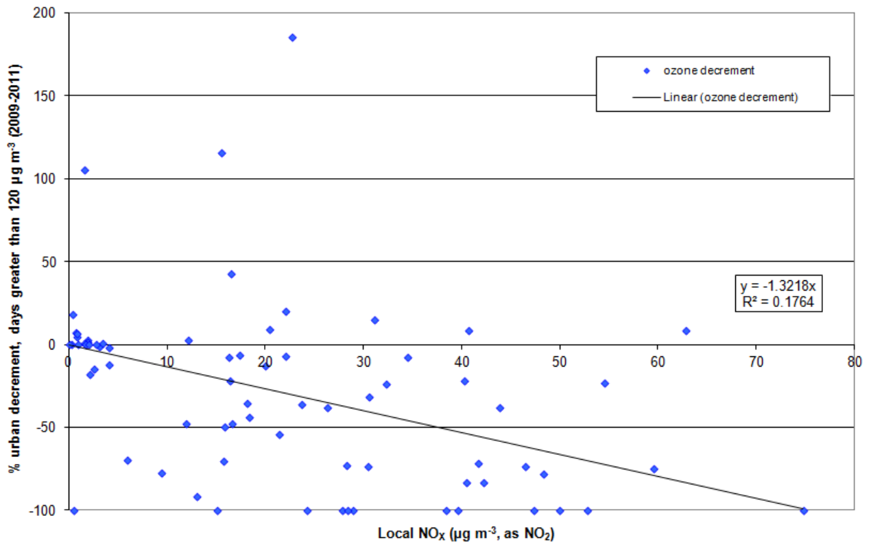
Figure 9.4 - Days greater than 120 \mu\text{g m}^{-3} percentage decrement in ozone concentrations, 2009-2011
