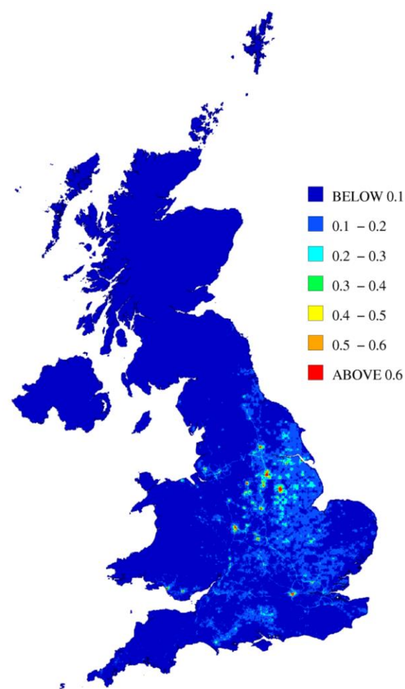
Figure 10.2 - Annual mean background Cadmium (Cd) concentration, 2011 (ng m -3 )
