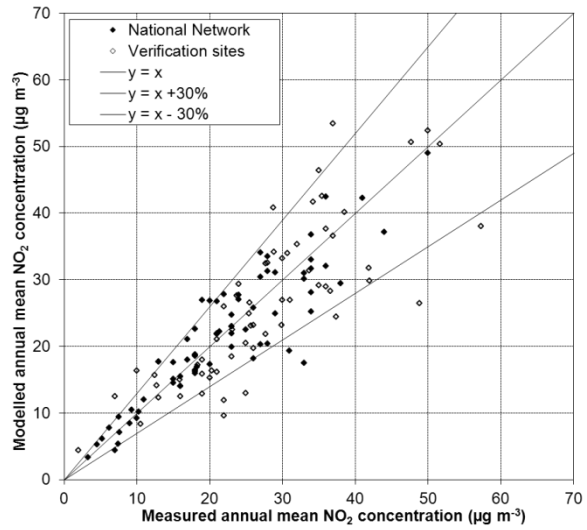
Figure 3.18 - Verification of background annual mean NO 2 model 2011
