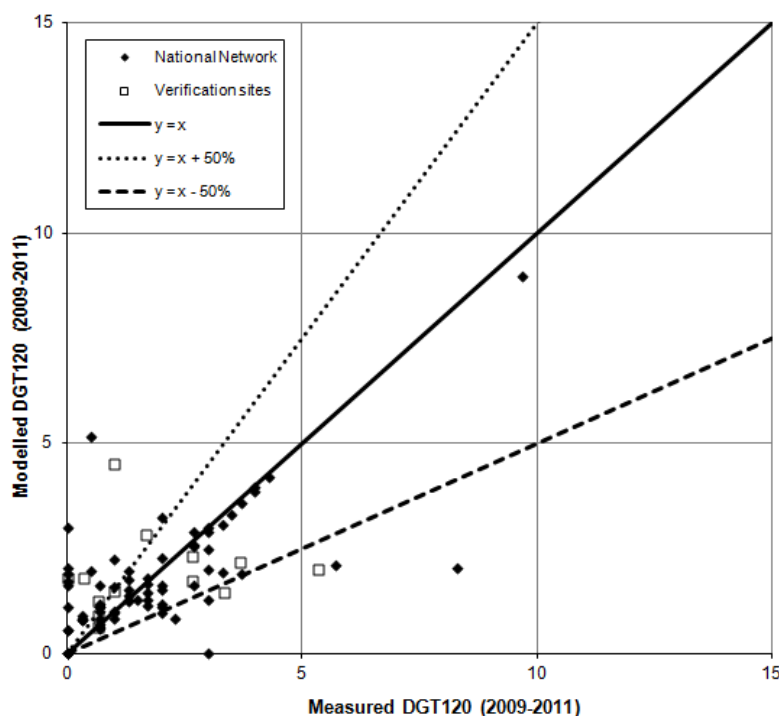
Figure 9.6 - Verification of background number of days > 120 \mu\text{g m}^{-3} model 2009-2011
