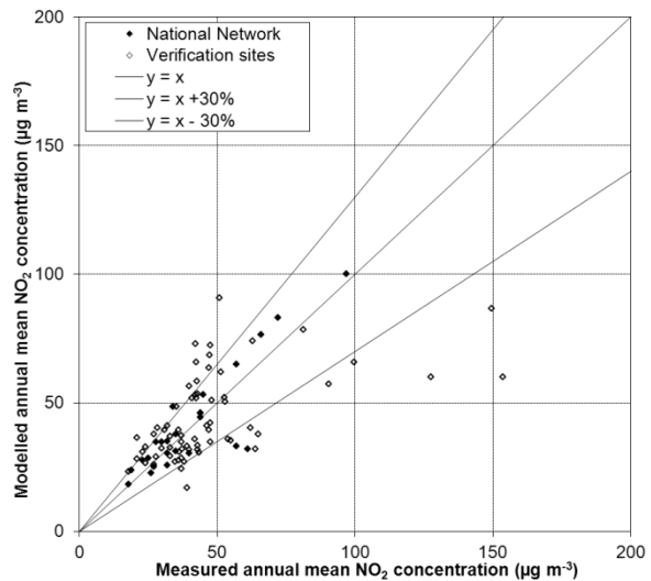
Figure 3.20 - Verification of roadside annual mean NO 2 model 2011
