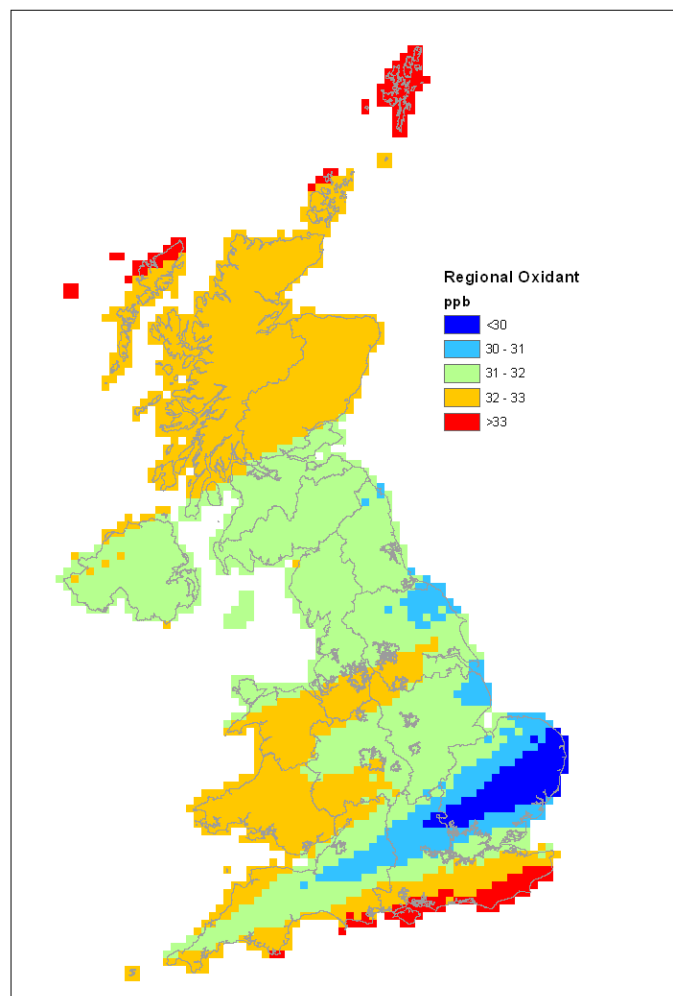
Figure 3.10 - Regional oxidant [OX]_B for 2011 (ppb)
