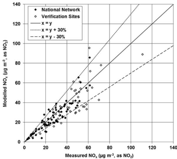
Figure 3-20 - Verification of roadside annual mean NO x model 2017
