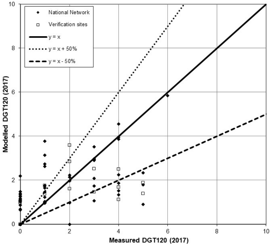
Figure 9-6 - Verification of background number of days > 120 µg m -3 model 2017
