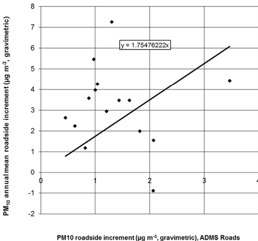
Figure 5-9 - Calibration of PM 10 PCM-RKM model 2017 (µg m -3 , gravimetric)
