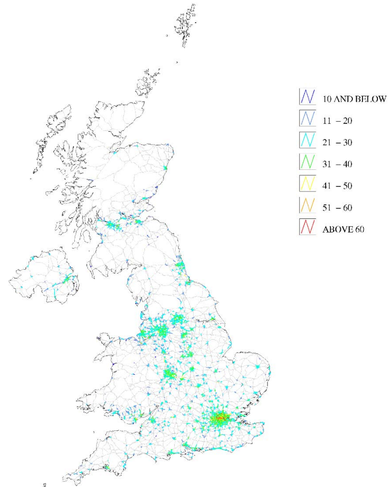
Figure 3-2 - Urban major roads, annual mean roadside NO 2 concentration, 2017 ( \mu\text{g m}^{-3} )
