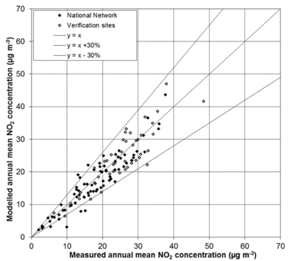
Figure 3-21 - Verification of roadside annual mean NO 2 model 2017
