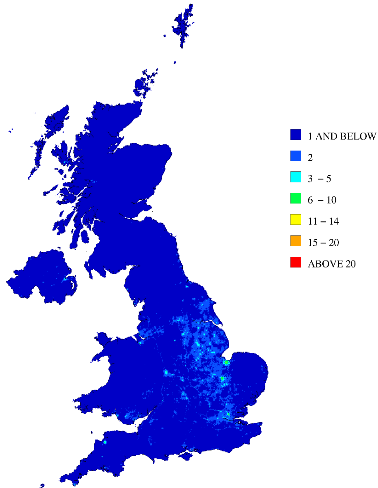
Figure 10-4 - Annual mean background Ni concentration, 2017 (ng m -3 )
