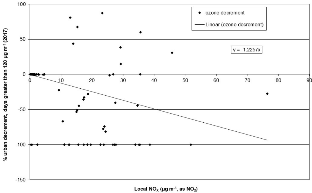
Figure 9-5 - Days greater than 120 µg m -3 percentage decrement in ozone concentrations, 2015-2017
