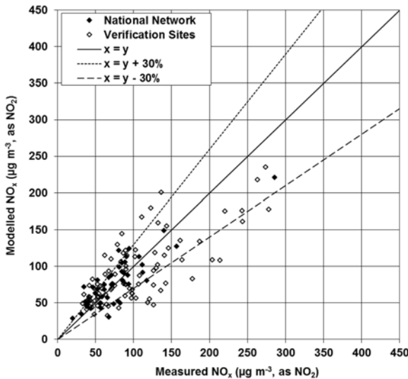
Figure 3-20 - Verification of roadside annual mean NO x model 2017
