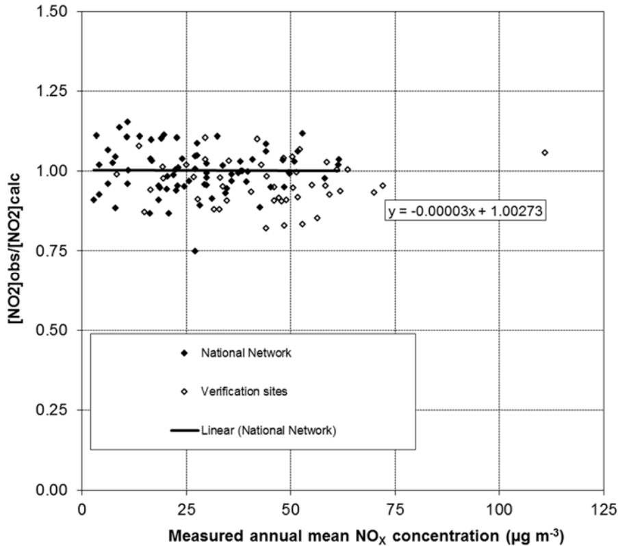
Figure 3-13 - Verification of background relationship at background locations in 2017 a) Uncalibrated b) Calibrated
