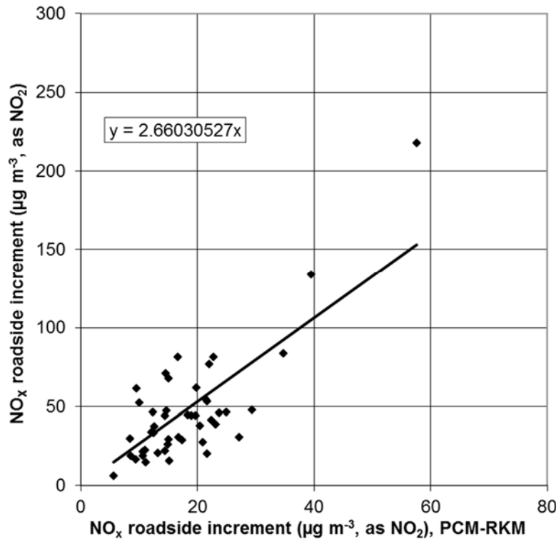
Figure 3-9 - Calibration of NO x PCM RKM model, 2017 (µg m -3 , as NO 2 )
