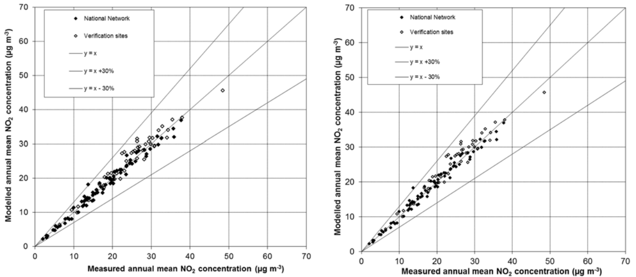
Figure 3-13 - Verification of background relationship at background locations in 2017 a) Uncalibrated b) Calibrated
