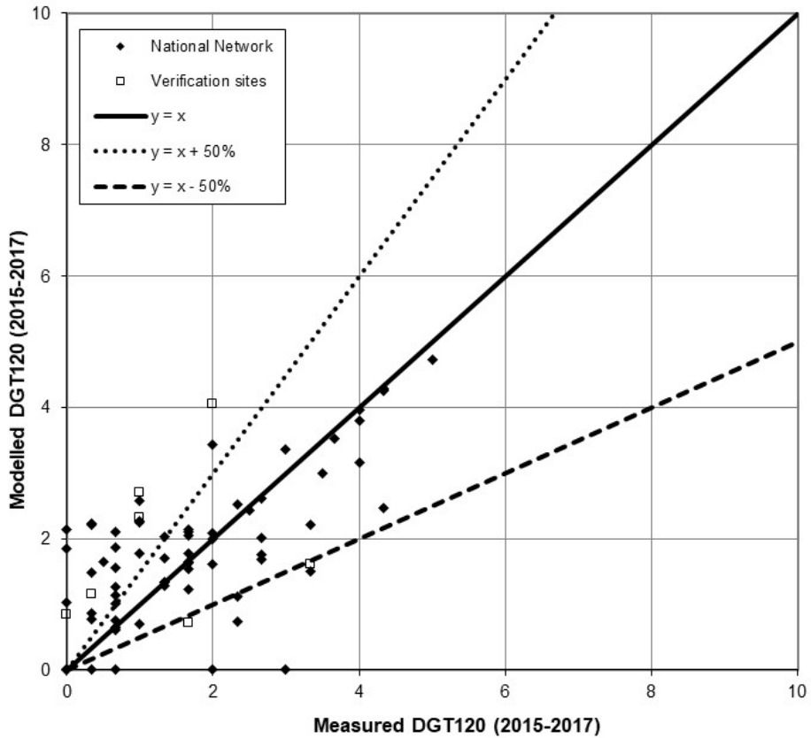
Figure 9-7 - Verification of background number of days > 120 µg m -3 model 2015-2017
