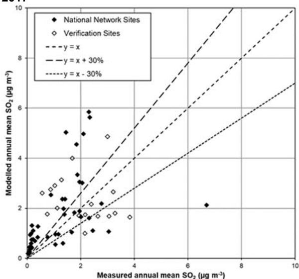
Figure 4-12 - Verification of annual mean SO 2 model, 2017
