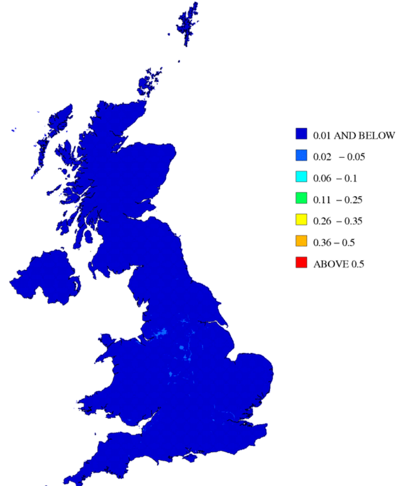
Figure 10-5 - Annual mean background Pb concentration, 2017 (µg m -3 )
