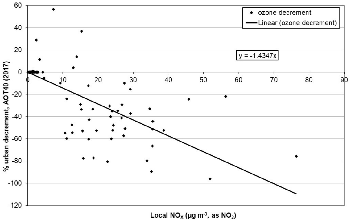
Figure 9-11 - AOT40 percentage decrement in ozone concentrations, 2013-2017
