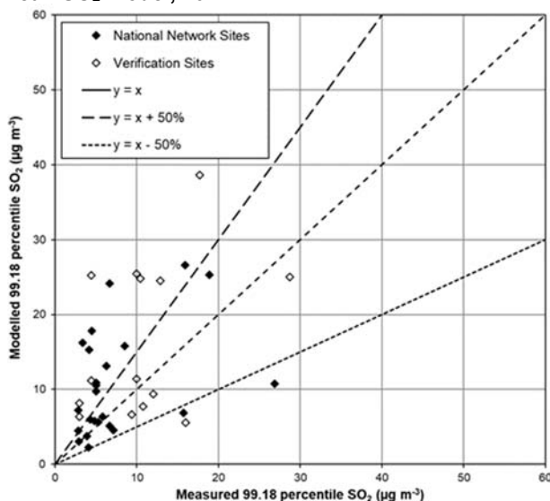
Figure 4-14 -Verification of 99.18 percentile of 24-hour mean SO 2 model, 2017
