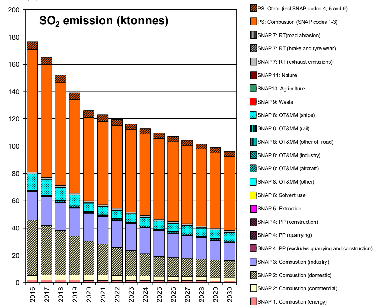
Figure 4-6 - Total UK SO 2 emissions for 2016 and emissions projections up to 2030 by SNAP code from NAEI 2016
