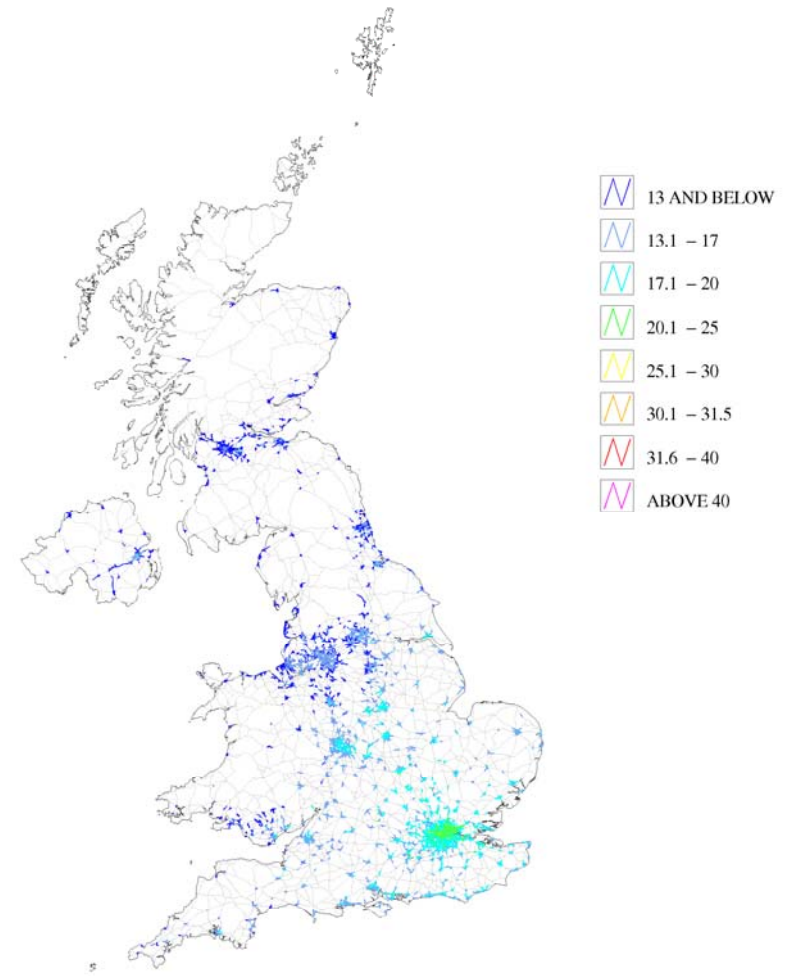
Figure 5-2 - Urban major roads, annual mean roadside PM 10 concentration, 2017 ( \mu\text{g m}^{-3} , gravimetric)
