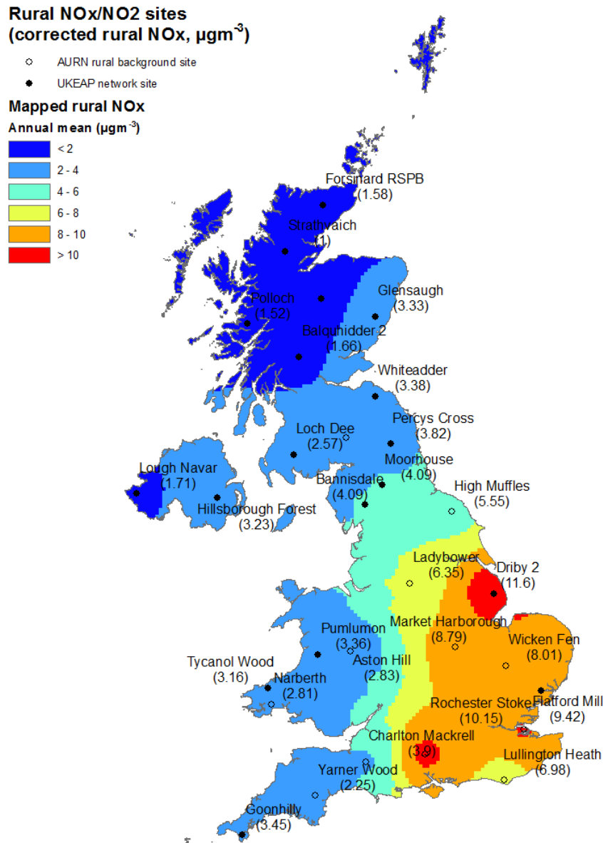
Figure 3-7 - Rural background NO x concentrations map with monitoring sites used in the interpolation (annual mean NO x concentrations for 2017 (μg m -3 , as NO 2 ) are shown below the site name)
