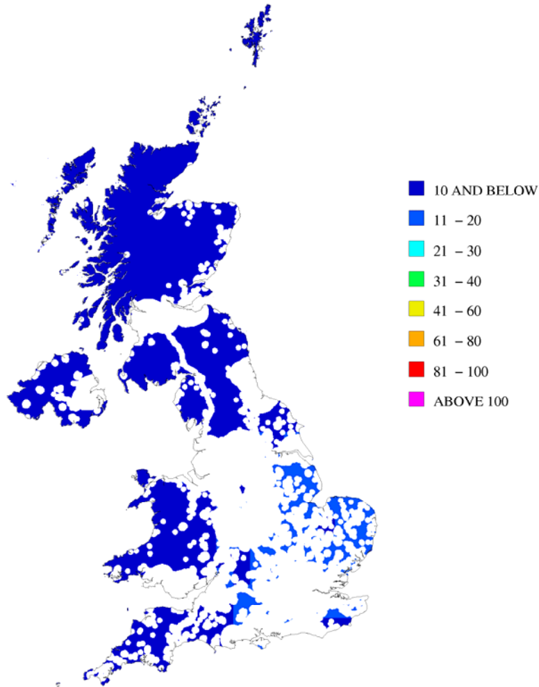
Figure 3-3 - Annual mean map of NO x concentrations for comparison with the NO x vegetation critical level, 2017 (µg m -3 , as NO 2 )
