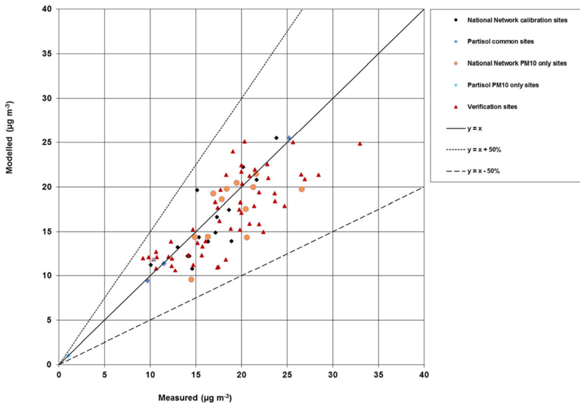
Figure 5-11 - Verification of roadside annual mean PM 10 model 2017
