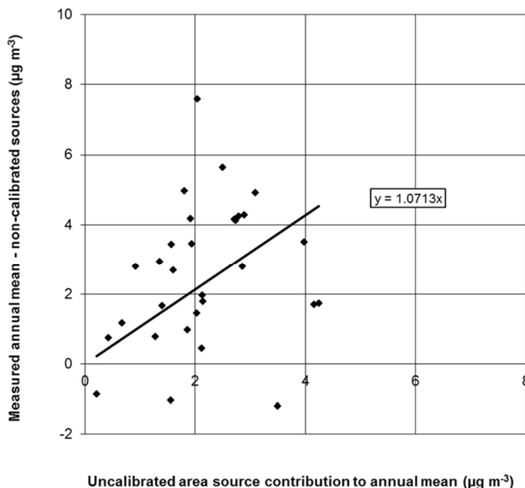
Figure 5-8 - Calibration of PM 10 area source model 2017 (µg m -3 , gravimetric)
