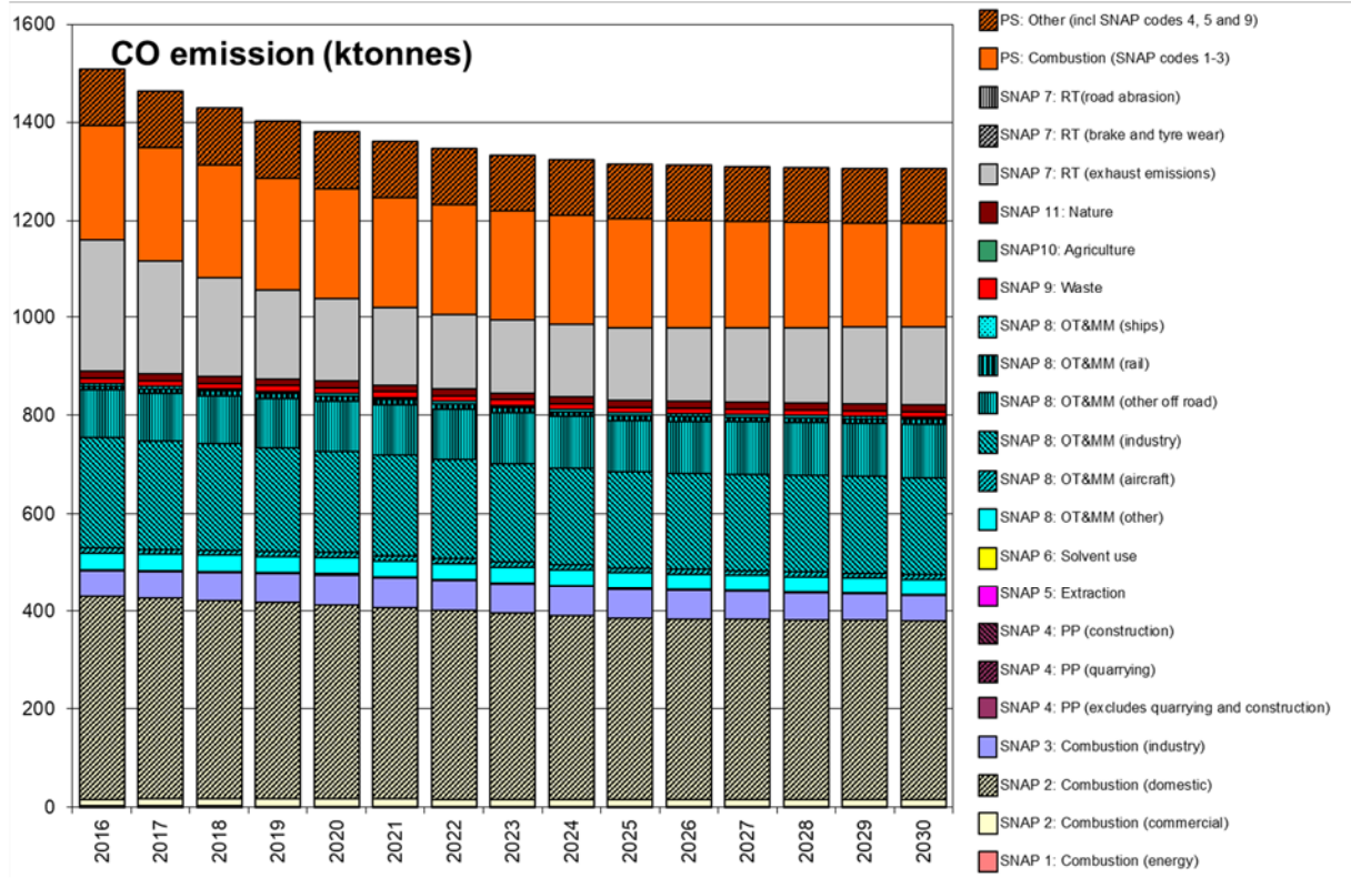
Figure 8-1 - Total UK CO emissions for 2016 and emissions projections up to 2030 by SNAP code from NAEI 2016
