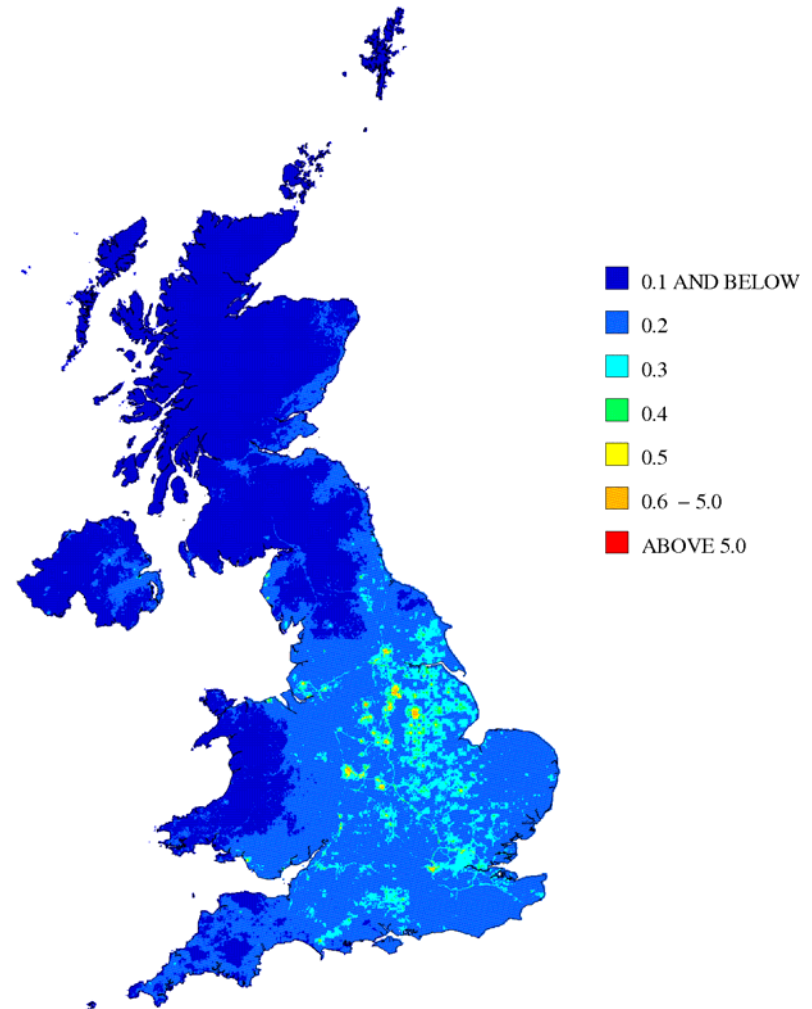
Figure 10-3 - Annual mean background Cadmium (Cd) concentration, 2017 (ng m -3 )
