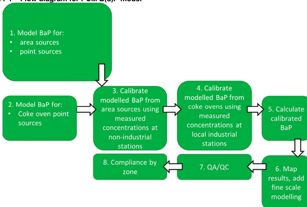
Figure 11-1 – Flow diagram for PCM B(a)P model
