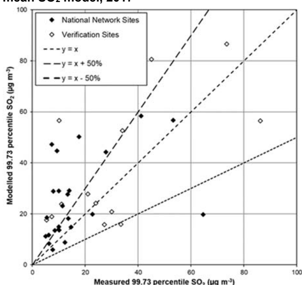
Figure 4-13 - Verification of 99.73 percentile of 1-hour mean SO 2 model, 2017
