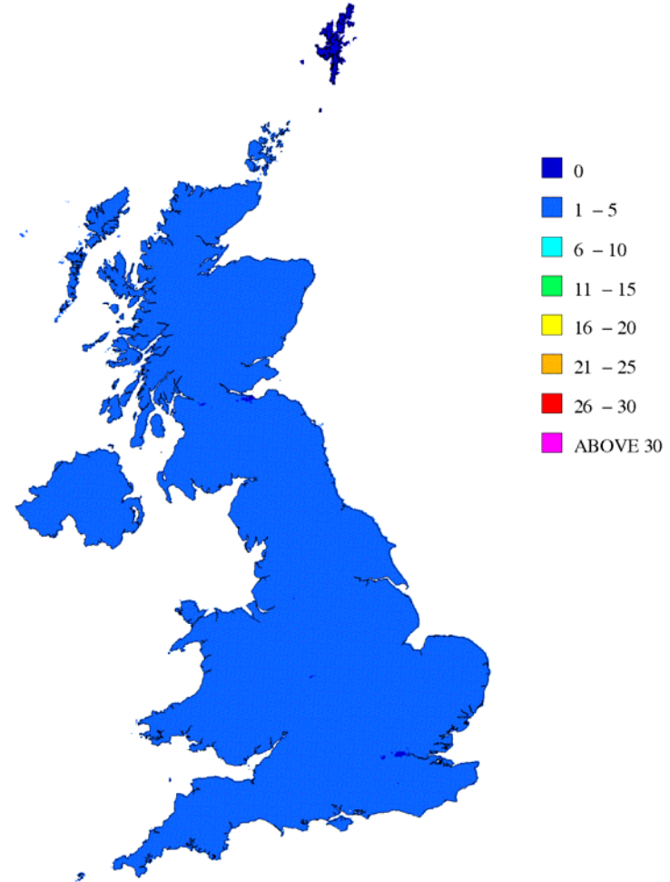
Figure 9-3 - Estimated average number of days with an 8-hour mean ozone concentration above 120 \mu\text{g m}^{-3} , 2015 to 2017
