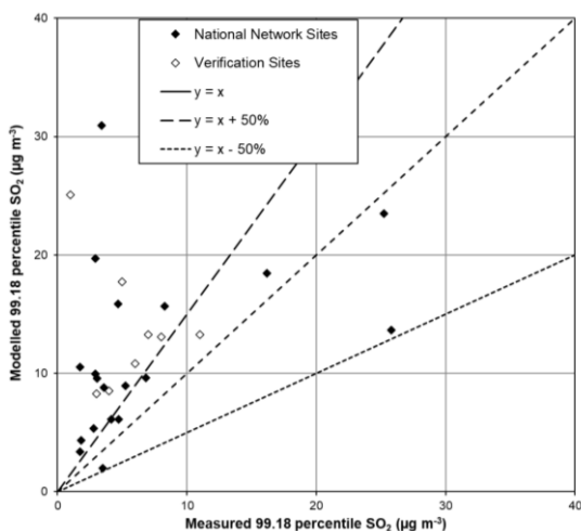
Figure 5.14 -Verification of 99.18 percentile of 24-hour mean SO 2 model, 2020
