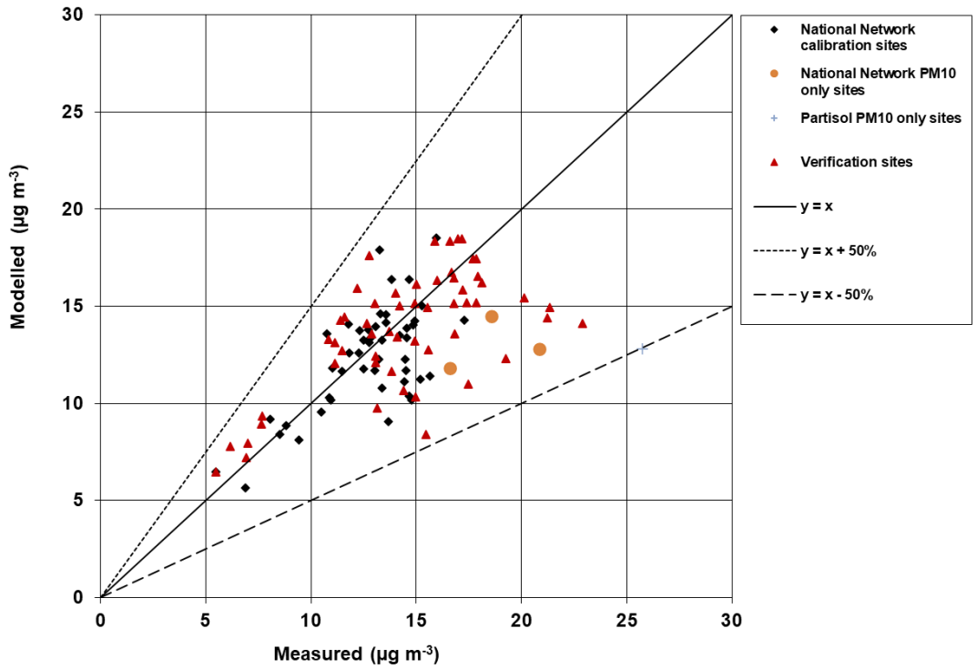
Figure 6.11 - Verification of roadside annual mean PM 10 model 2020
