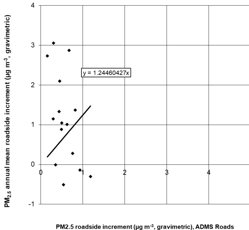
Figure 7.6 - Calibration of PM_{2.5} roadside increment model 2020 ( \mu g m^{-3} , gravimetric)
