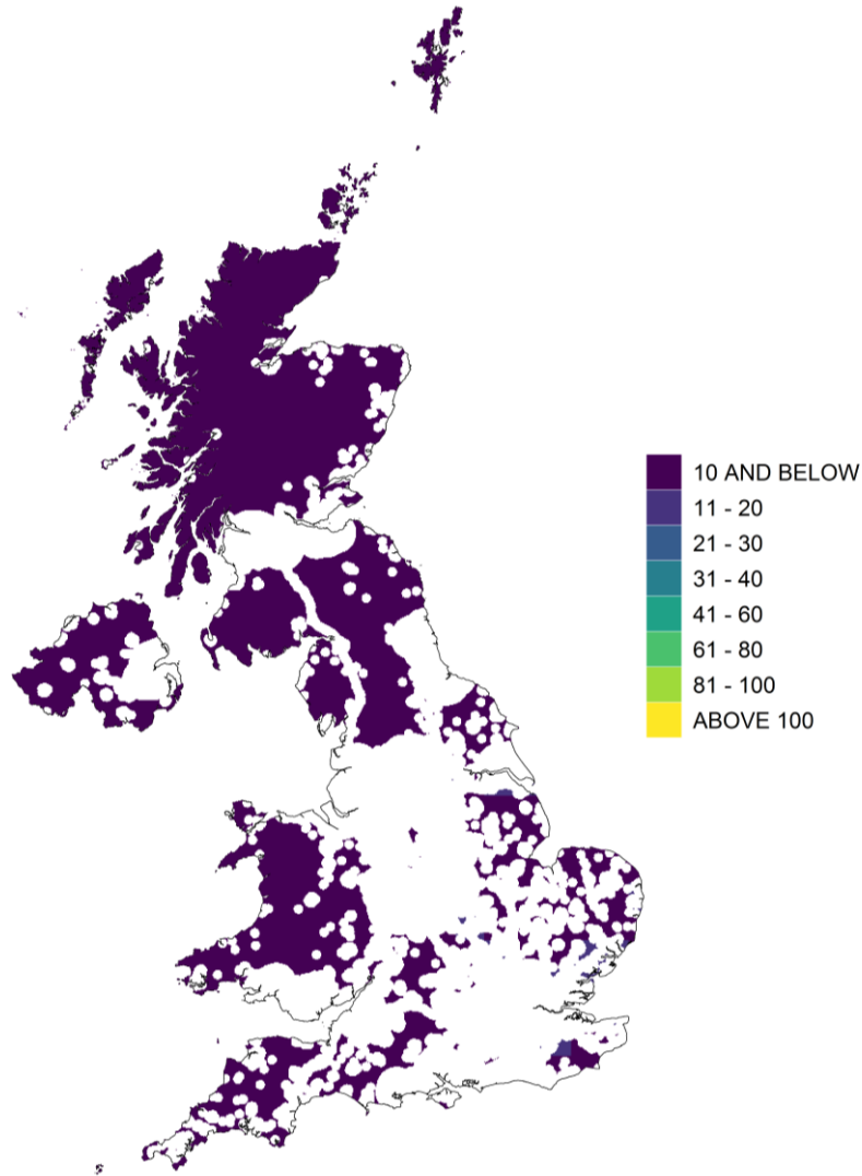
Figure 4.3 - Annual mean map of NO x concentrations for comparison with the NO x vegetation critical level, 20120 (µg m -3 , as NO 2 )
