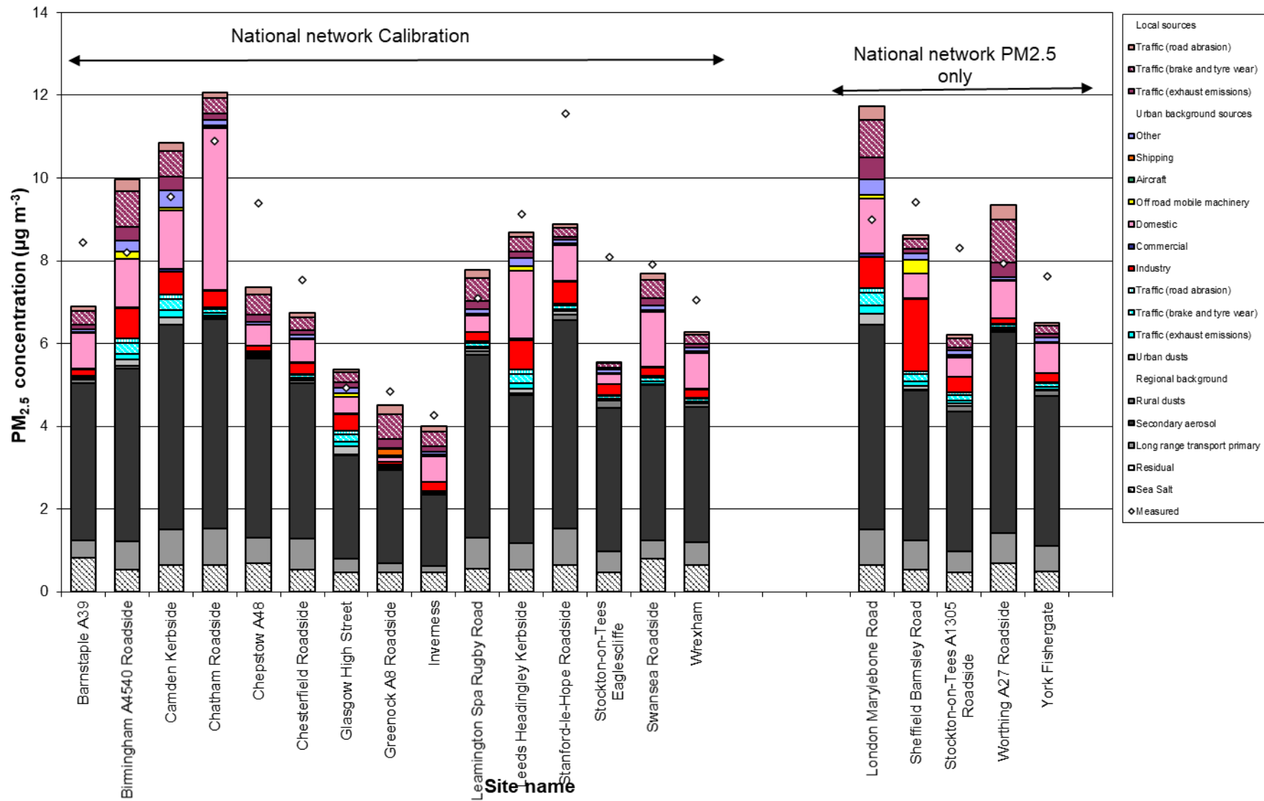
Figure 7.10 - Annual mean PM 2.5 source apportionment at roadside national network monitoring sites 2020
