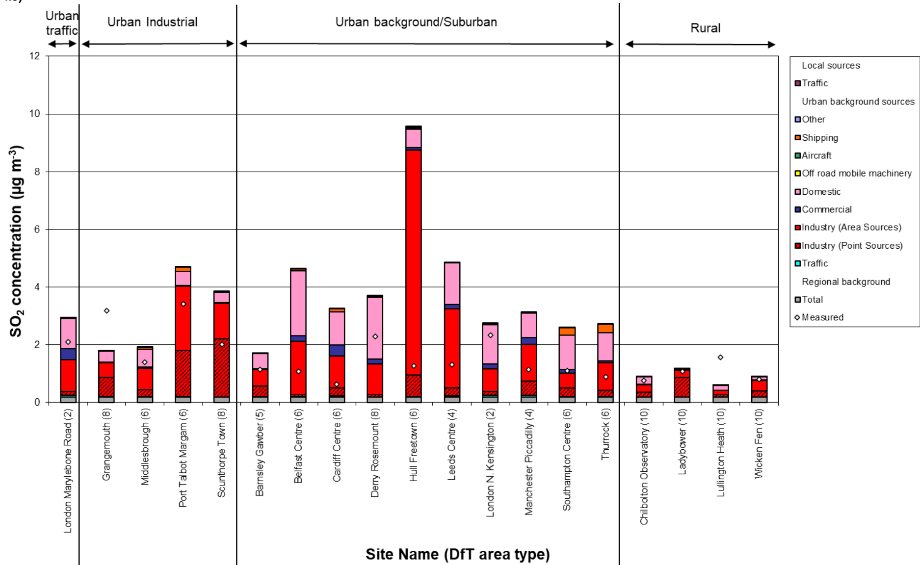
Figure 5.15 - Annual mean SO 2 source apportionment at AURN monitoring sites in 2020 (the area type of each site is shown in parenthesis after its name – see Table 4.5)
