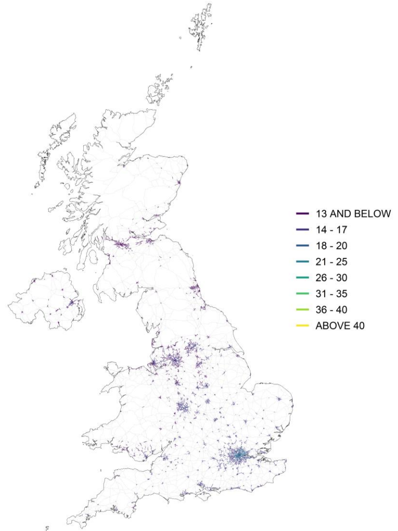
Figure 6.2 - Urban major roads, annual mean roadside PM 10 concentration, 2020 ( \mu\text{g m}^{-3} , gravimetric)
