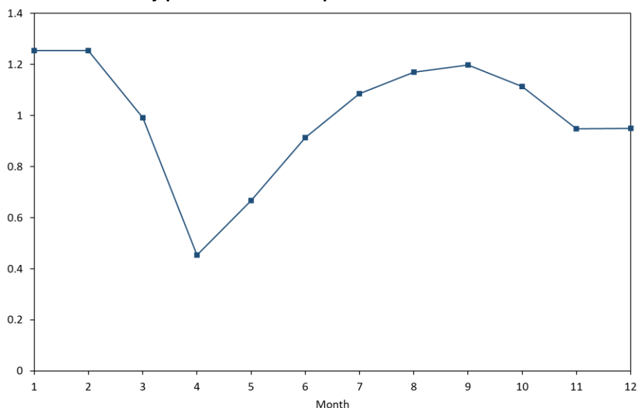
Figure 3.1 - Normalised monthly profile of road transport emissions for 2020
