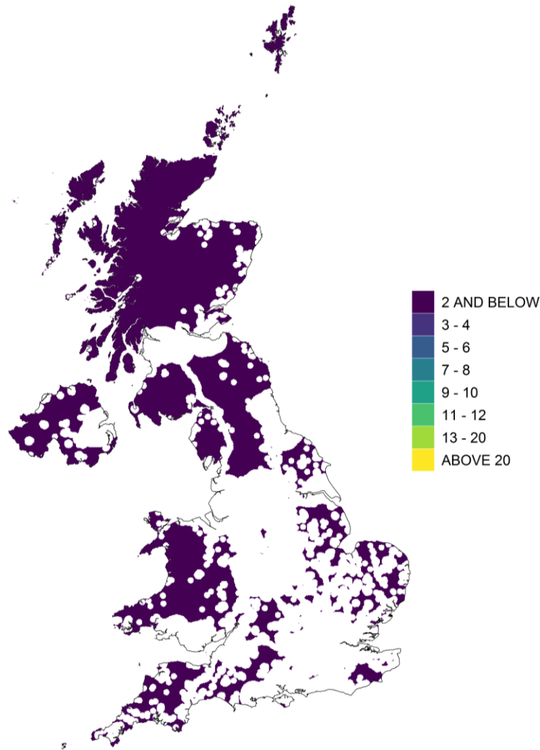
Figure 5.2 - Annual mean SO 2 concentration, 2020 (µg m -3 ) in vegetation areas
