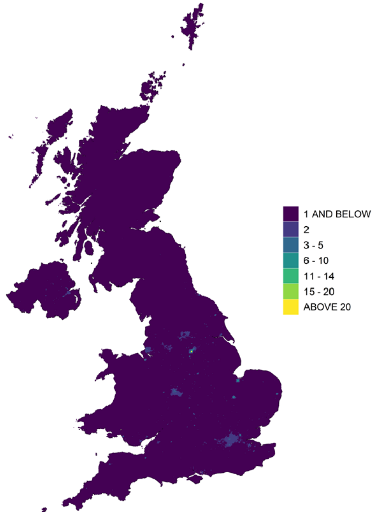
Figure 11.4 - Annual mean background Ni concentration, 2020 (ng m -3 )
