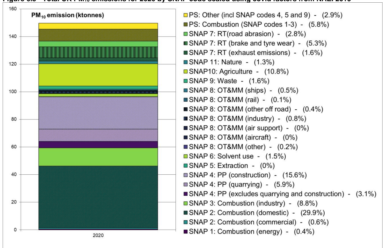
Figure 6.5 - Total UK PM 10 emissions for 2020 by SNAP code scaled using covid factors from NAEI 2019
