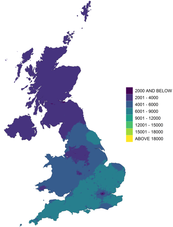
Figure 10.9 - Estimated AOT40 vegetation metric, averaged 2016-2020 ( \mu\text{g m}^{-3} hours)
