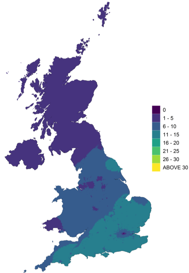
Figure 10.3 - Estimated average number of days with an 8-hour mean ozone concentration above 120 \mu\text{g m}^{-3} , 2018 to 2020
