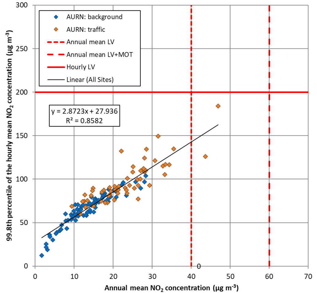
Figure 4.4 - Plot of annual mean against 99.8th percentile hourly NO 2 concentrations in 2020
