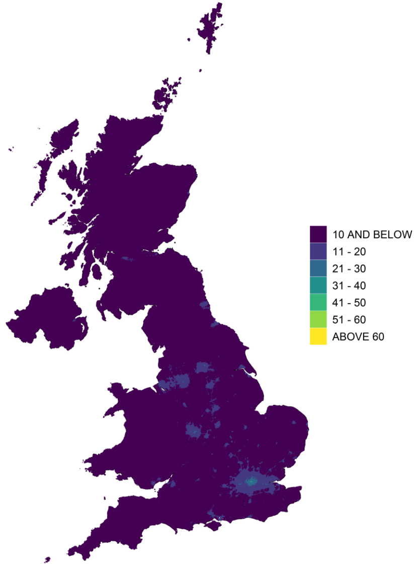
Figure 4.1 - Annual mean background NO 2 concentration, 2020 ( \mu\text{g m}^{-3} )
