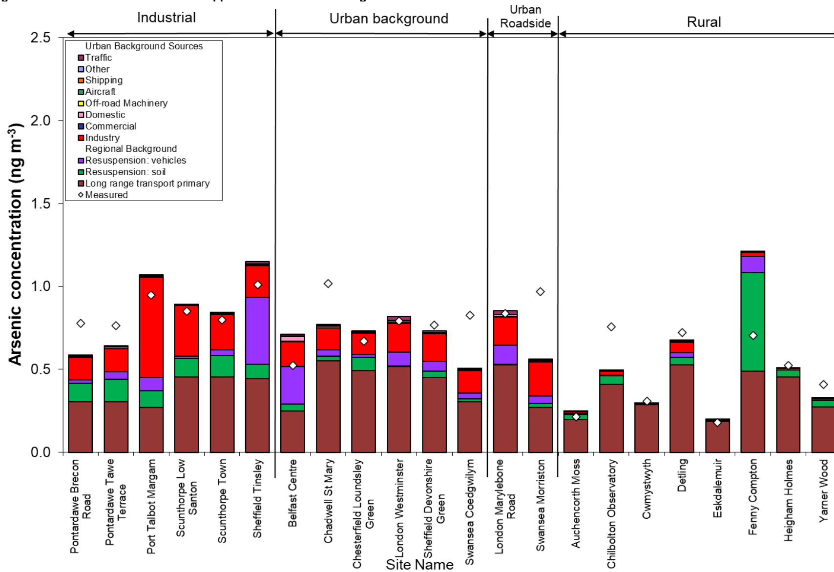
Figure 11.11 - Annual mean As source apportionment at monitoring sites in 2020.
