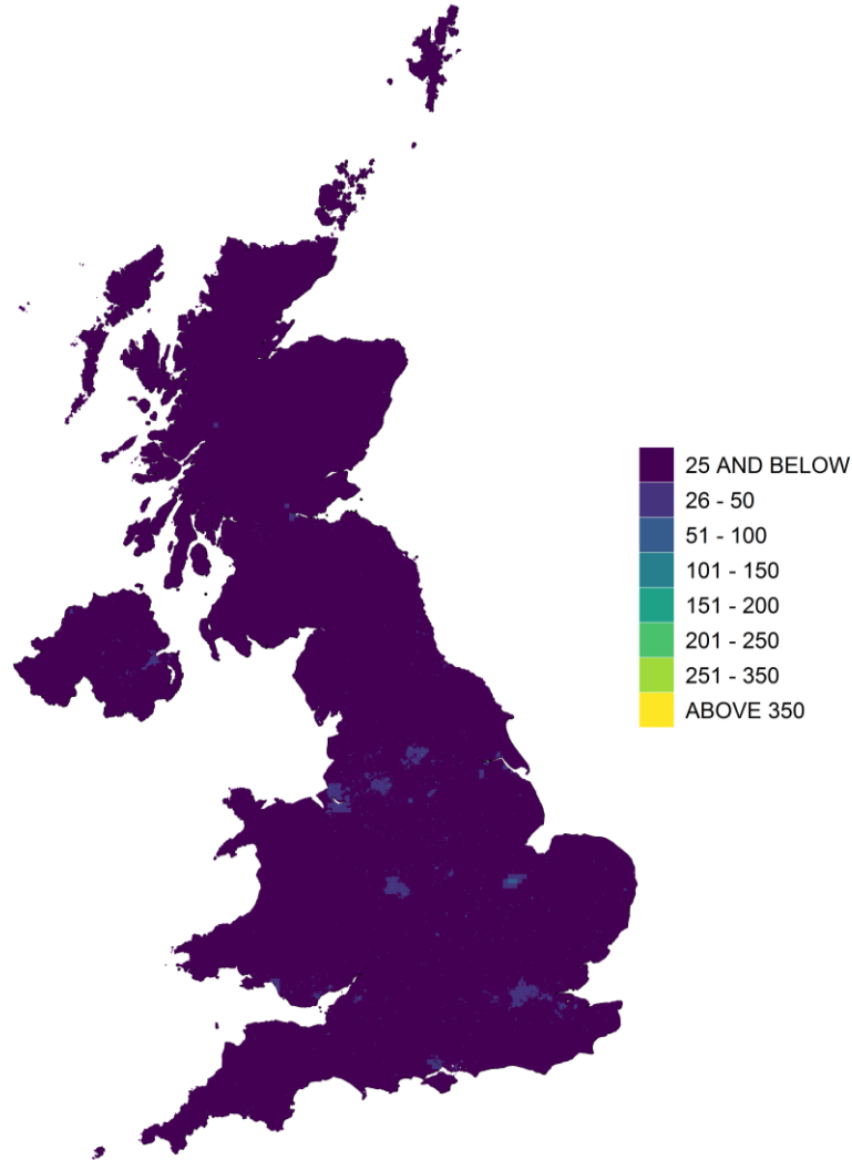
Figure 5.4 - 99.73 percentile of 1-hour mean SO 2 concentration, 2020 (µg m -3 )
