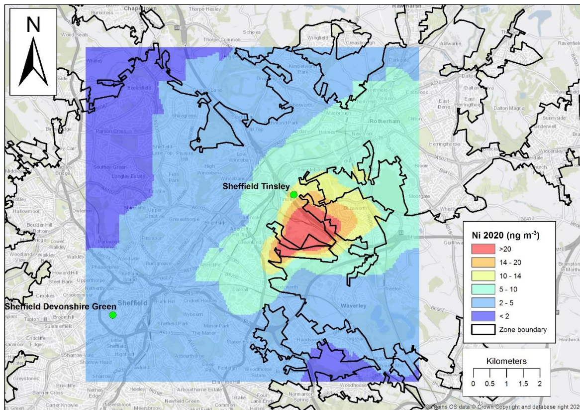
Figure 11.17 - Modelled annual mean Ni concentration resulting from the local industrial sources in Sheffield Tinsley in 2020.
