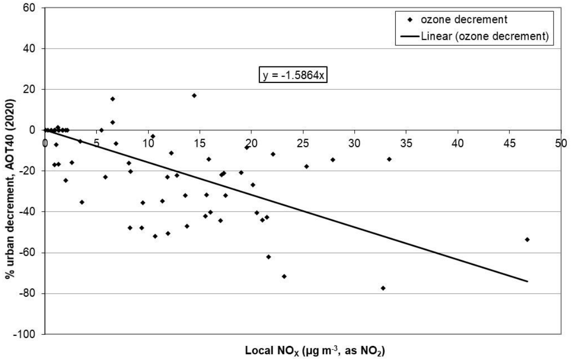
Figure 10.11 - AOT40 percentage decrement in ozone concentrations, 2016-2020
