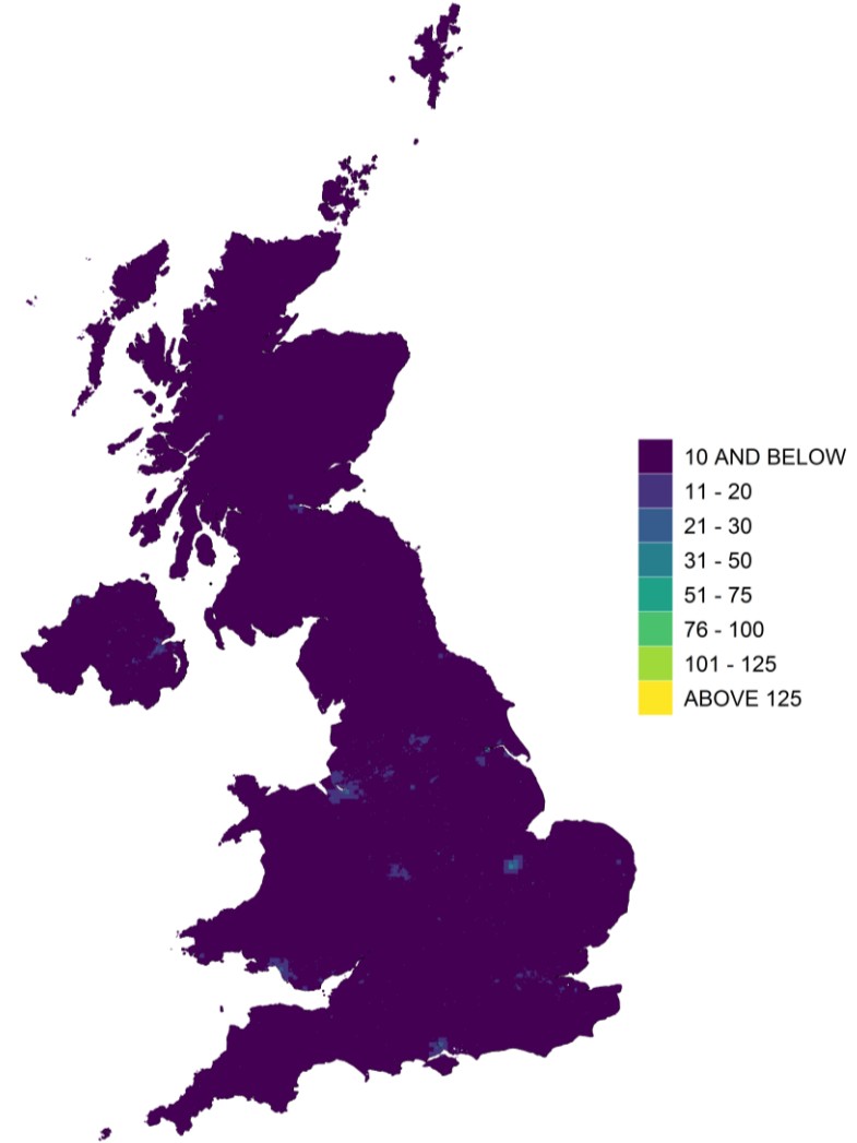
Figure 5.5 - 99.18 percentile of 24-hour mean SO 2 concentration, 2020 (µg m -3 )
