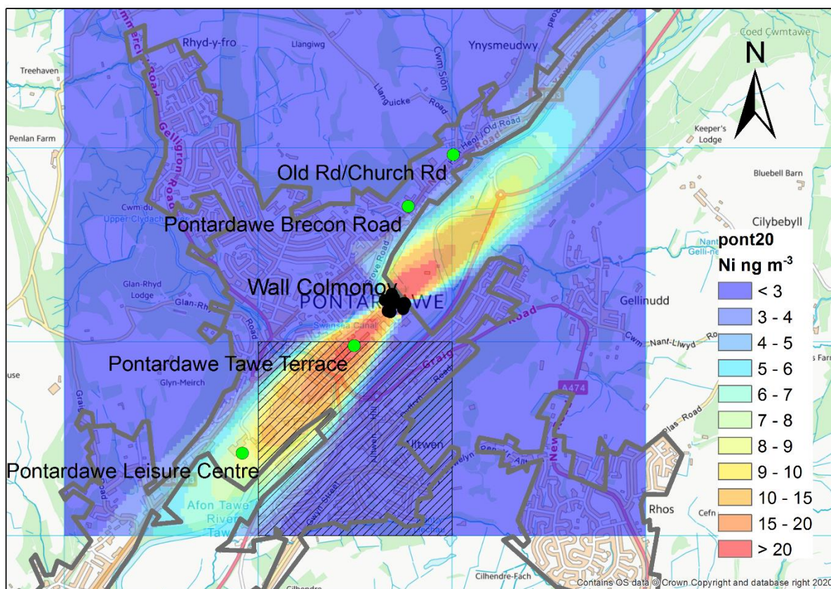
Figure 11.16 - Modelled annual mean Ni concentration resulting from the local industrial point source in Pontardawe in 2020.
