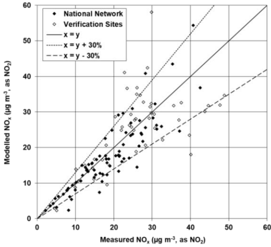
Figure 4.18 - Verification of roadside annual mean NO x model 2020
