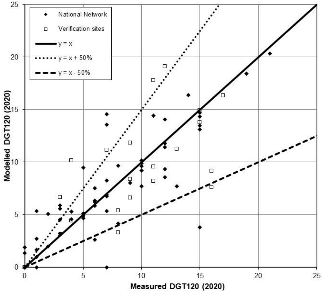
Figure 10.6 - Verification of background number of days > 120 µg m -3 model 2020
