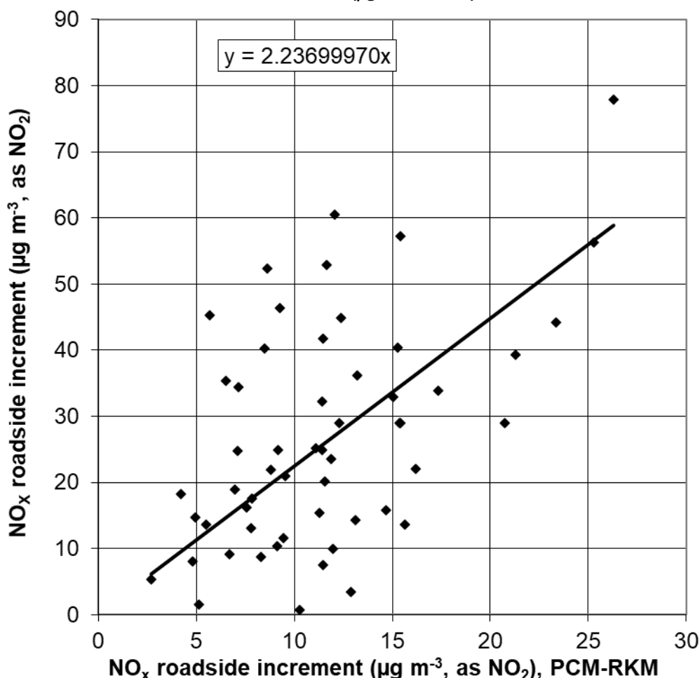
Figure 4.9 - Calibration of \text{NO}_x PCM RKM model, 2020 ( \mu\text{g m}^{-3} , as \text{NO}_2 )
