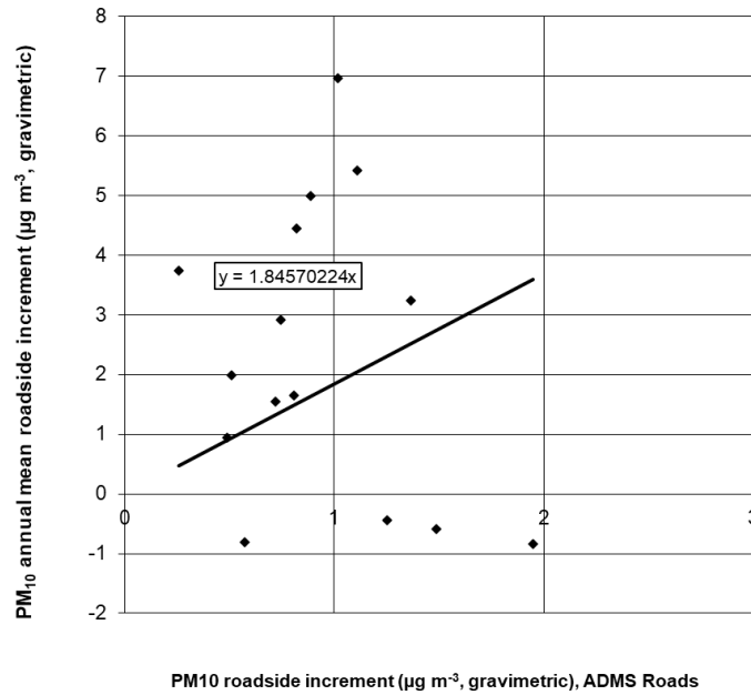
Figure 6.9 - Calibration of PM 10 PCM-RKM model 2020 (µg m -3 , gravimetric)
