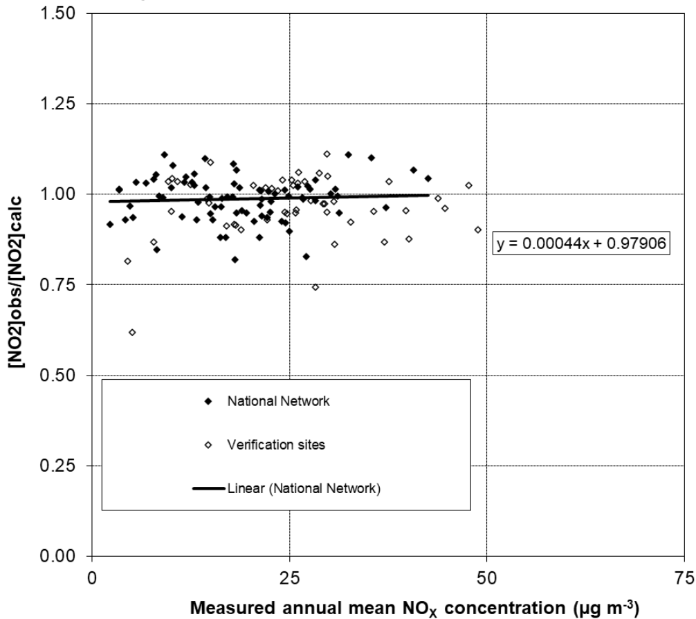
Figure 4.13 - Verification of background relationship at background locations in 2020
