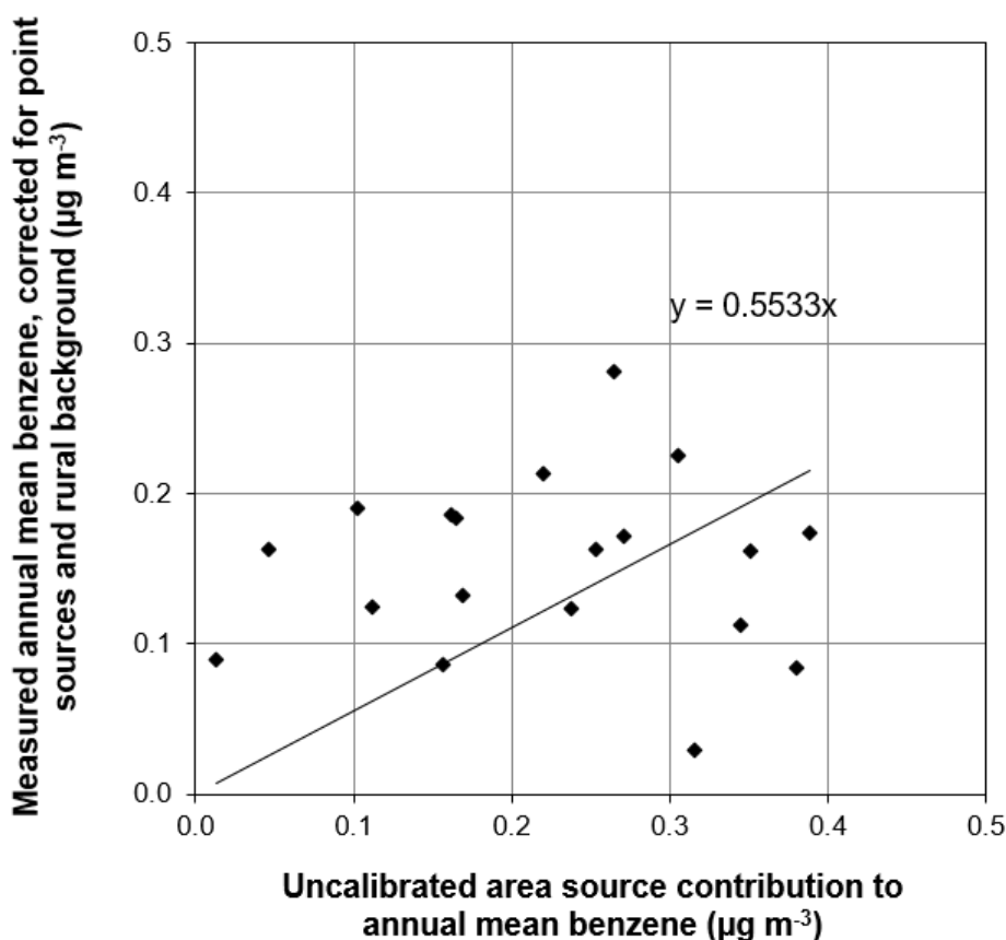
Figure 8.5 - Calibration of area source benzene model, 2020 ( \mu\text{g m}^{-3} )
