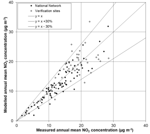
Figure 4.19 - Verification of roadside annual mean NO 2 model 2020
