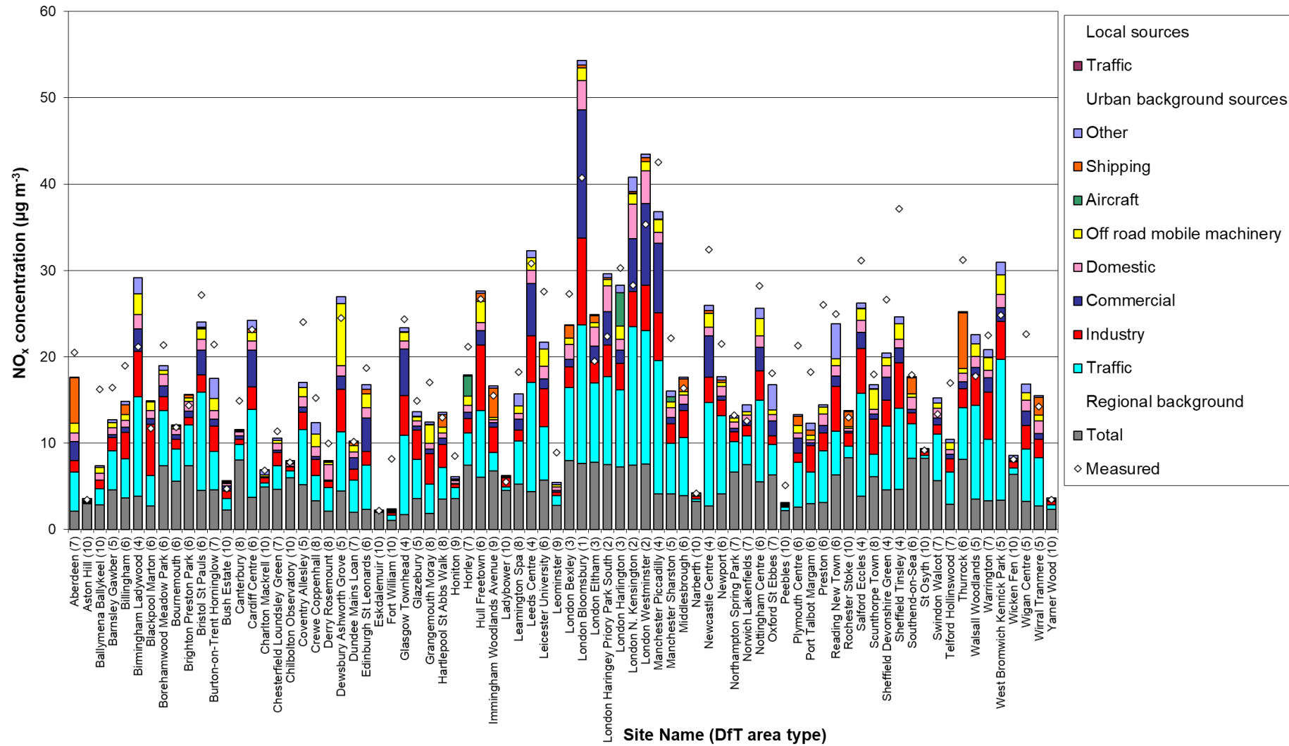
Figure 4.20 - Annual mean NO x source apportionment at background AURN monitoring sites in 2020 (area type of each site is shown in parenthesis after its name – see Table 4.5)
