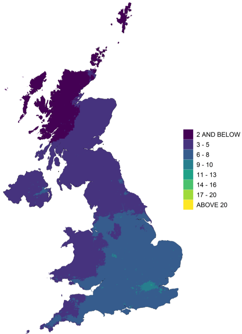
Figure 7.1 - Annual mean background PM 2.5 concentration, 2020 ( \mu\text{g m}^{-3} , gravimetric)
