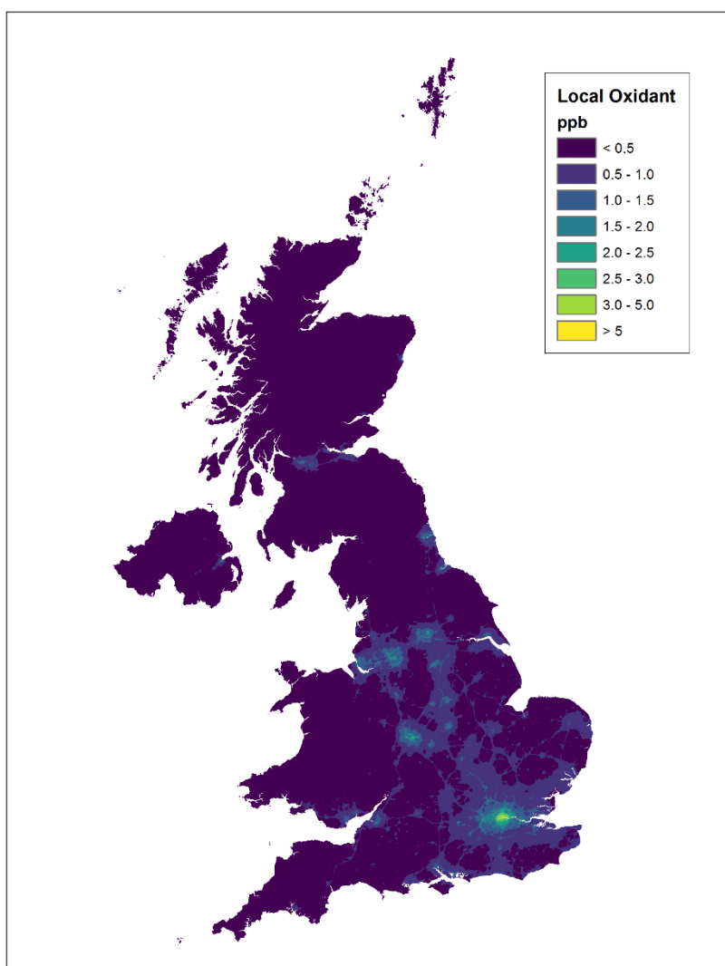
Figure 4.11 - Background local oxidant map for 2020 (ppb)
