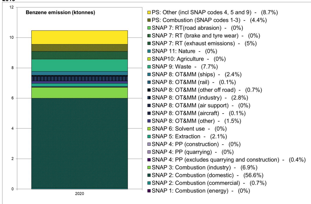
Figure 8.4 - Total UK benzene emissions for 2020 by SNAP code scaled using Covid factors from NAEI 2019
