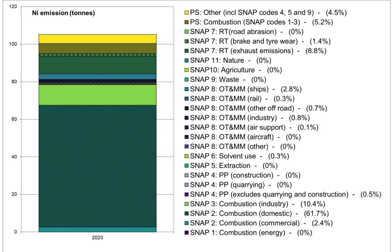
Figure 11.8 - Total UK Ni emissions for 2020 by SNAP code scaled using Covid factors from NAEI 2019
