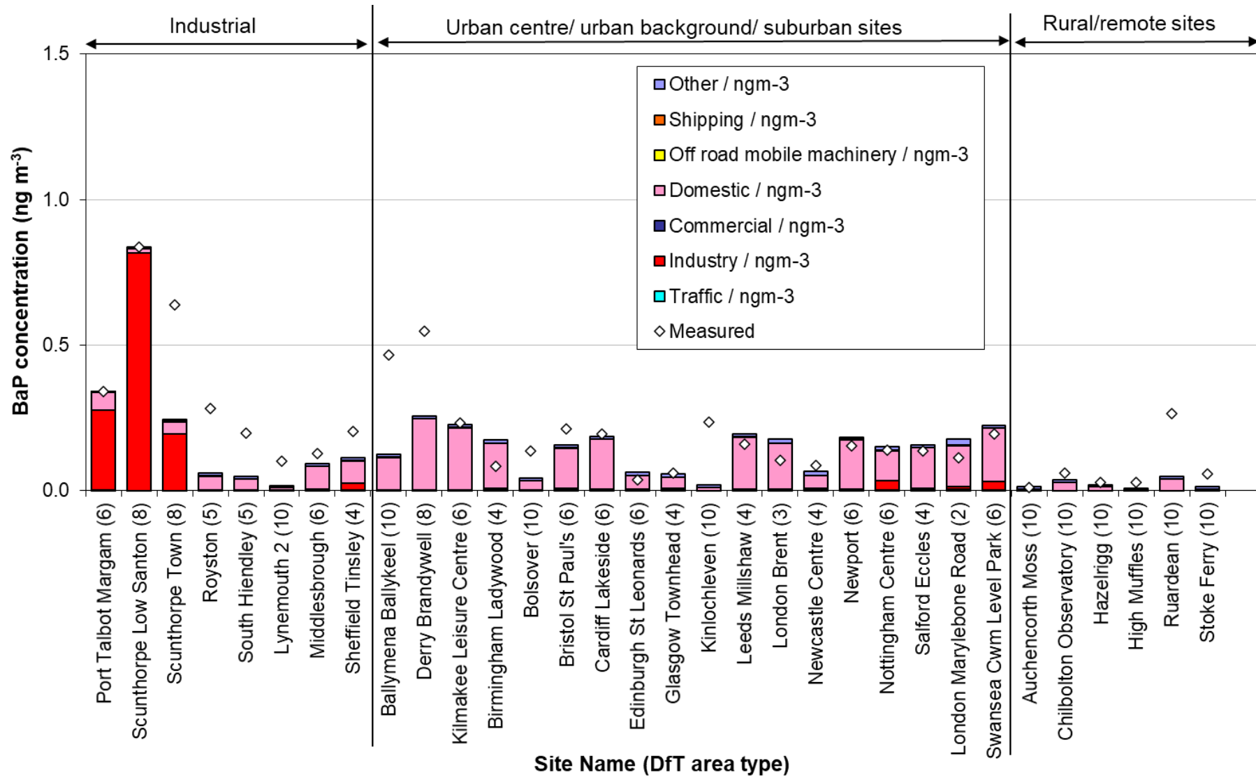
Figure 12.6 - Annual mean B(a)P source apportionment at background national network monitoring stations in 2020 (the area type of each station is shown in parenthesis after its name)
