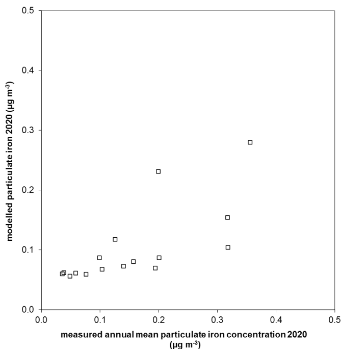
Figure 6.7 - Comparison of modelled and measured annual mean elemental Fe concentrations 2020 ( \mu\text{g m}^{-3} )
