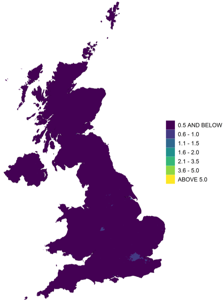
Figure 8.2 - Annual mean background benzene concentration, 2020 ( \mu\text{g m}^{-3} )
