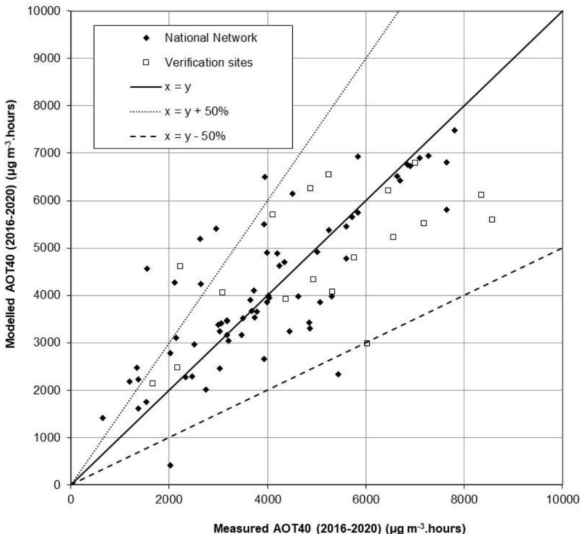
Figure 10.13 - Verification of background AOT40 vegetation model, 2016-2020
