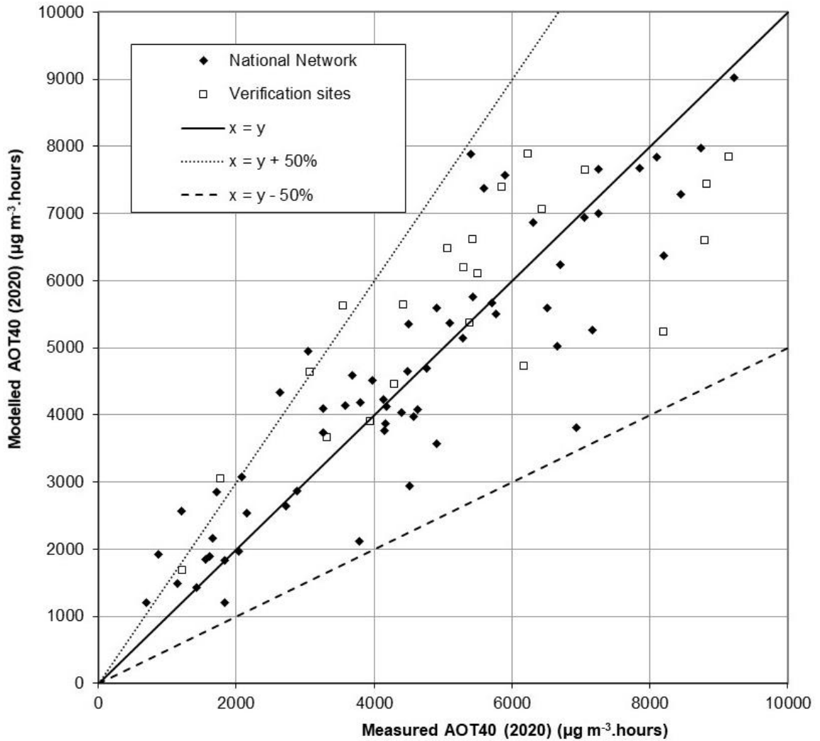
Figure 10.12 - Verification of background AOT40 vegetation model, 2020
