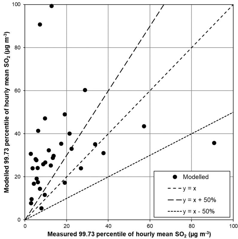
Figure 5.8 - Comparison plot for 2020 99.73 percentile of 1-hour mean SO 2 concentrations
