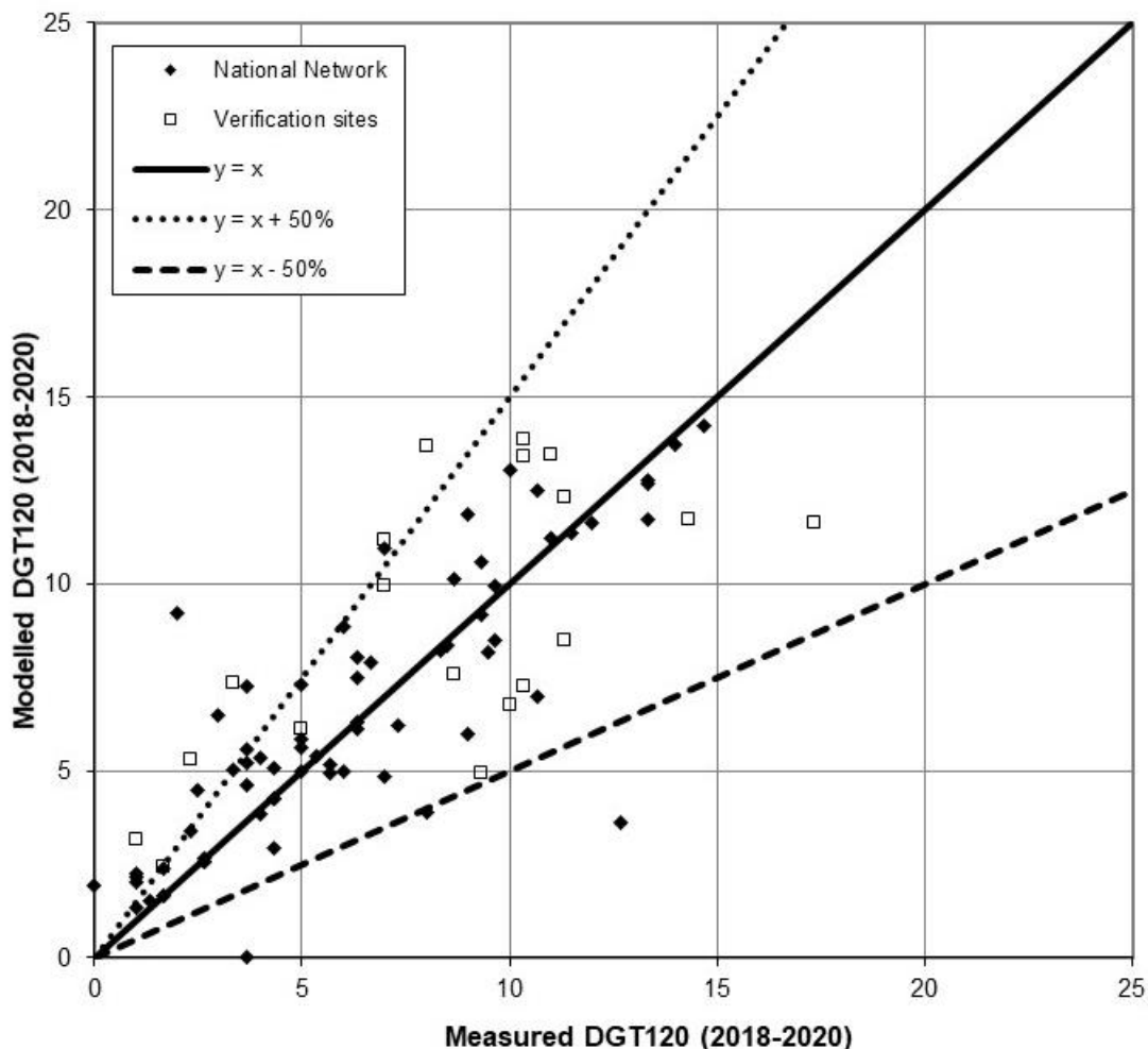
Figure 10.7 - Verification of background number of days > 120 µg m -3 model 2018-2020
