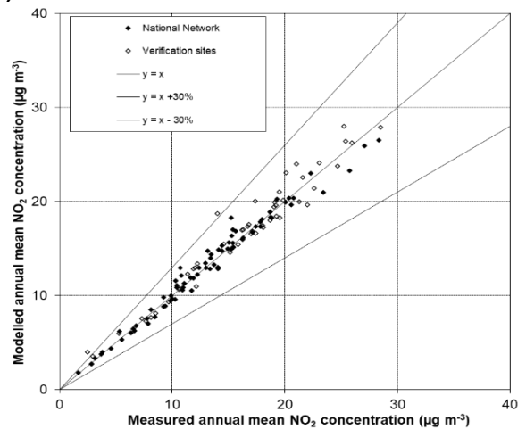
Figure 4.13 - Verification of background relationship at background locations in 2020
