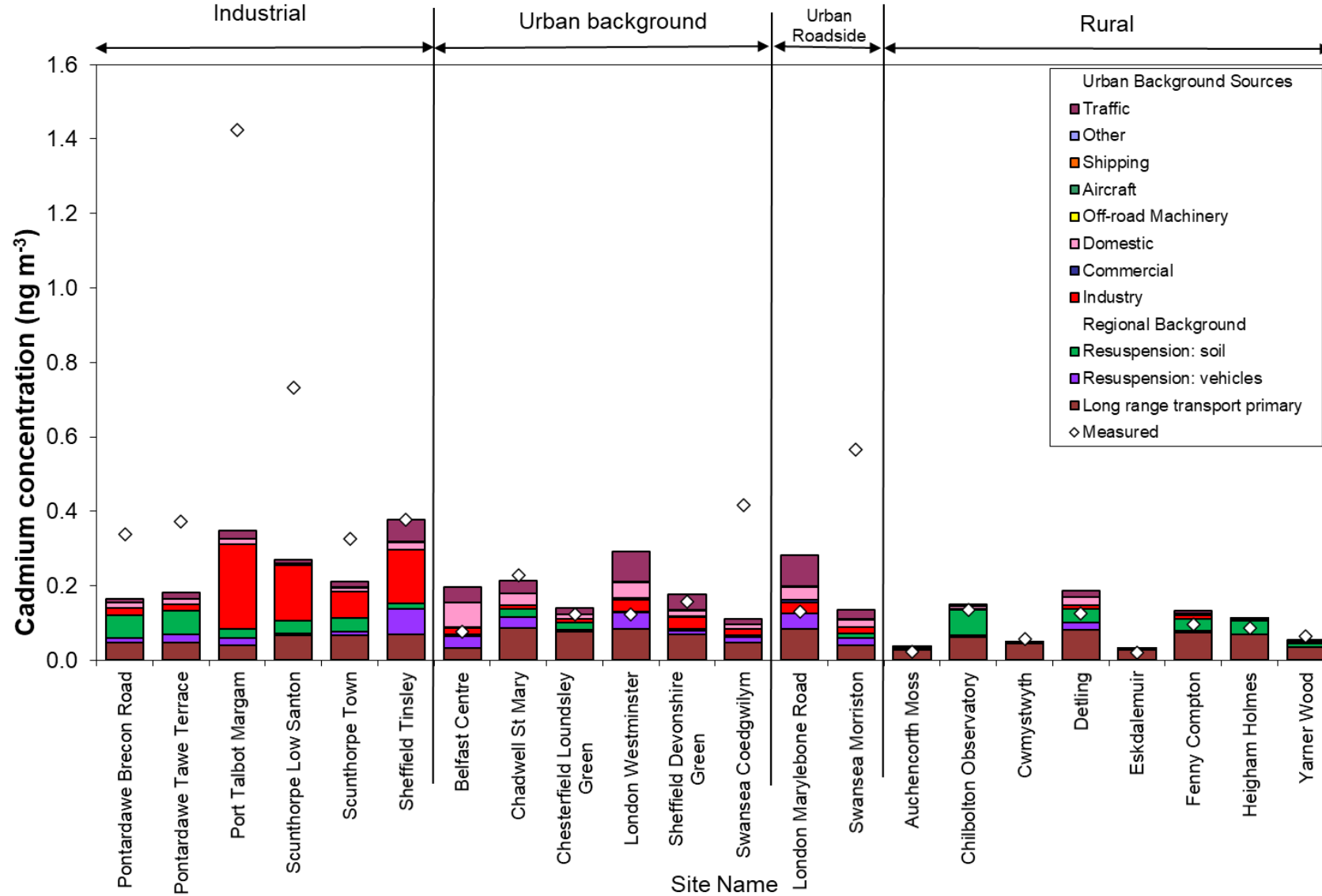
Figure 11.13 - Annual mean Cd source apportionment at monitoring sites in 2020.
