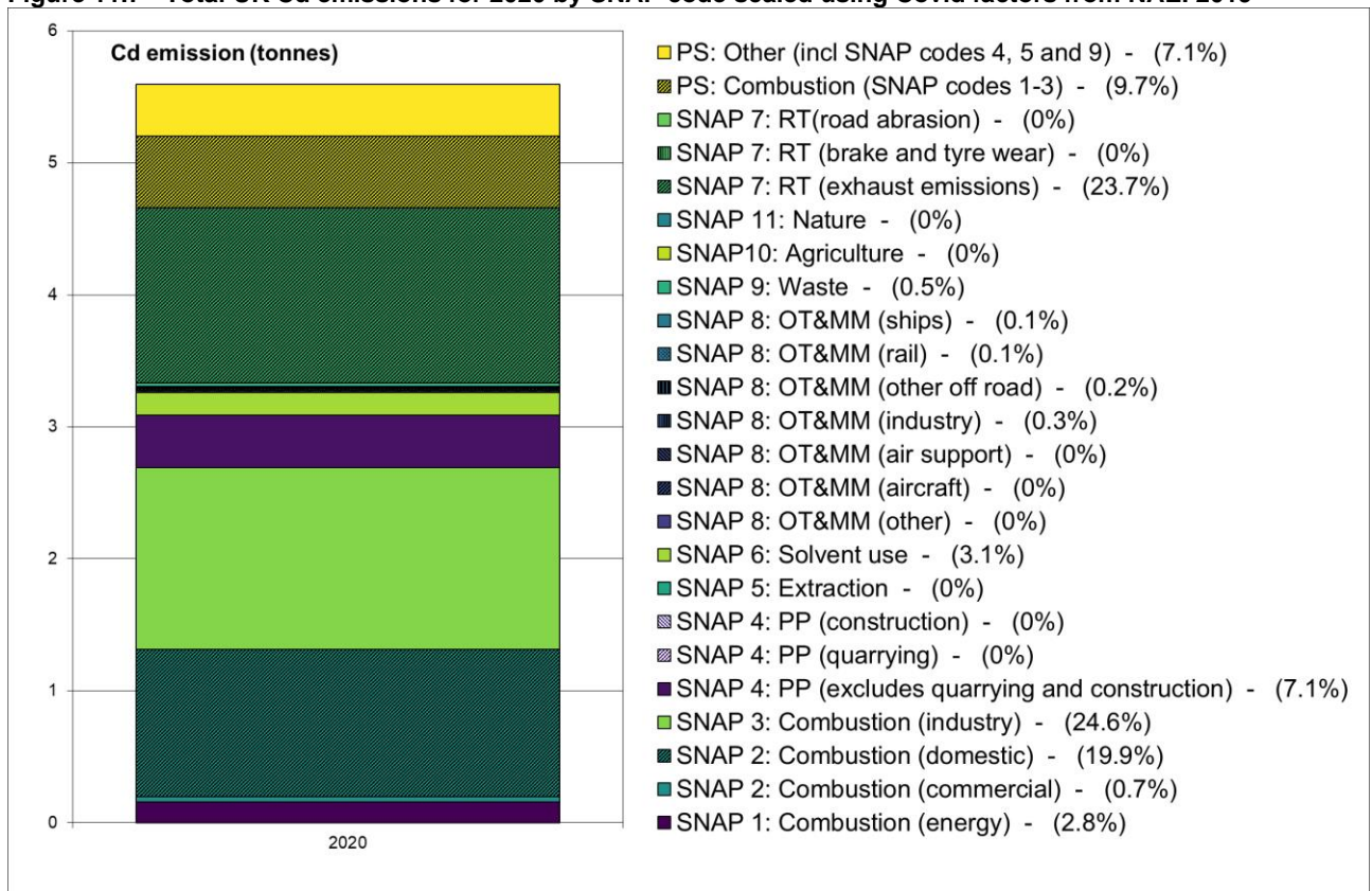
Figure 11.7 - Total UK Cd emissions for 2020 by SNAP code scaled using Covid factors from NAEI 2019
