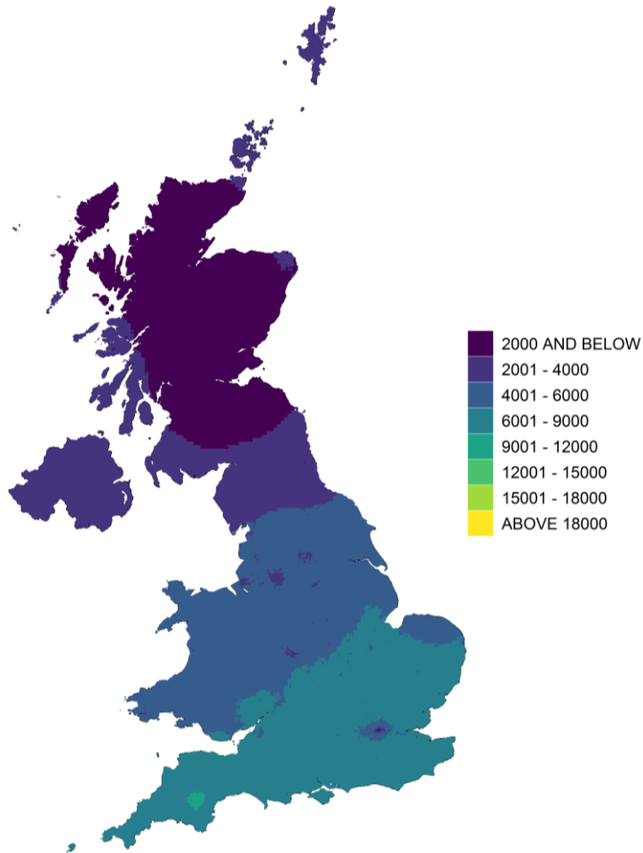
Figure 10.8 - Estimated AOT40 vegetation metric, 2020 ( \mu\text{g m}^{-3} hours)
