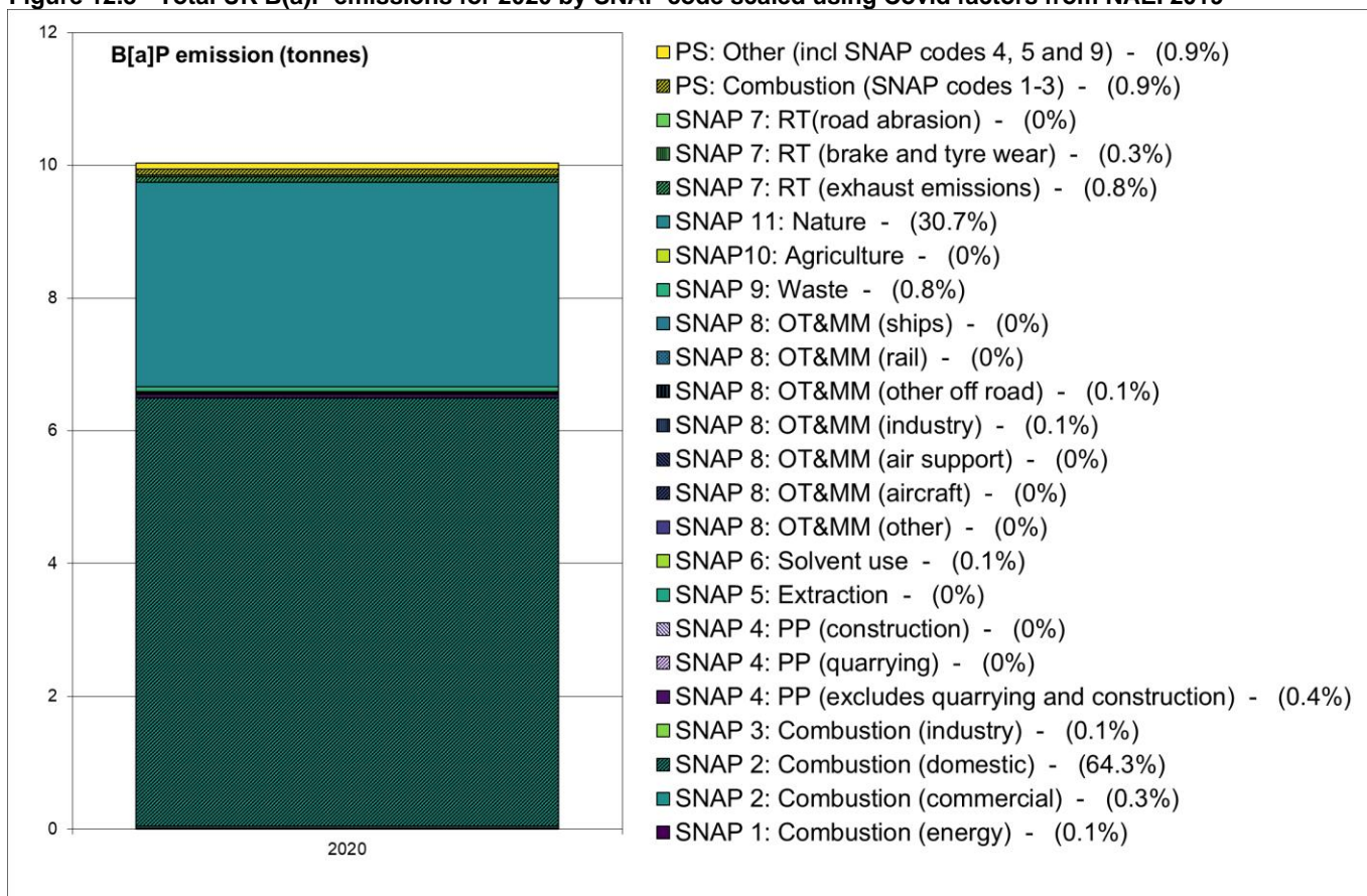
Figure 12.3 - Total UK B(a)P emissions for 2020 by SNAP code scaled using Covid factors from NAEI 2019
