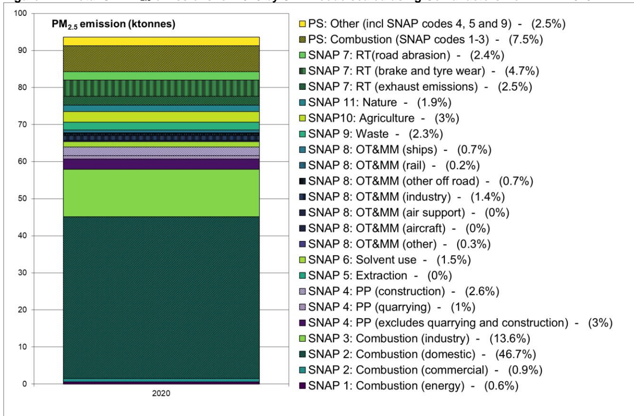
Figure 7.4 - Total UK PM 2.5 emissions for 2020 by SNAP code scaled using Covid factors from NAEI 2019
