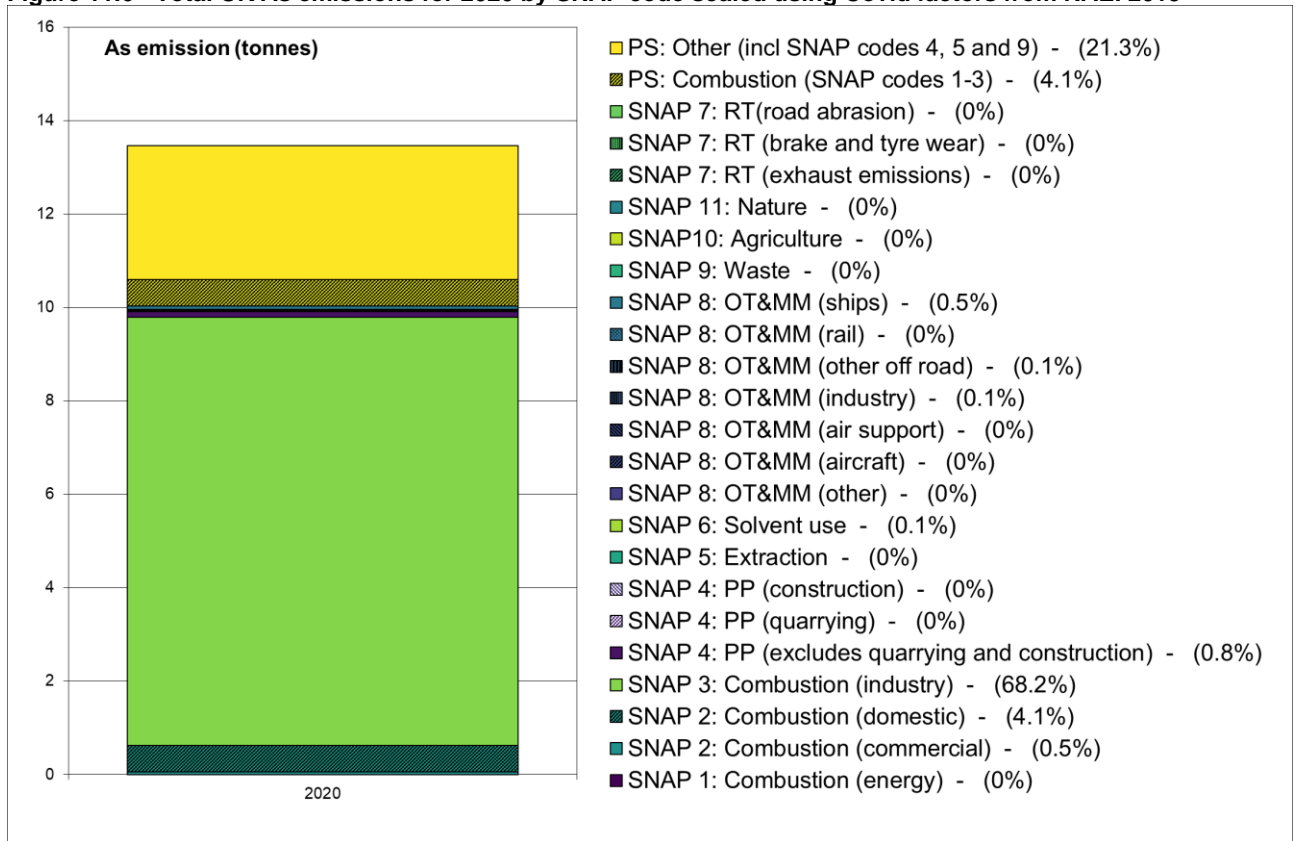
Figure 11.6 - Total UK As emissions for 2020 by SNAP code scaled using Covid factors from NAEI 2019
