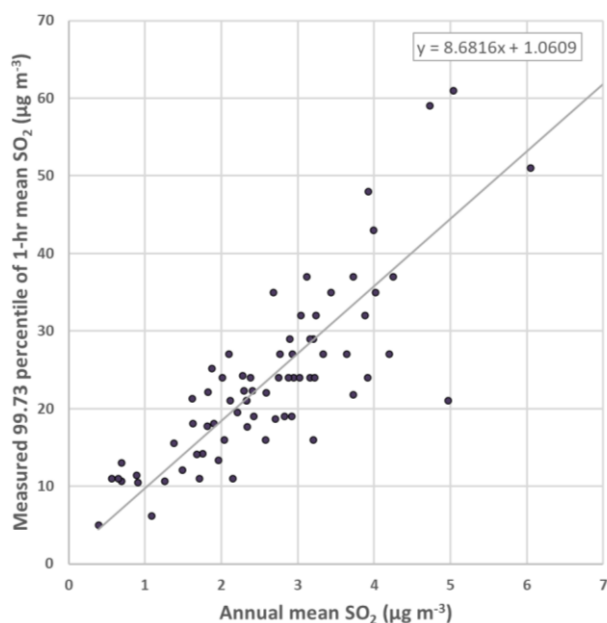
Figure 5.10 - Relationship between mean concentration and 99.73 percentile of 1-hour concentrations at sampling sites in Northern Ireland, 2008-2020
