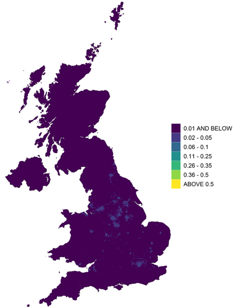
Figure 11.5 - Annual mean background Pb concentration, 2020 (µg m -3 )
