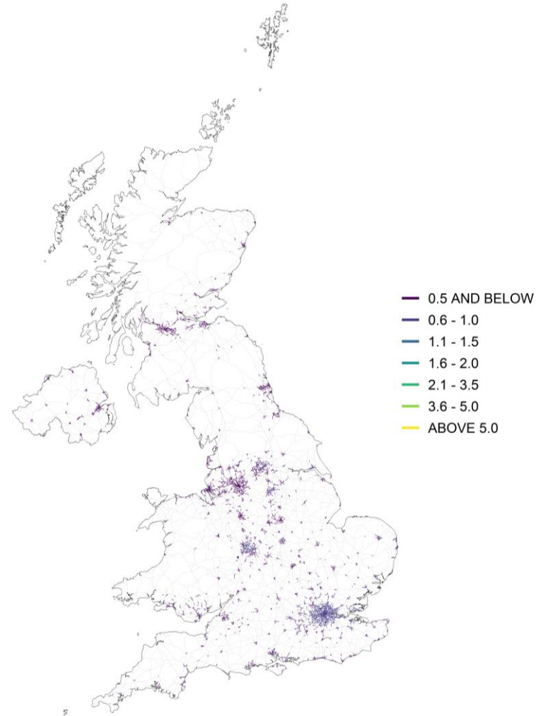
Figure 8.3 - Urban major roads, annual mean roadside benzene concentration, 2020 ( \mu\text{g m}^{-3} )
