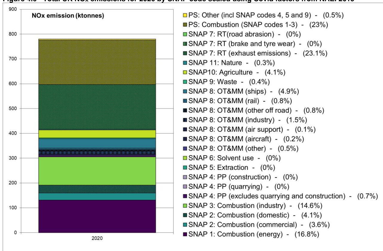
Figure 4.6 - Total UK NO x emissions for 2020 by SNAP code scaled using Covid factors from NAEI 2019
