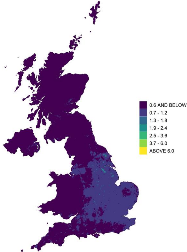
Figure 11.2 - Annual mean background As concentration, 2020 (ng m -3 )
