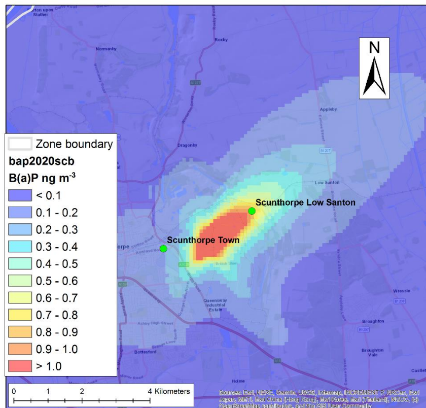
Figure 12.7 - Modelled total annual mean B(a)P concentration in the vicinity of the Appleby coke ovens at the Scunthorpe steelworks in 2020.
