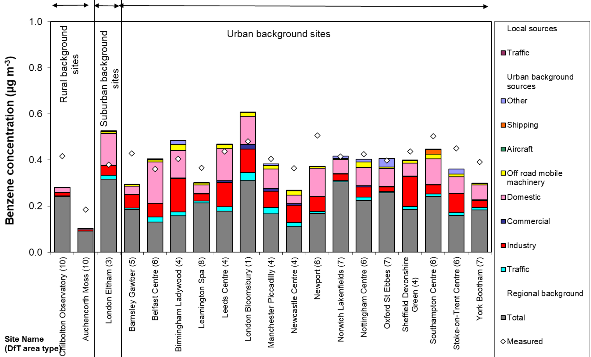
Figure 8.9 - Annual mean benzene source apportionment at background monitoring sites in 2020 (the area type of each site is shown in parenthesis after its name)
