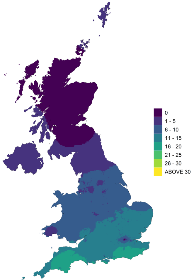
Figure 10.2 - Estimated number of days with an 8-hour mean ozone concentration above 120 \mu\text{g m}^{-3} , 2020
