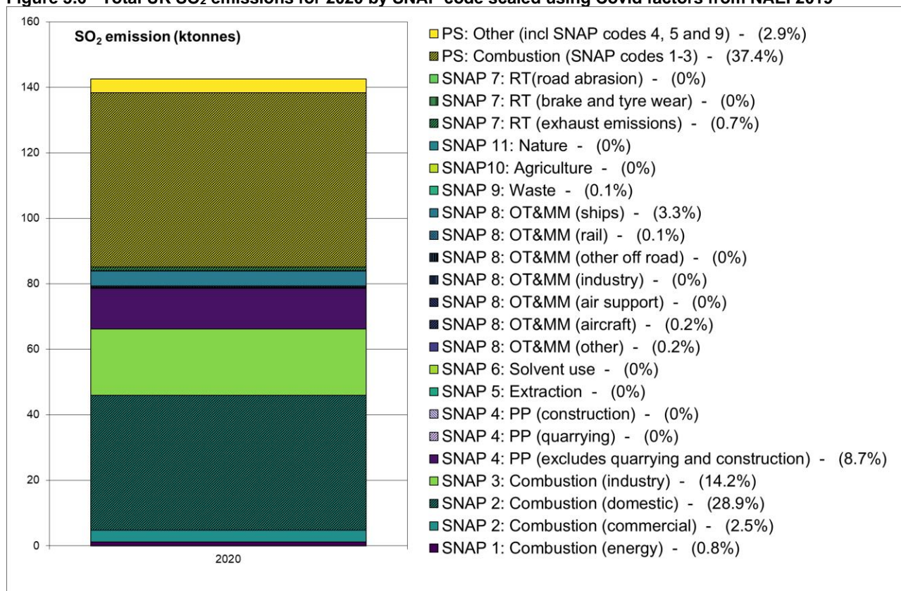
Figure 5.6 - Total UK SO 2 emissions for 2020 by SNAP code scaled using Covid factors from NAEI 2019
