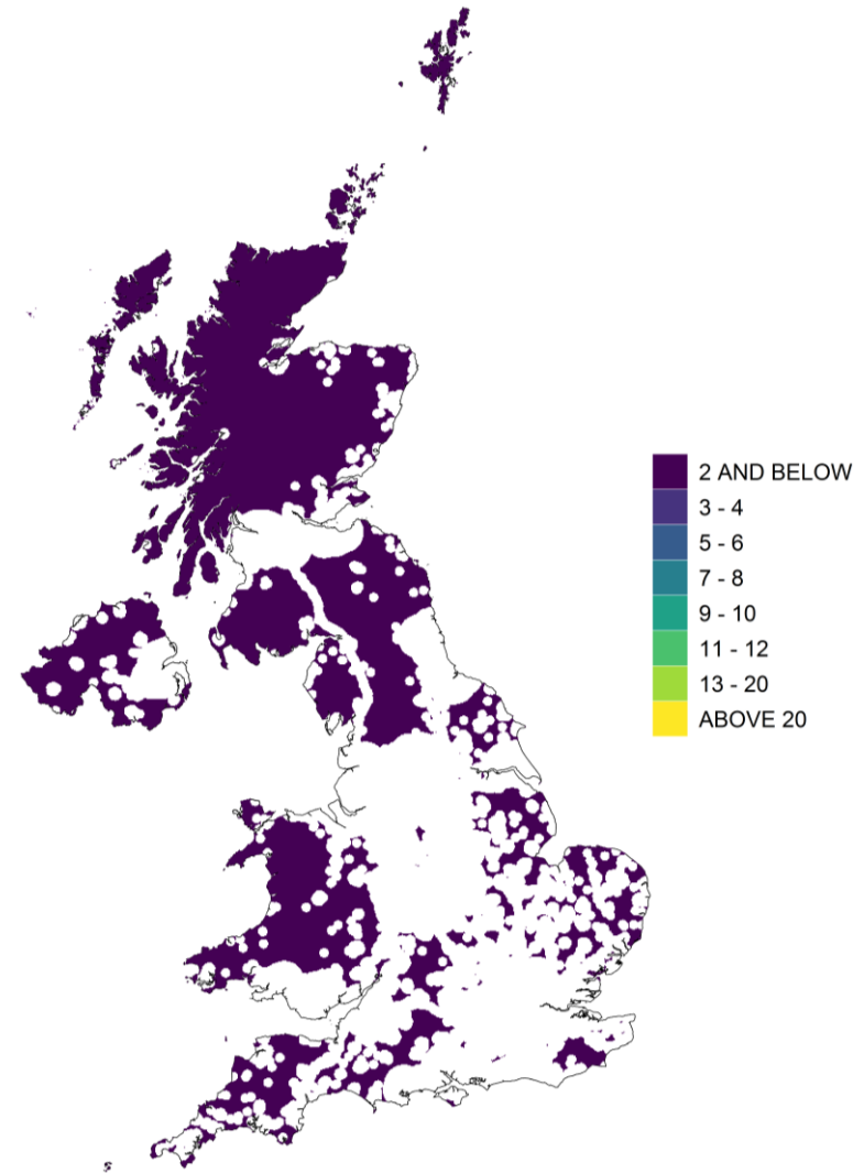
Figure 5.3 - Winter mean SO 2 concentration, 2019-2020 (µg m -3 ) in vegetation areas
