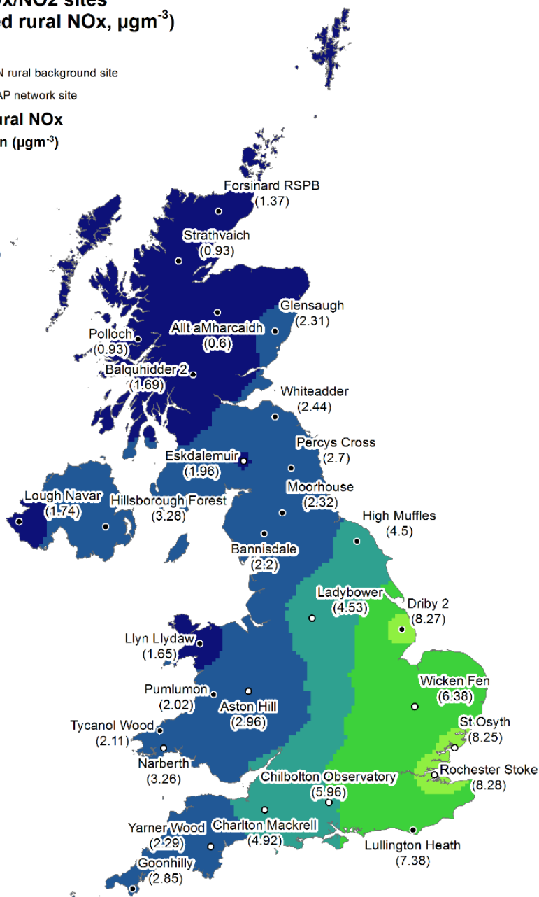
Figure 4.7 - Rural background NO x concentrations map with monitoring sites used in the interpolation (annual mean NO x concentrations for 2020 ( \mu\text{g m}^{-3} , as NO 2 ) are shown below the site name)
