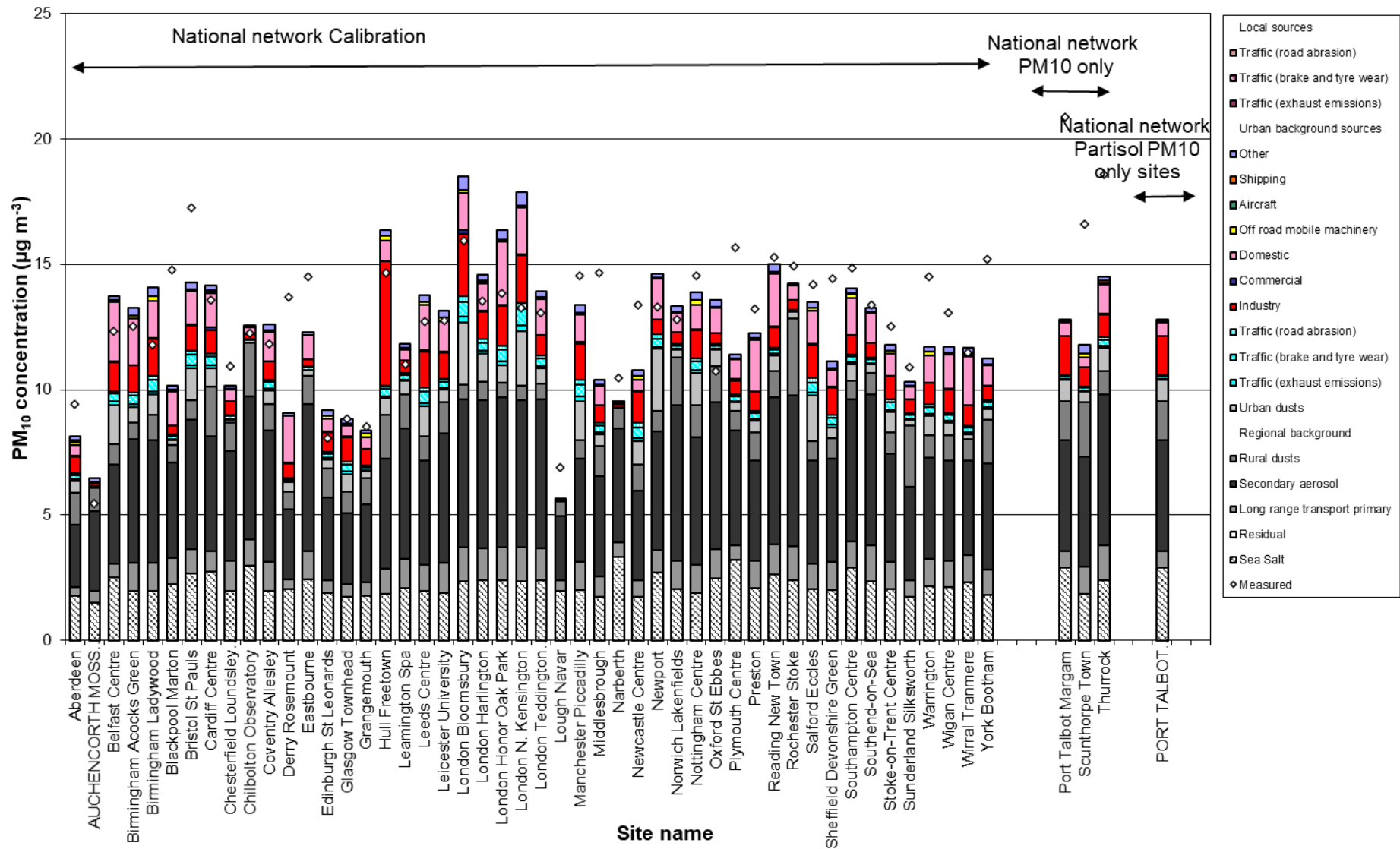
Figure 6.12 - Annual mean PM 10 source apportionment at background national network monitoring sites in 2020
