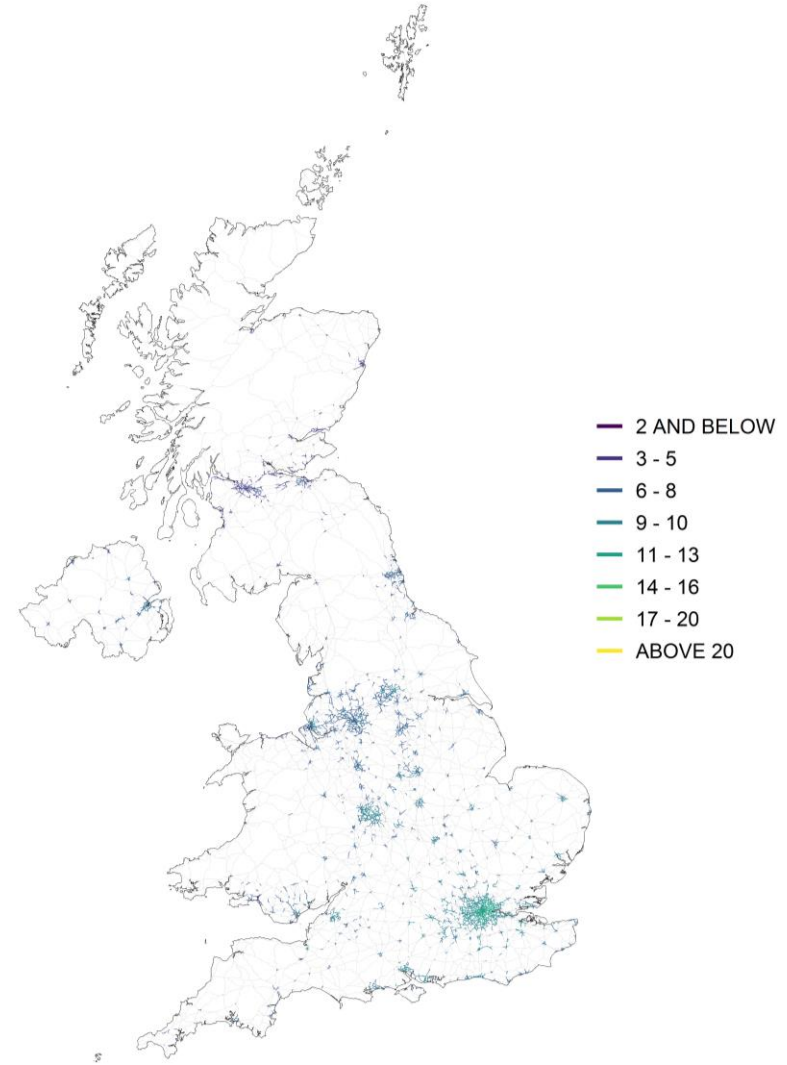
Figure 7.2 - Urban major roads, annual mean roadside PM 2.5 concentration, 2020 ( \mu\text{g m}^{-3} , gravimetric)
