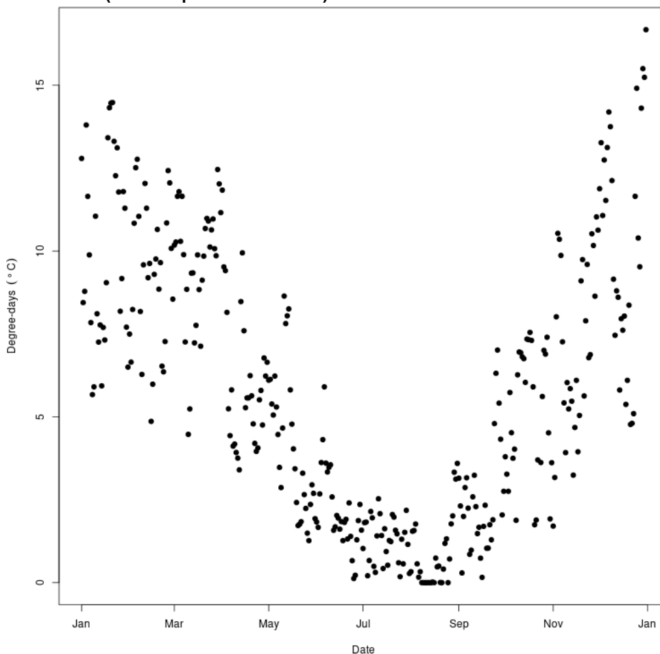
Figure A5.3 - Seasonal profile of degree days calculated for an example WRF grid cell in London in 2020 (base temperature of 15.5°C)
