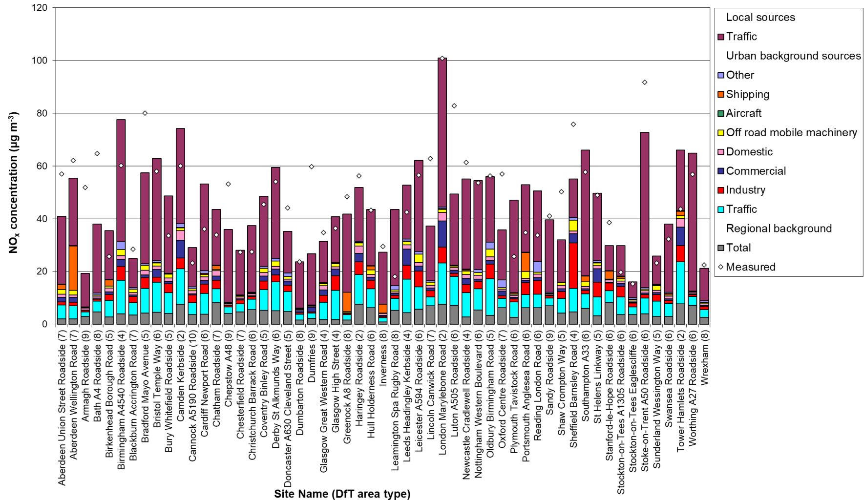
Figure 4.21 - Annual mean NO x source apportionment at roadside AURN monitoring sites in 2020 (area type of each site is shown in parenthesis after its name – see Table)
