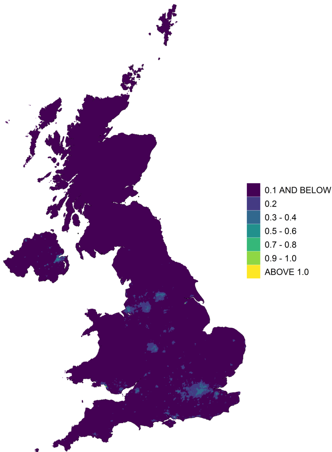
Figure 12.2 - Annual mean background B(a)P concentration, 2020 (ng m -3 )
