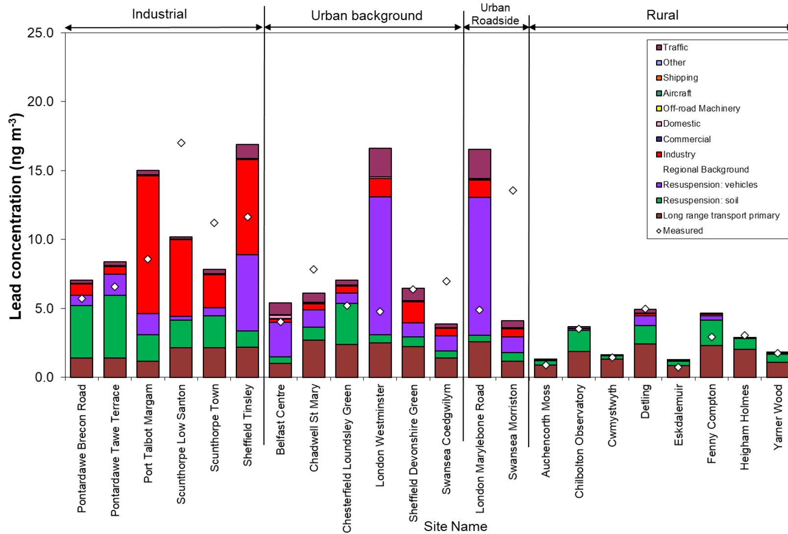
Figure 11.19 - Annual mean Pb source apportionment at monitoring sites in 2020.
