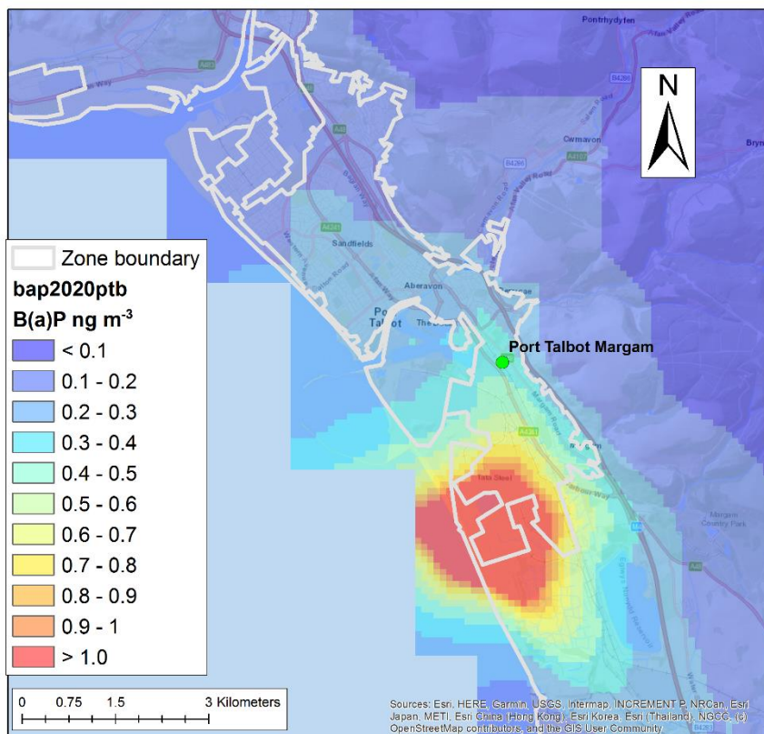
Figure 12.8 - Modelled total annual mean B(a)P concentration in the vicinity of the coke ovens at the Port Talbot steelworks in 2020
