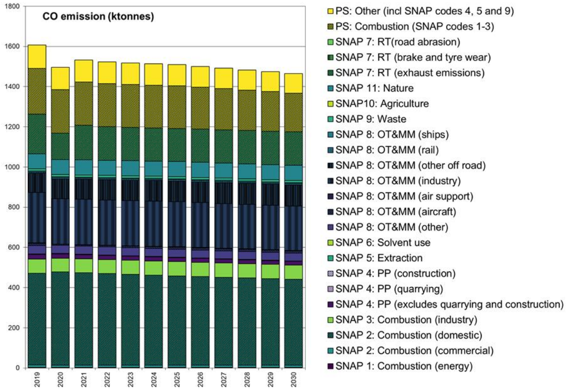
Figure 9.1 - Total UK CO emissions for 2019 and emissions projections up to 2030 by SNAP code from NAEI 2019
