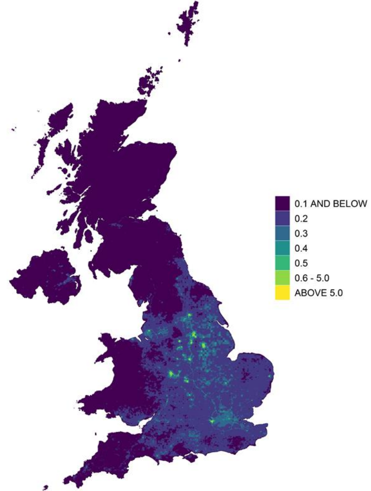
Figure 11.3 - Annual mean background Cd concentration, 2020 (ng m -3 )
