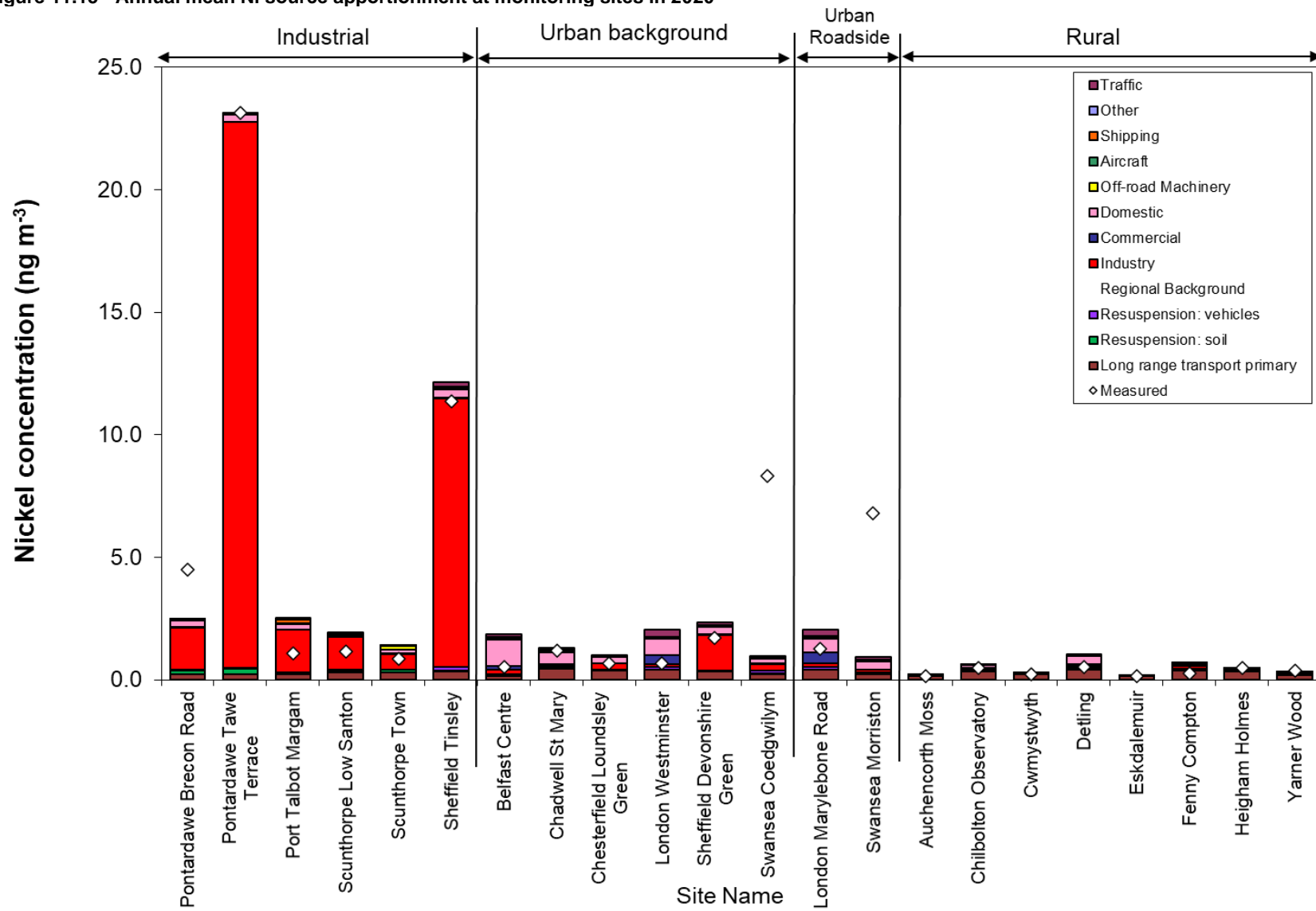
Figure 11.15 - Annual mean Ni source apportionment at monitoring sites in 2020
