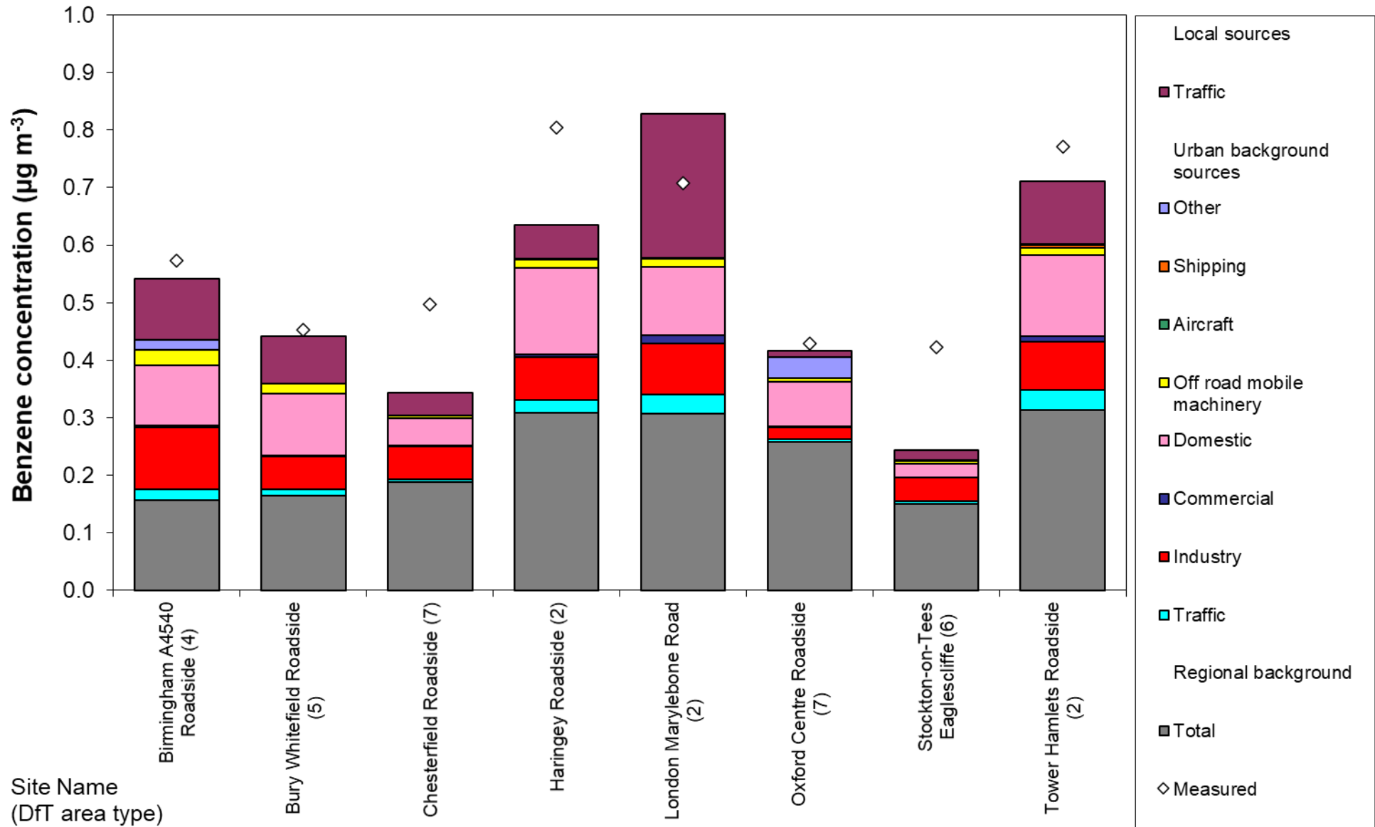
Figure 8.10 - Annual mean benzene source apportionment at roadside monitoring sites in 2020 (the area type of each site is shown in parenthesis after its name)
