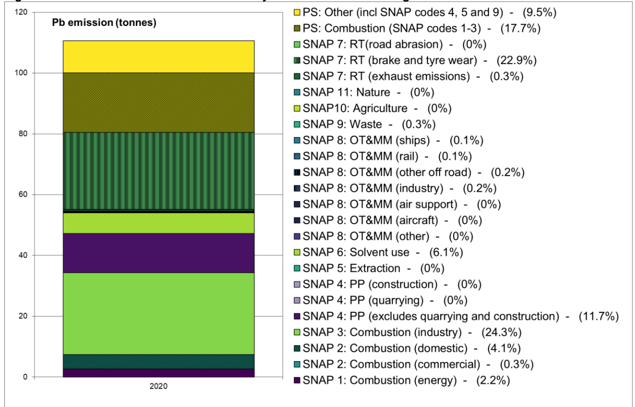
Figure 11.9 - Total UK Pb emissions for 2020 by SNAP code scaled using Covid factors from NAEI 2019
