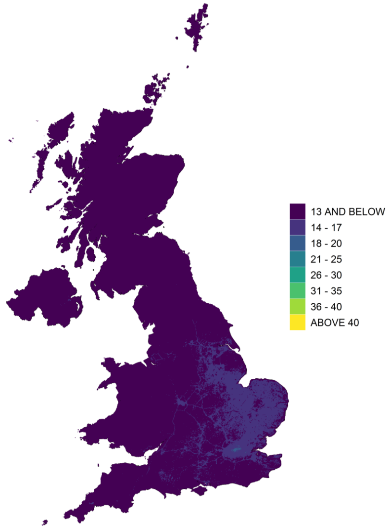
Figure 6.1 - Annual mean background PM 10 concentration, 2020 ( \mu\text{g m}^{-3} , gravimetric)
