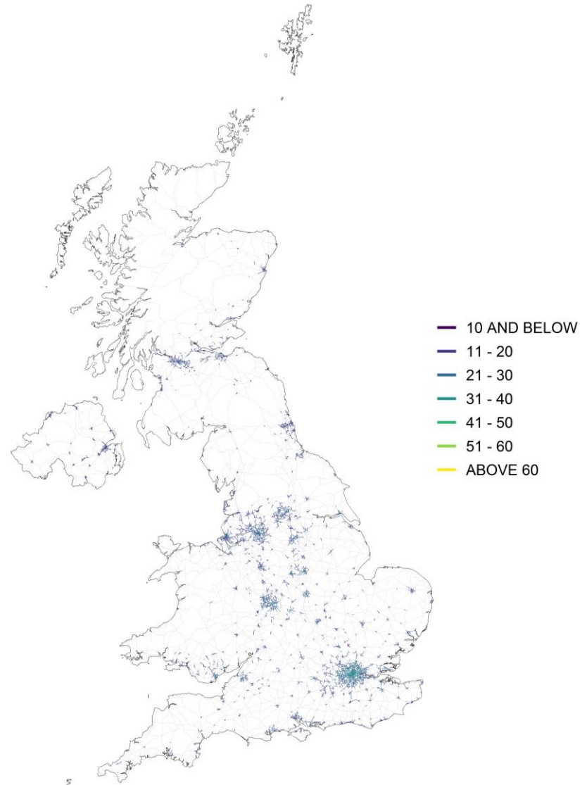
Figure 4.2 - Urban major roads, annual mean roadside NO 2 concentration, 2020 ( \mu\text{g m}^{-3} )
