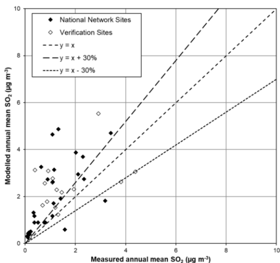
Figure 5.12 - Verification of annual mean SO 2 model, 2020
