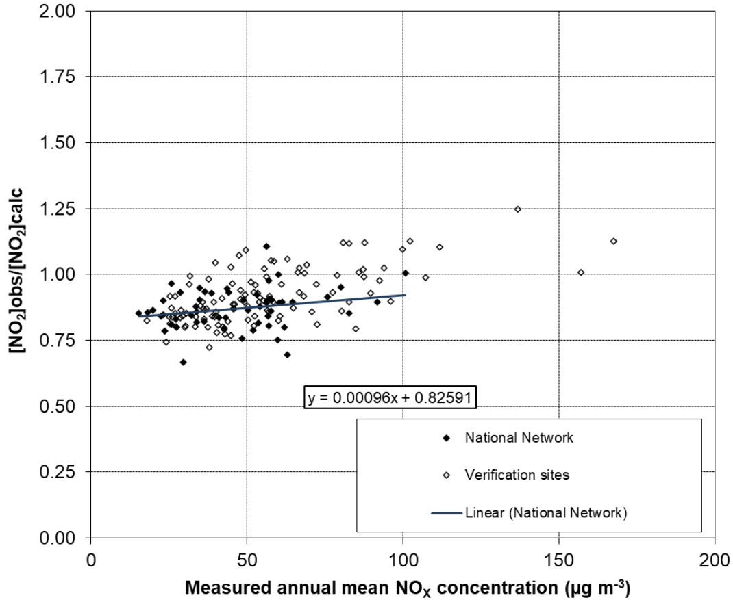
Figure 4.14 - Roadside NO 2 calibration curve (NB verification sites are shown for reference here, but were not used in calculating the calibration factors), 2020
