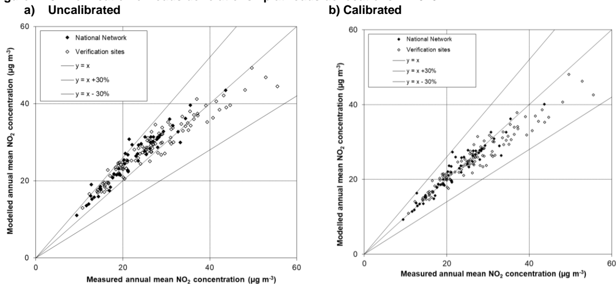
Figure 4.15 - Verification of roadside relationship at roadside locations in 2020
