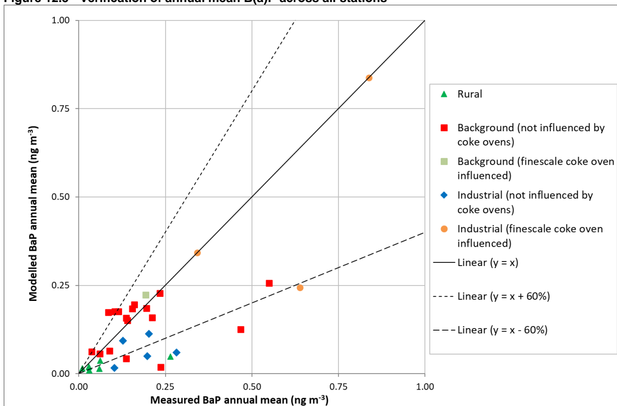
Figure 12.5 - Verification of annual mean B(a)P across all stations
