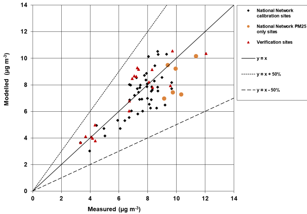
Figure 7.8 - Verification of roadside annual mean PM 2.5 model 2020
