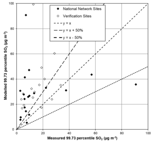
Figure 5.13 - Verification of 99.73 percentile of 1-hour mean SO 2 model, 2020
