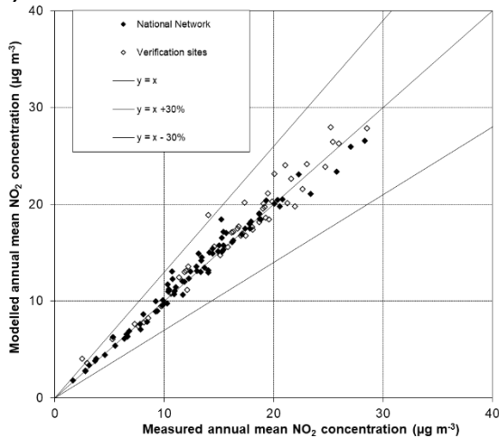
Figure 4.13 - Verification of background relationship at background locations in 2020
