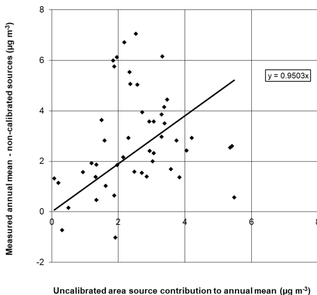
Figure 6.8 - Calibration of PM 10 area source model 2020 (µg m -3 , gravimetric)
