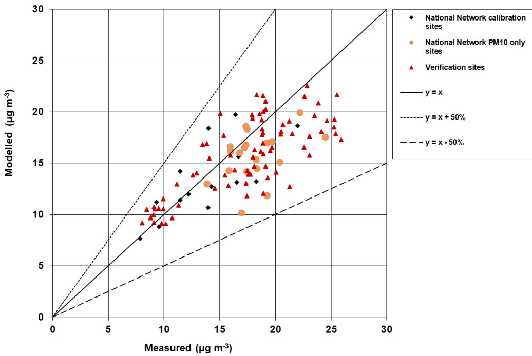
Figure 6.11 - Verification of roadside annual mean PM 10 model 2020
