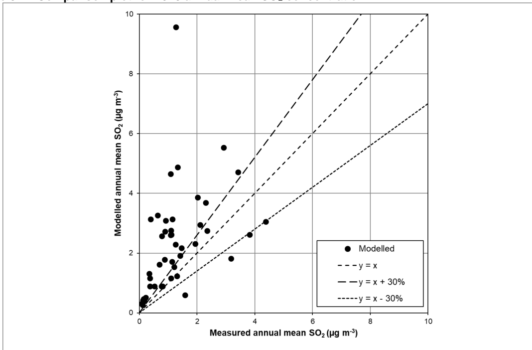
Figure 5.7 - Comparison plot for 2020 annual mean SO 2 concentration
