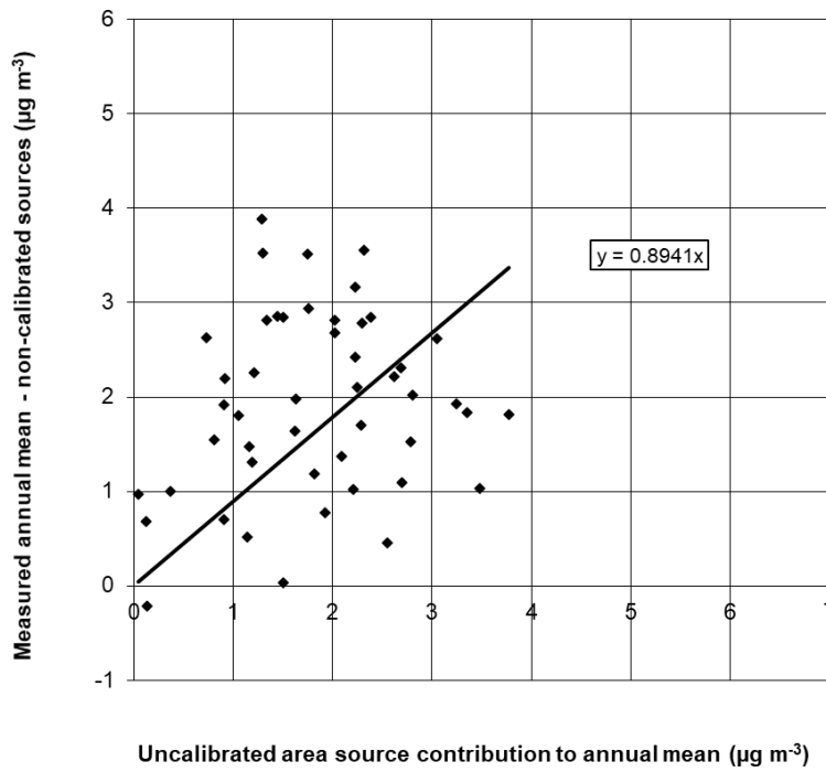
Figure 7.5 - Calibration of PM 2.5 area source model 2020 (µg m -3 , gravimetric)
