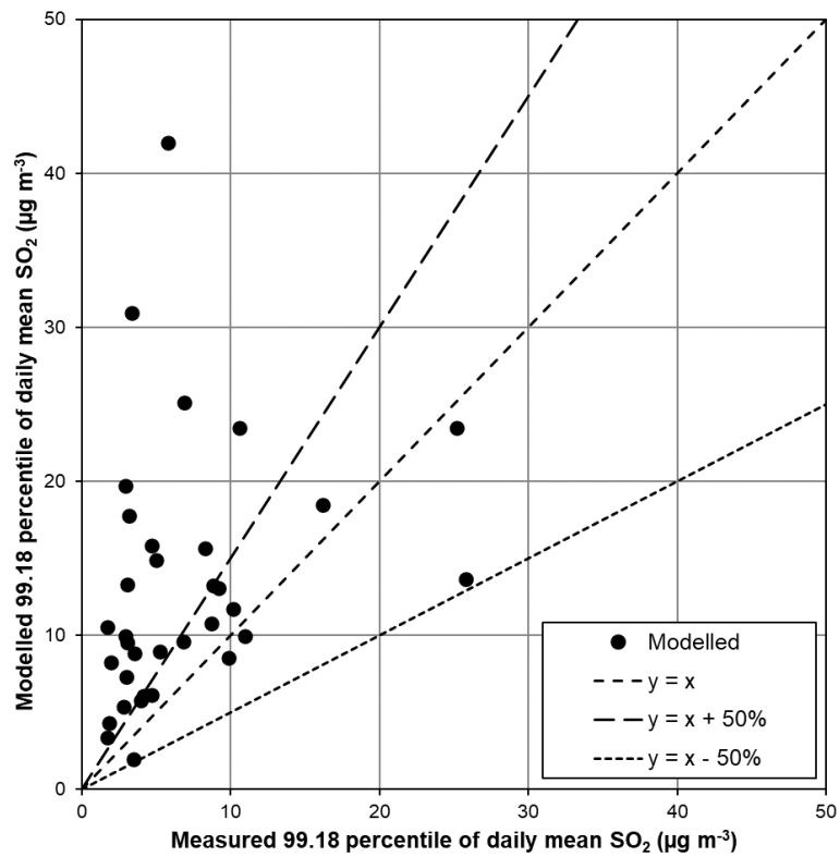
Figure 5.9 - Comparison plot for 2020 99.18 percentile of 24-hour mean SO 2 concentrations
