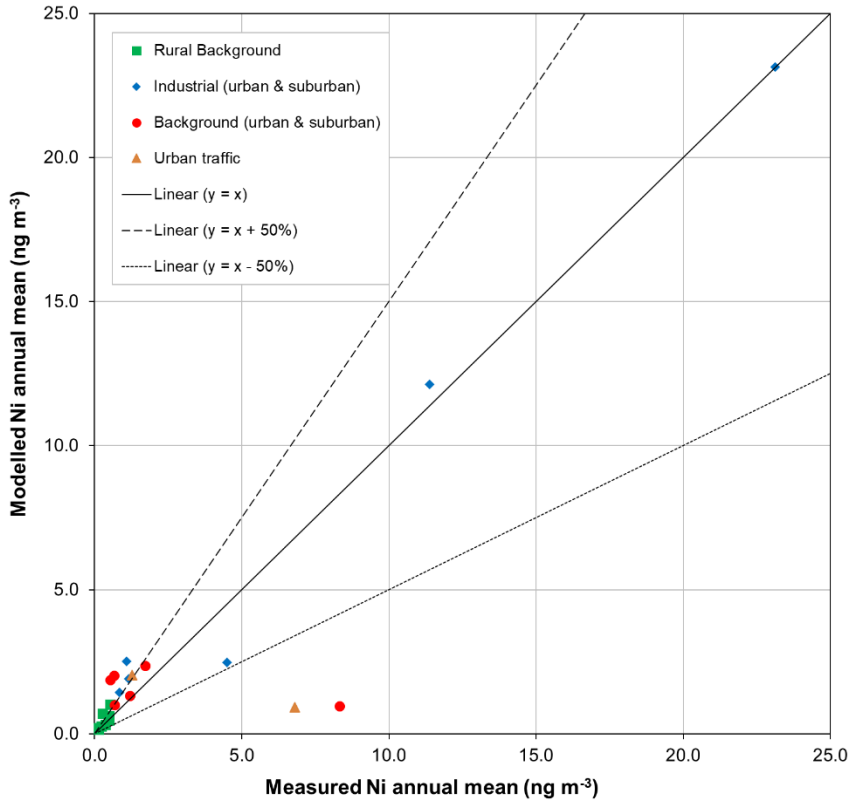
Figure 11.14 - Verification of annual mean Ni across all sites.
