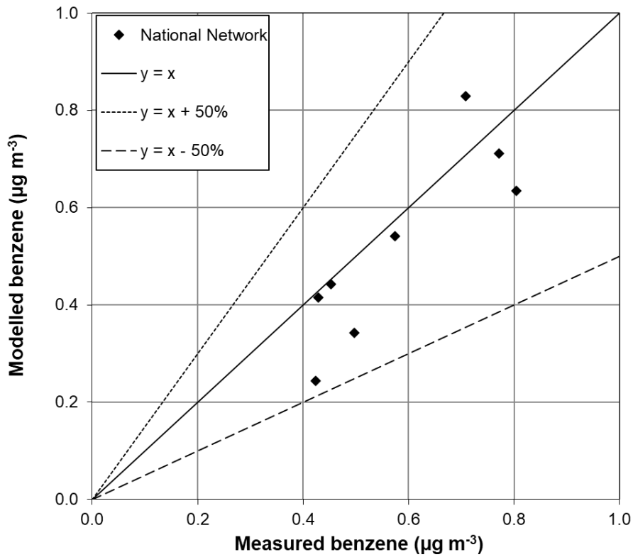
Figure 8.8 - Verification of roadside annual mean benzene model 2020
