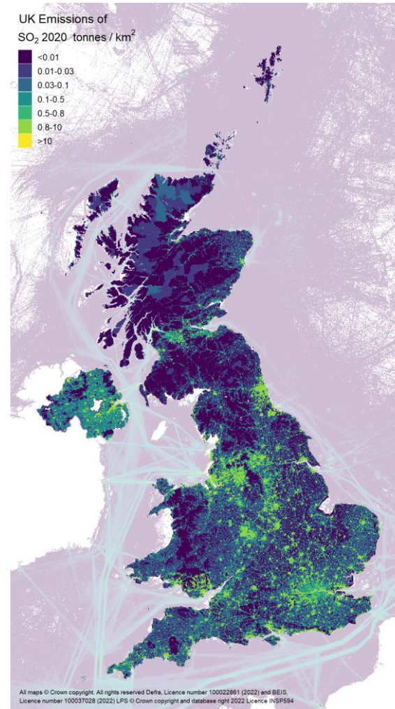
Figure 5-5 SO 2 0-1km column mean (large-scale bias corrected) in Dobson unit in 2020 (Left). Total NAEI SO 2 emissions in tonnes in 2020 (Right). Both maps are plotted in 1x1km
