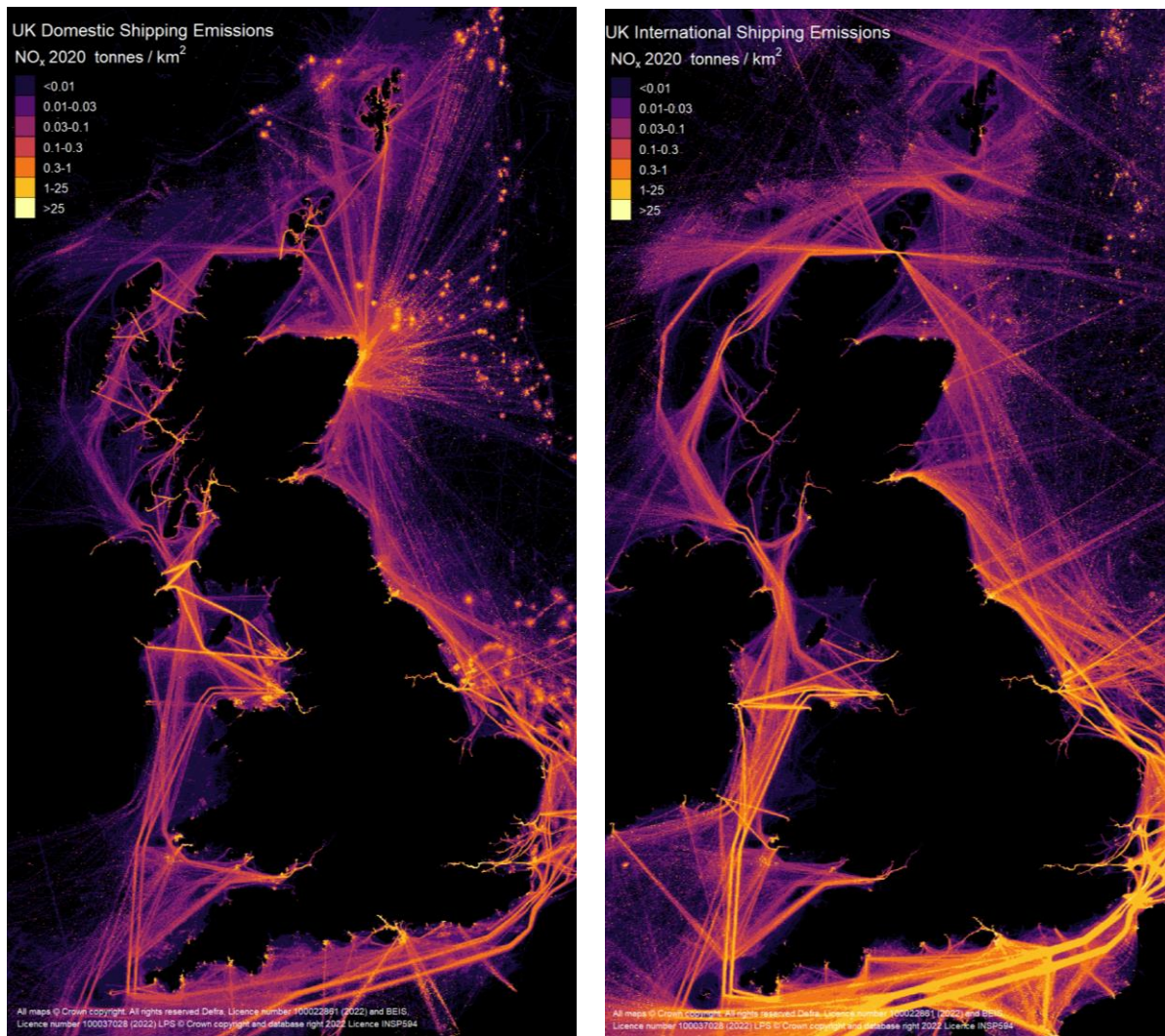
Figure 3-9 NO x shipping emissions by trip type for 2020.
