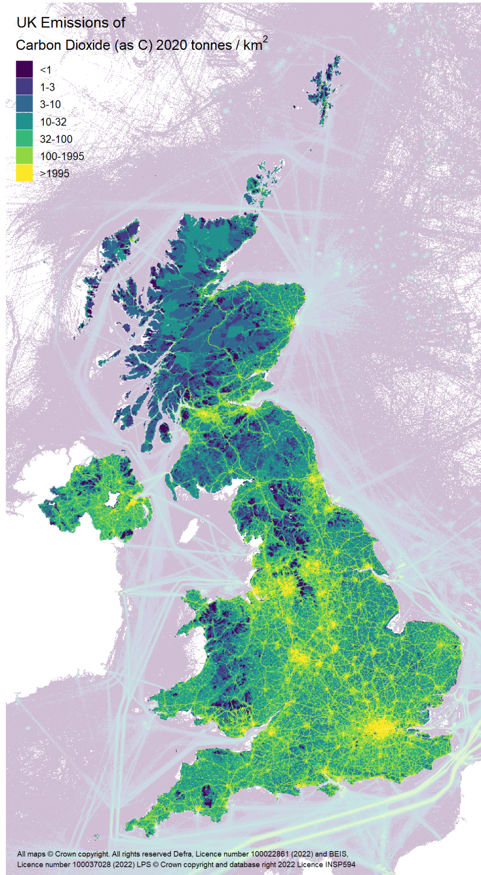
Figure 4-4 UK total CO 2 emissions in 2020 excluding emissions from Land Use Change
