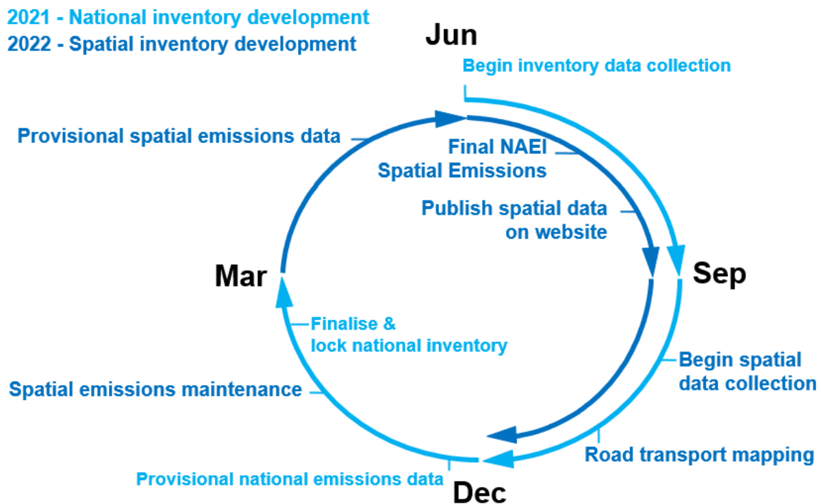
Figure 1-1 The 2020 NAEI spatial inventory development cycle
