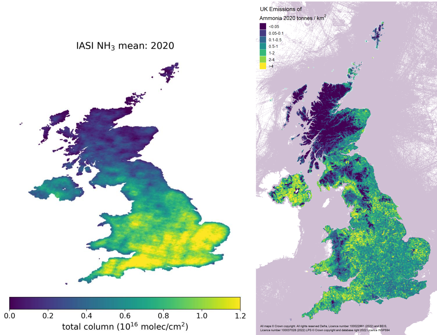
Figure 5-6 NH 3 total column mean in molecules/cm 2 in 2020 (Left). Total NAEI NH 3 emissions in tonnes in 2020 (Right). The IASI map is plotted in 2x2km while the NAEI map is plotted in 1x1km
