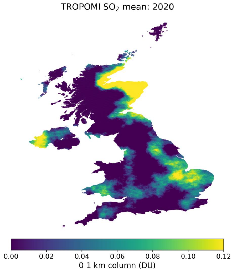
Figure 5-5 SO 2 0-1km column mean (large-scale bias corrected) in Dobson unit in 2020 (Left). Total NAEI SO 2 emissions in tonnes in 2020 (Right). Both maps are plotted in 1x1km
