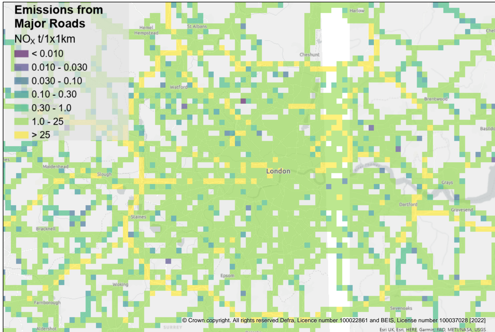
Figure 3-6 2020 NO x road transport emissions on major roads aggregated to 1x1 km resolution
