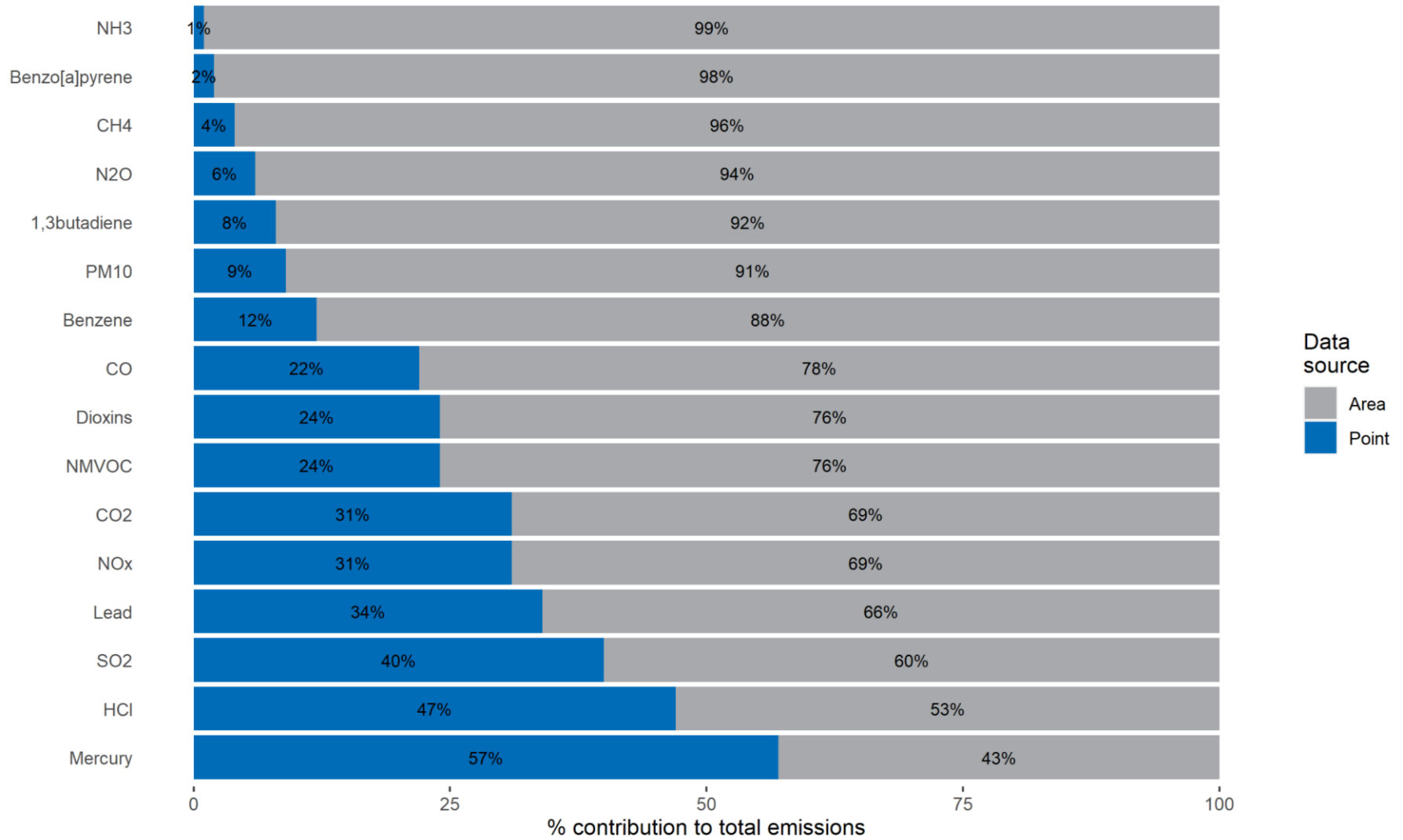
Figure 5-1 Contribution of point sources to mapped emission totals (2020)
