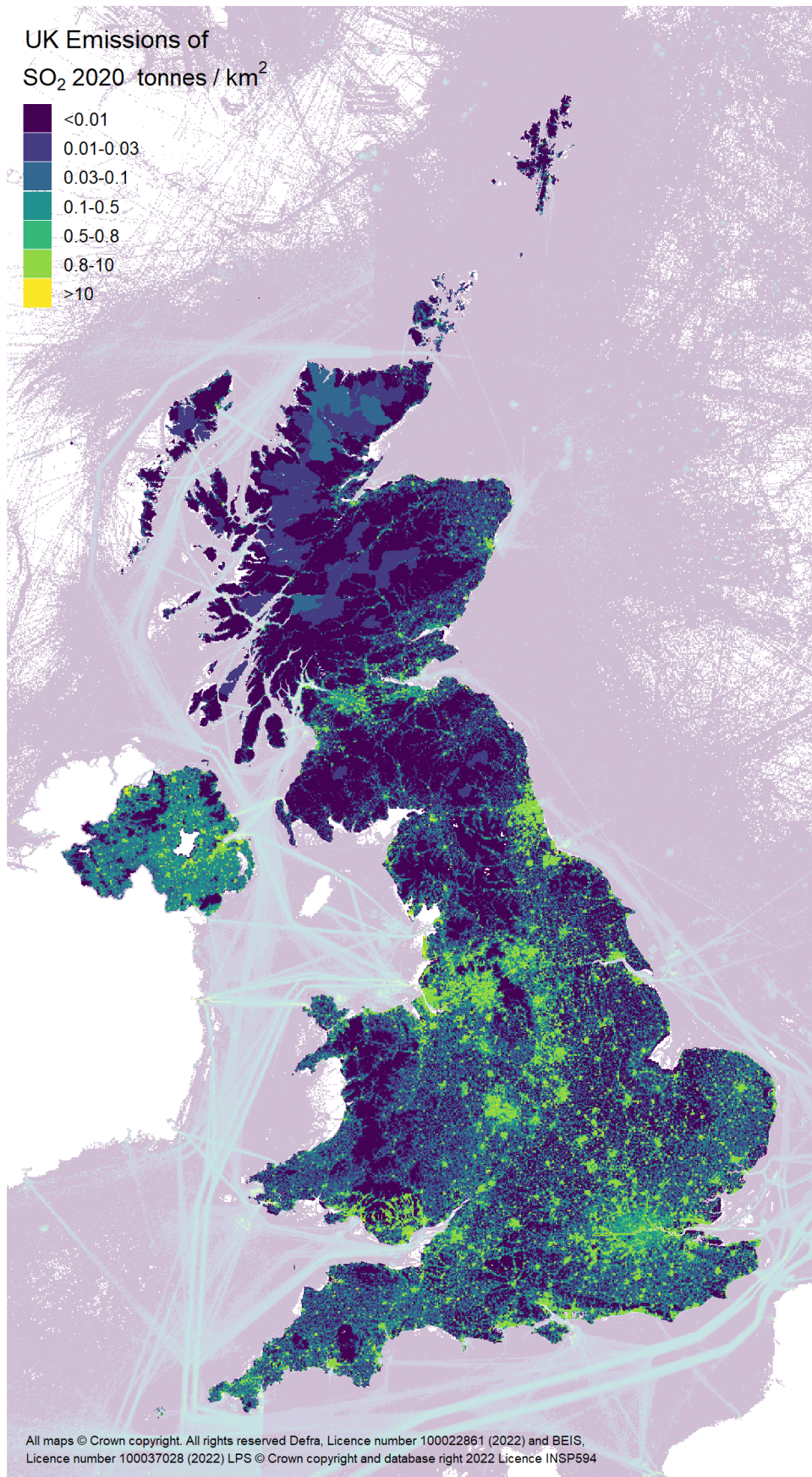
Figure 4-3 UK total SO 2 emissions in 2020
