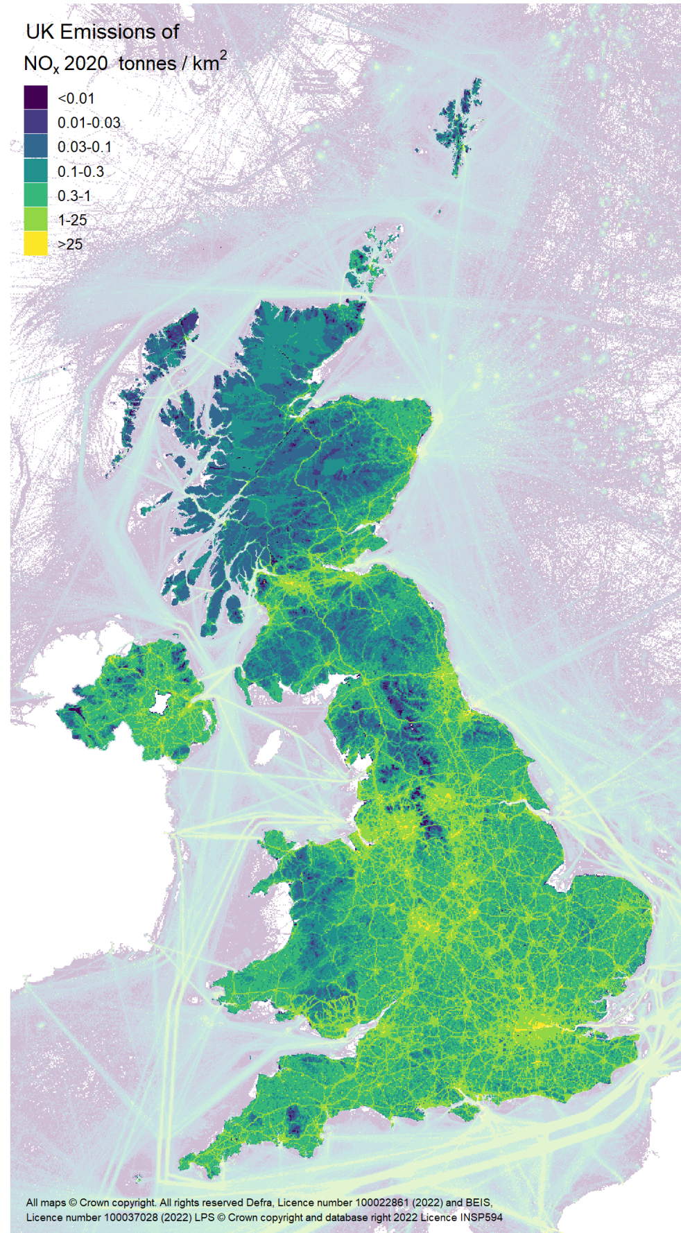
Figure 2-4 UK total NO x emissions in 2020
