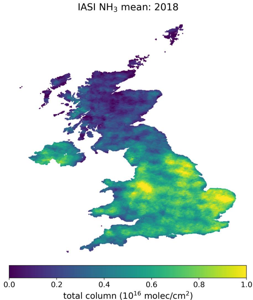
Figure 5-7 \text{NH}_3 total column mean in molecules/cm 2 in 2018 in 2x2km.
