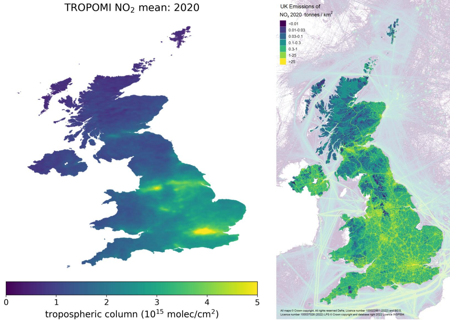
Figure 5-4 NO 2 tropospheric column mean in molecules/cm 2 in 2020 (Left). Total NAEI NO x emissions in tonnes for 2020 (Right). Both maps are plotted in 1x1km
