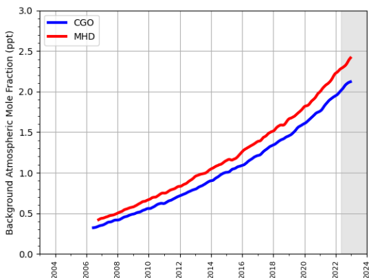
(e) HFC-227ea
