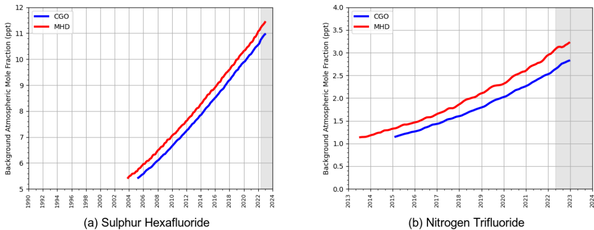
Figure A 6.19 (a) shows the hemispheric background atmospheric concentrations of sulphur hexafluoride (SF 6 ) from 2004 onwards. The background trend is monotonic and positive and in 2022 the Northern Hemispheric background concentration increased by 0.4 ppt.
