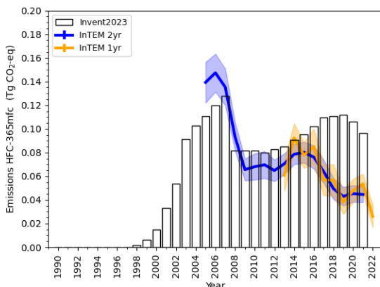
(c) HFC-365mfc
