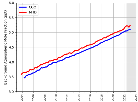
(b) PFC-116
