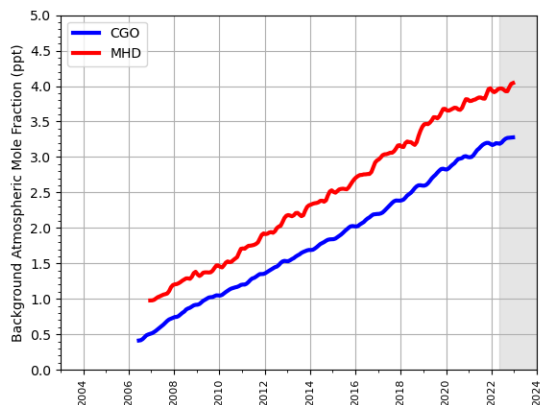
(f) HFC-245fa
