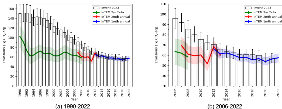
Figure A 6.2 Verification of the UK emission inventory estimates for CH 4 in Tg CO 2 -eq yr -1 (a) from 1990 and (b) from 2006. GHGI estimates are shown in black. InTEM 2-site 2-year estimates are shown in green ( \pm 1\sigma ). InTEM full network, 1-month annualised, estimates are shown in blue ( \pm 1\sigma ). InTEM 7-site, 2-month annualised, estimates are shown in red ( \pm 1\sigma ).
