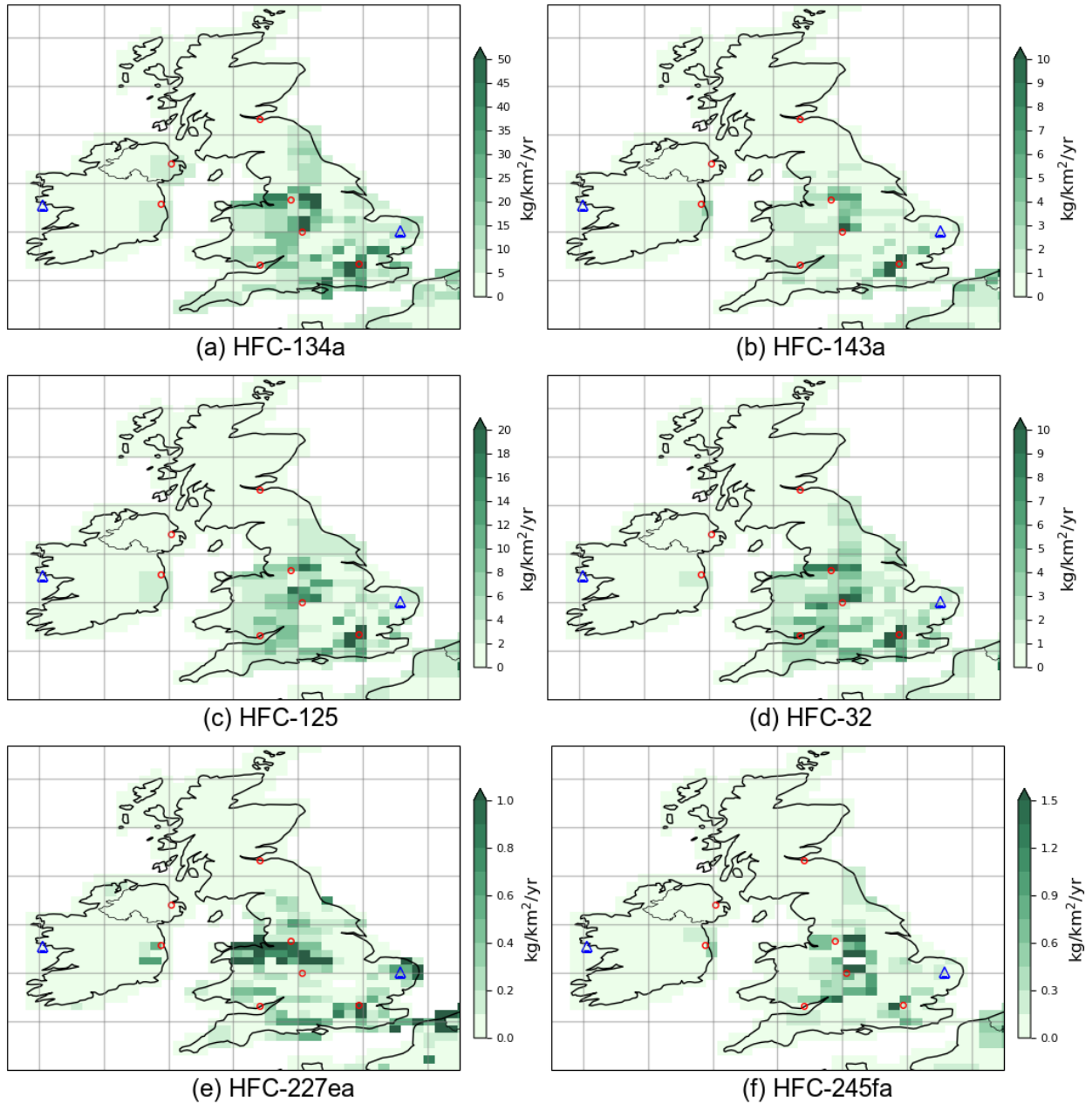
Figure A 6.13 Four-year average HFC-134a InTEM emission estimates ( \text{kg km}^{-2} \text{yr}^{-1} ) 2019-2022. The observation stations are shown as blue triangles. Major cities are shown as red circles.
