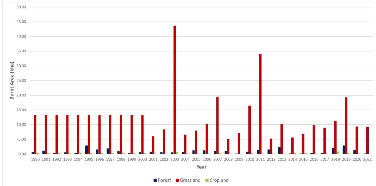
Figure A 3.16 Time series of wildfire burnt areas in the UK 1990 to the current inventory year
