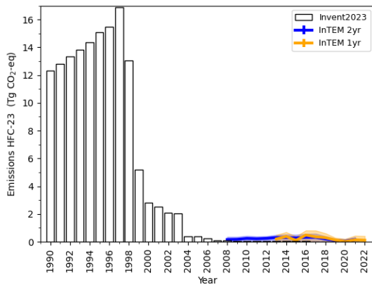
(a) HFC-23
