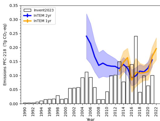
(c) PFC-218
