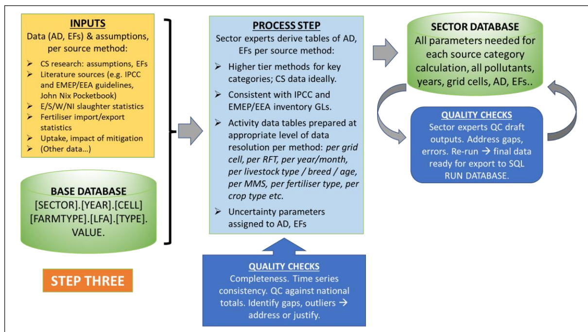
Figure A 3.6 Inventory Model Data Flows: Source AD to Sector Database
