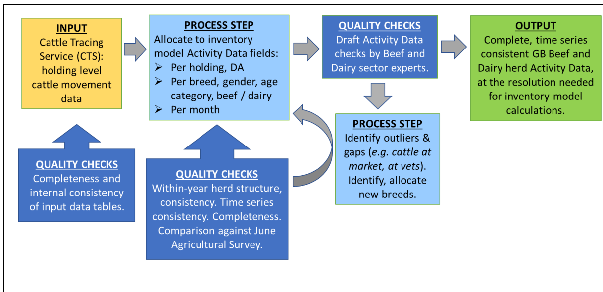
Figure A 3.5 Inventory Model Data Flows: Pre-processing of the CTS
