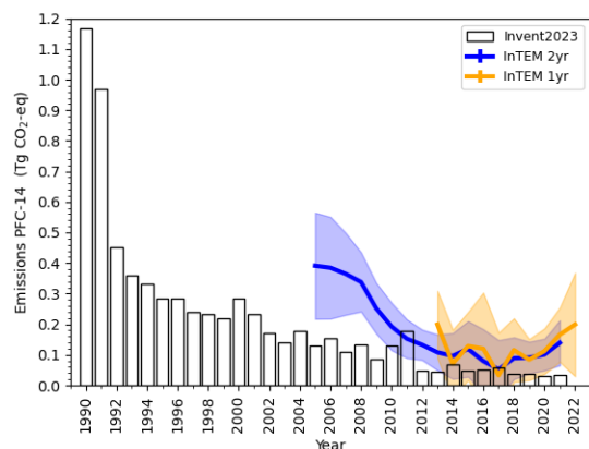
(a) PFC-14
