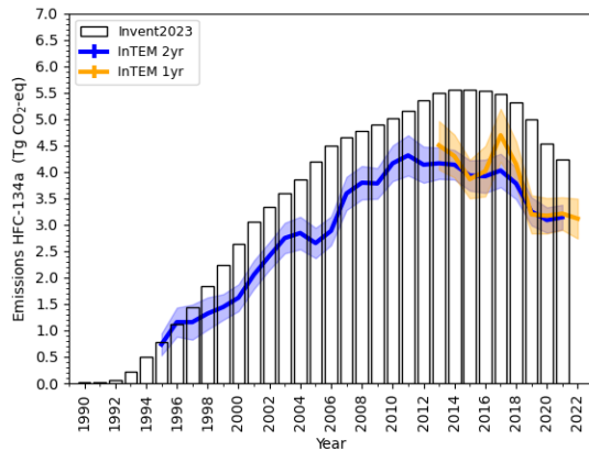
(a) HFC-134a
