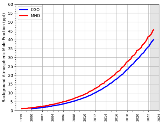
(c) HFC-125
