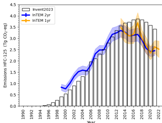
(c) HFC-125
