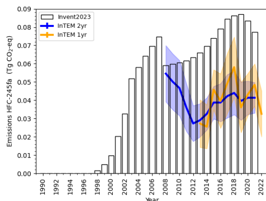
(f) HFC-245fa
