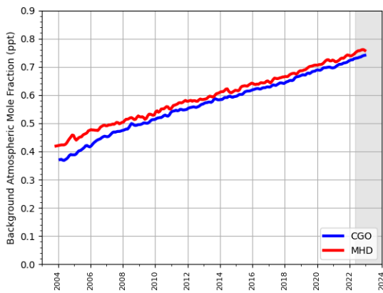
(c) PFC-218
