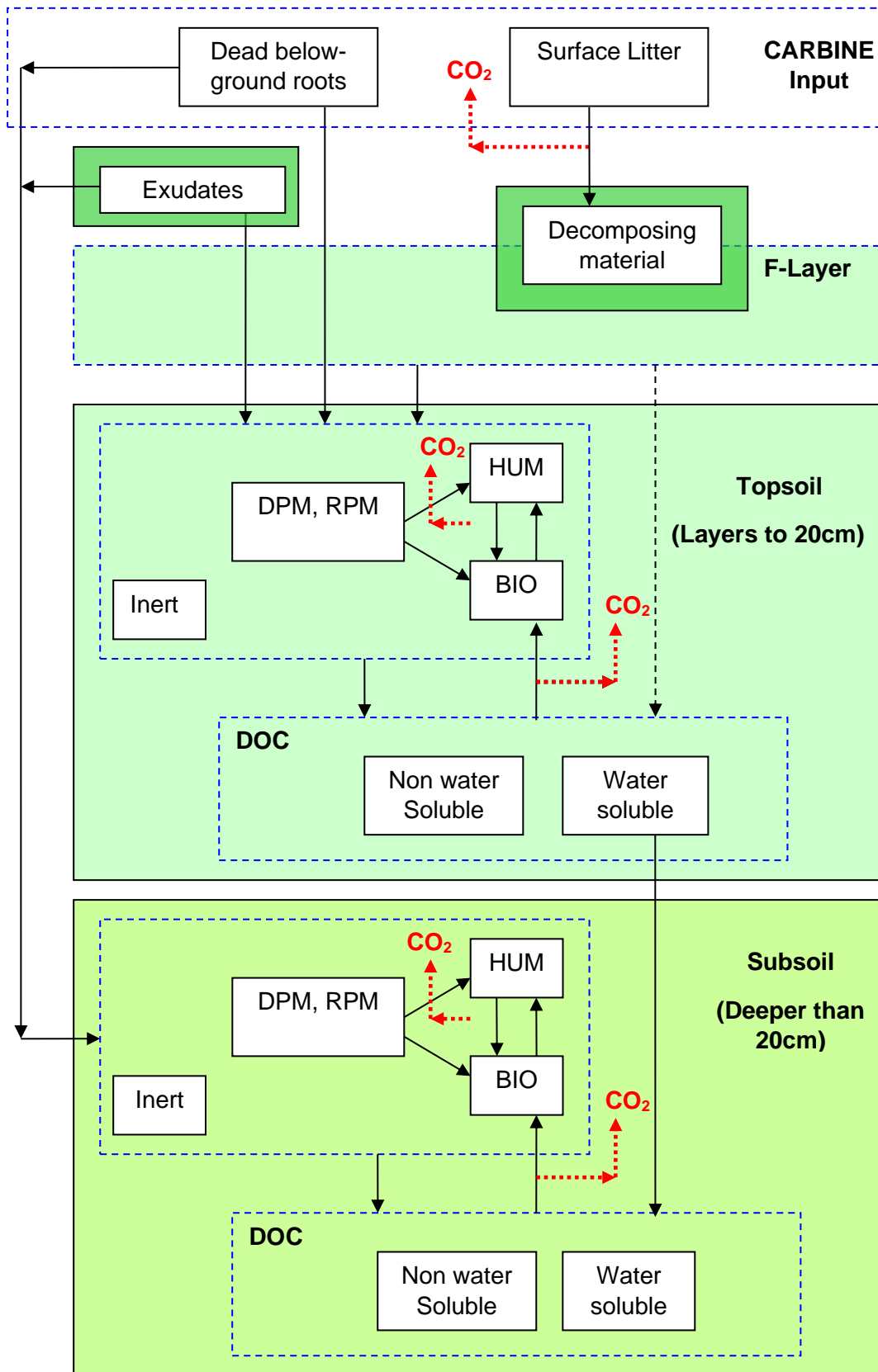
Figure A 3.9 The CARBINE SCOTIA model
