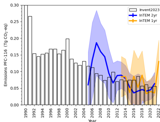
(b) PFC-116
