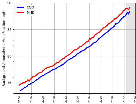
(a) PFC-14
