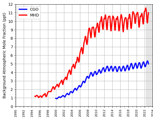
(c) HFC-152a
