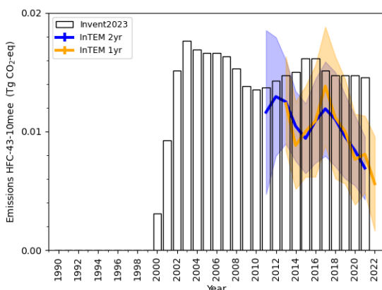
(e) HFC-43-10mee
