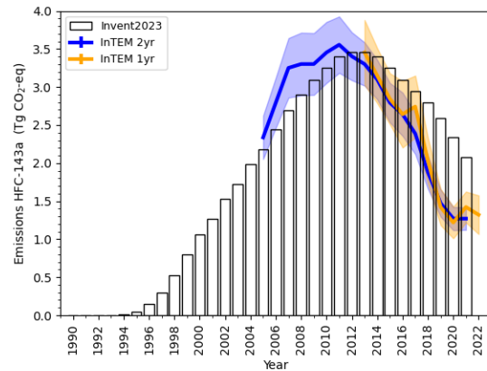
(b) HFC-143a
