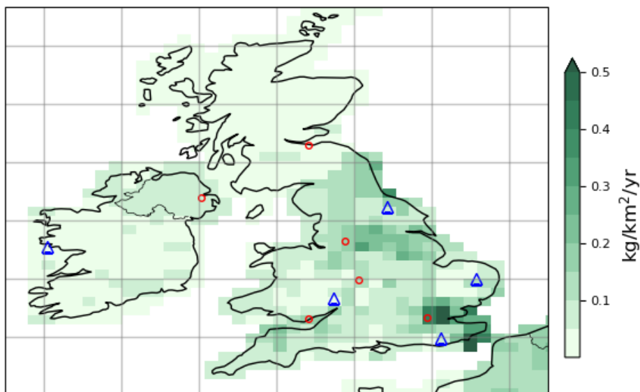
Figure A 6.22 Four-year average SF 6 InTEM emission estimates (kg km -2 yr -1 of gas) 2019-2022. The observation stations are shown as blue triangles. Major cities are shown as red circles.
