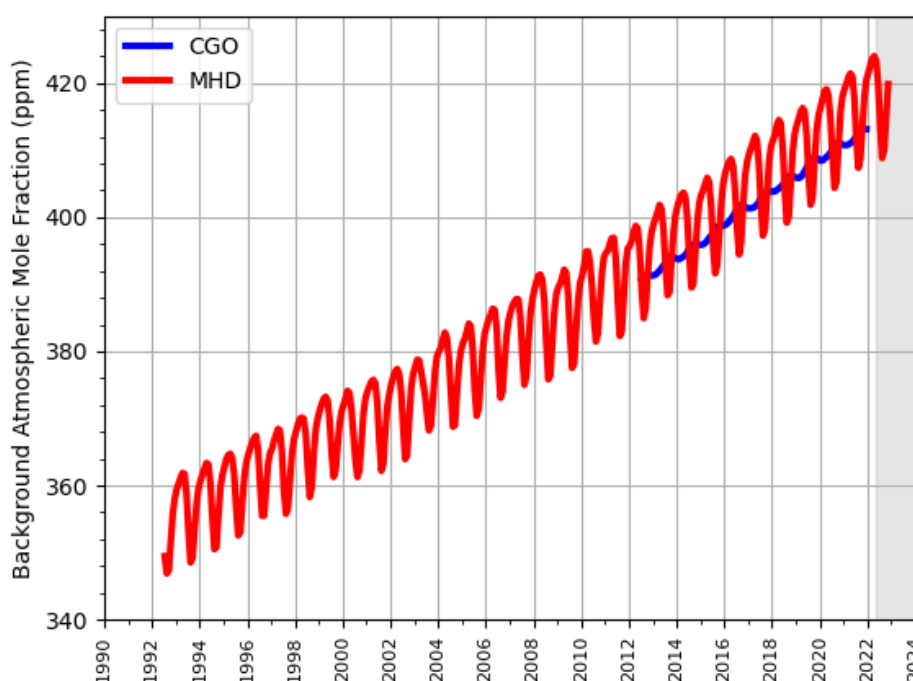
Figure A 6.25 Background Northern Hemisphere monthly concentrations of CO 2 estimated from MHD, Ireland observations (data obtained from LSCE equipment through a data sharing agreement) are shown in red, and background Southern Hemisphere monthly concentrations from CGO, Tasmania are shown in blue. Grey shading represents unratified data.
