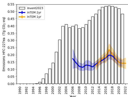
(e) HFC-227ea
