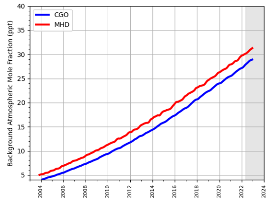
(b) HFC-143a
