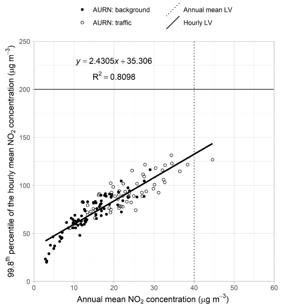
Figure 3.4 - Plot of annual mean against 99.8th percentile hourly NO 2 concentrations in 2022
