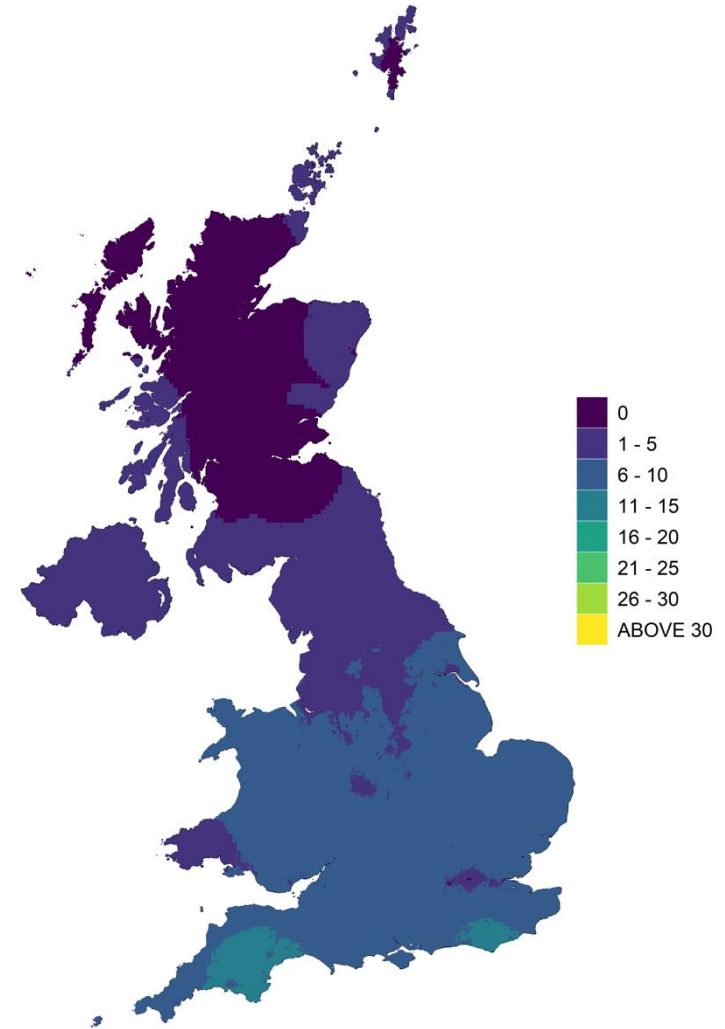
Figure 9.3 - Estimated average number of days with an 8-hour mean ozone concentration above 120 \mu\text{g m}^{-3} , 2020 to 2022
