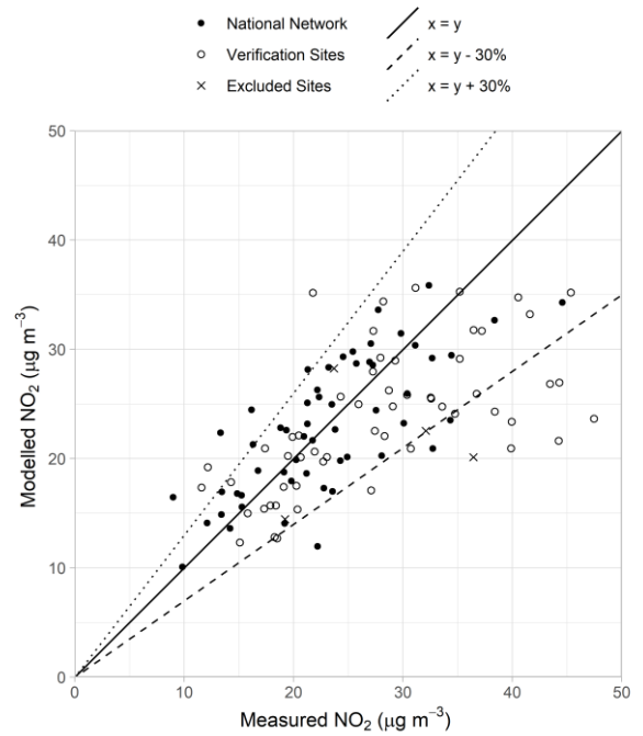
Figure 3.19 - Verification of roadside annual mean NO 2 model 2022
