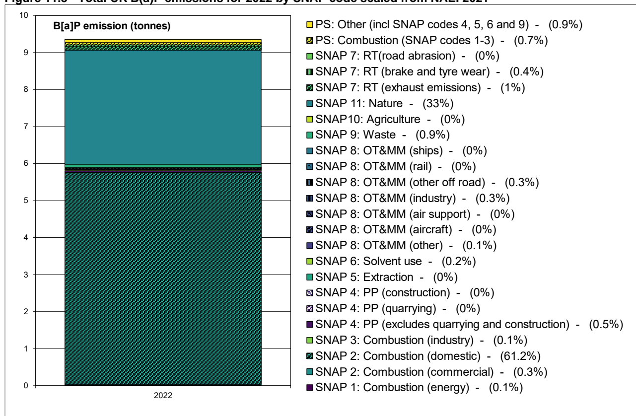
Figure 11.3 - Total UK B(a)P emissions for 2022 by SNAP code scaled from NAEI 2021
