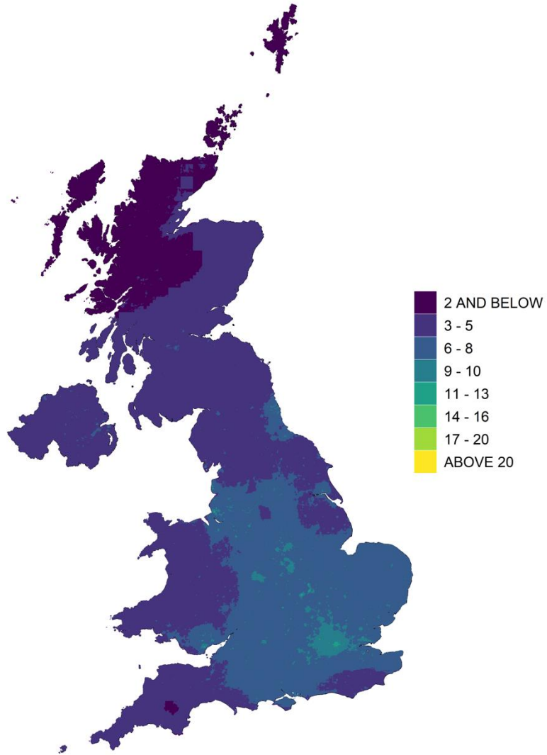
Figure 6.1 - Annual mean background PM 2.5 concentration, 2022 ( \mu\text{g m}^{-3} , gravimetric)
