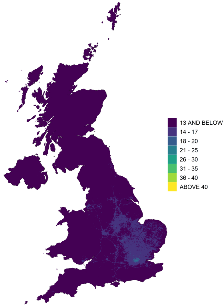
Figure 5.1 - Annual mean background PM 10 concentration, 2022 ( \mu\text{g m}^{-3} , gravimetric)
