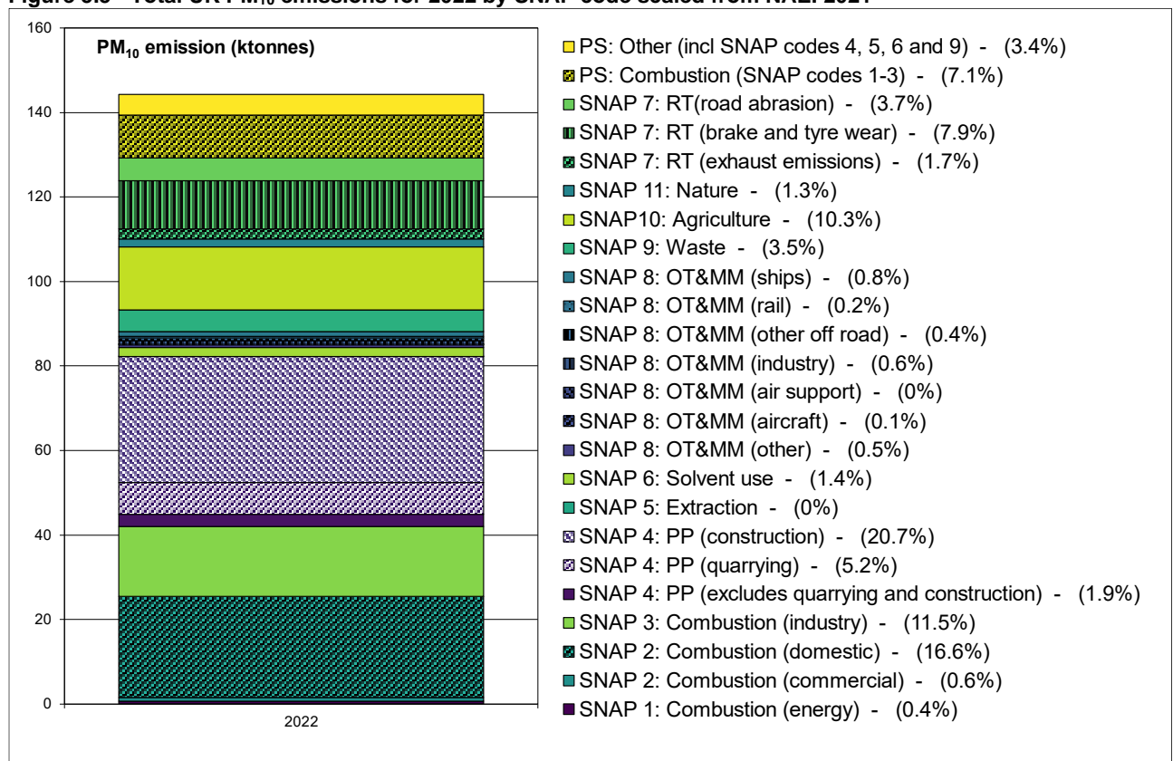
Figure 5.5 - Total UK PM 10 emissions for 2022 by SNAP code scaled from NAEI 2021
