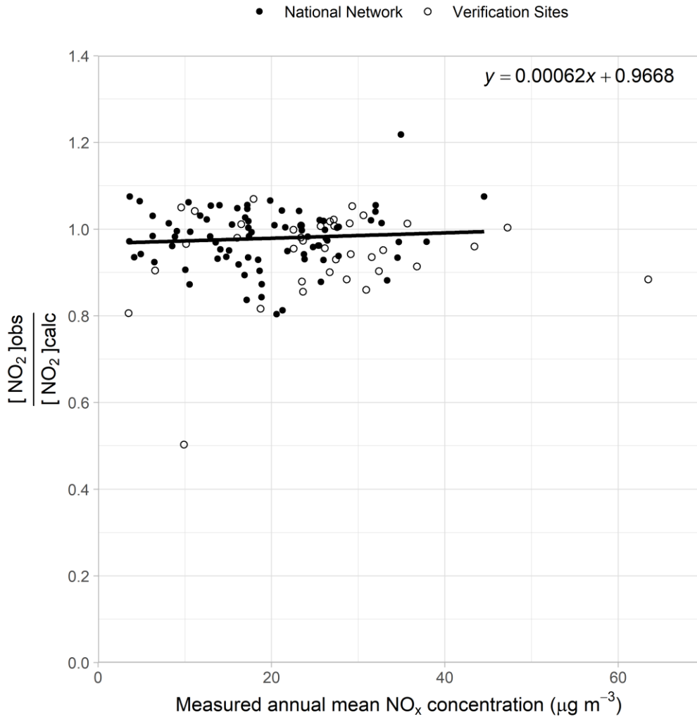
Figure 3.12 - Background NO 2 calibration curve (NB verification sites are shown for reference here, but were not used in calculating the calibration), 2022
