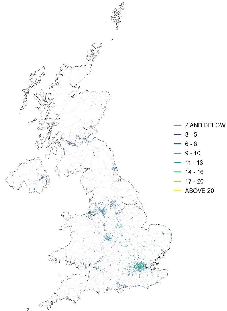
Figure 6.2 - Urban major roads, annual mean roadside PM 2.5 concentration, 2022 ( \mu\text{g m}^{-3} , gravimetric)
