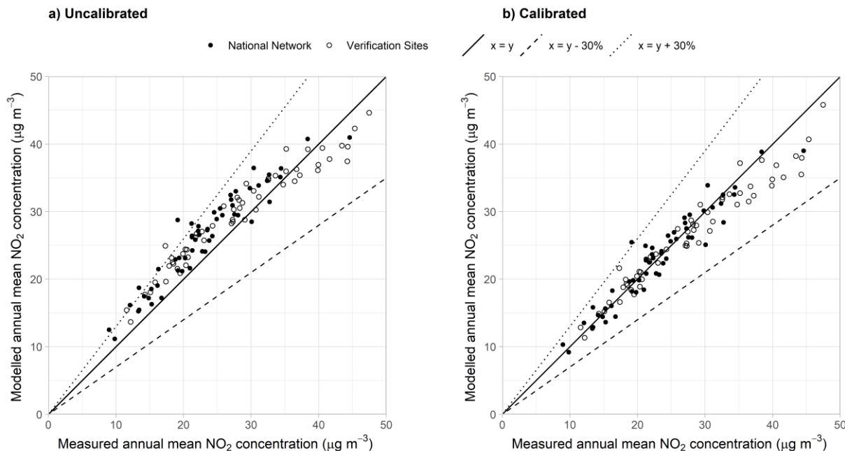
Figure 3.15 - Verification of roadside relationship at roadside locations in 2022
