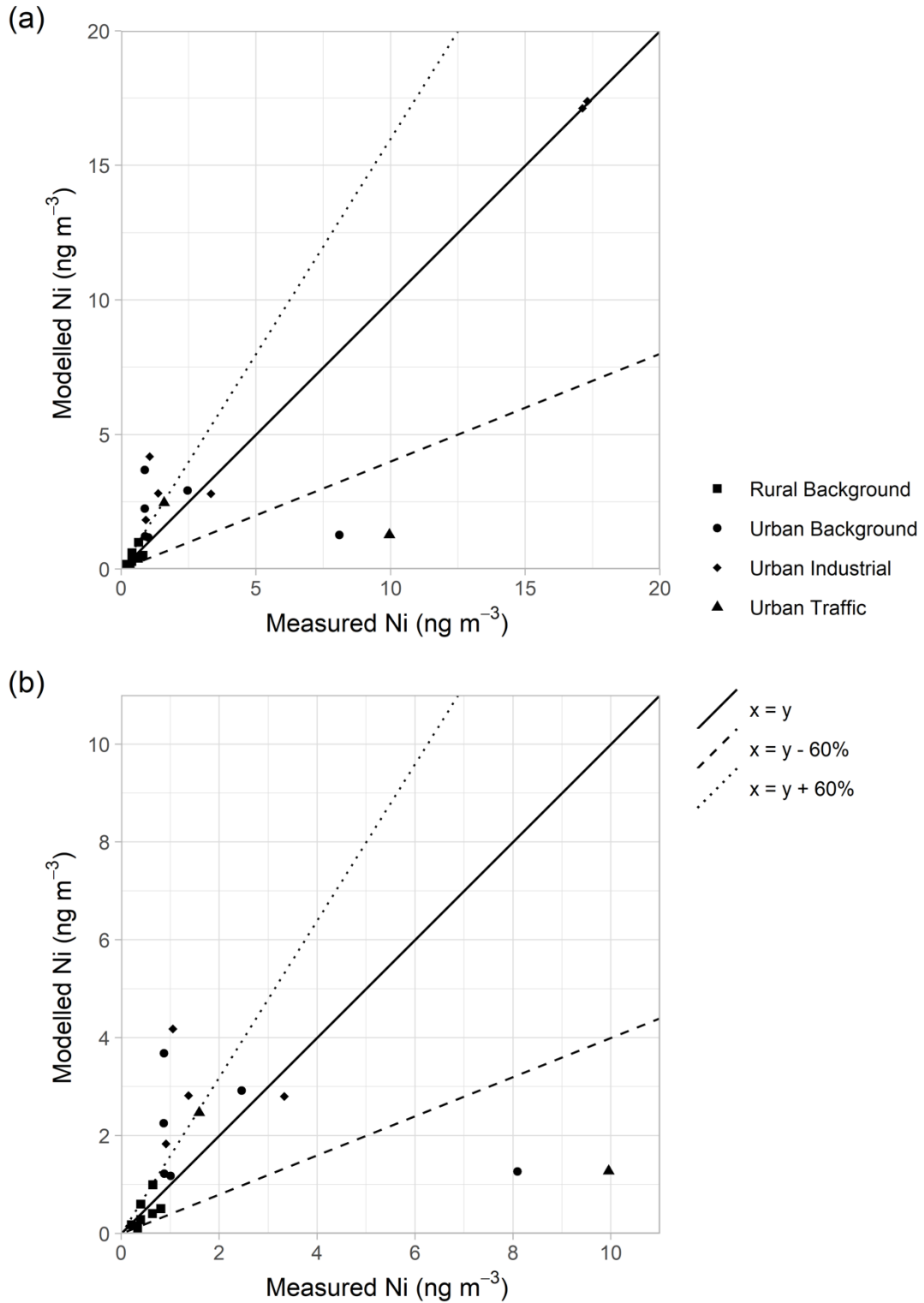
Figure 10.14 - Verification of annual mean Ni across all sites: (a) full scale showing all sites; (b) expanded scale where the results from Tawe Terrace and Sheffield Tinsley are off scale.
