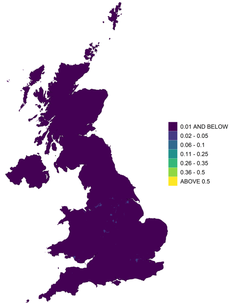
Figure 10.5 - Annual mean background Pb concentration, 2022 ( \mu\text{g m}^{-3} )
