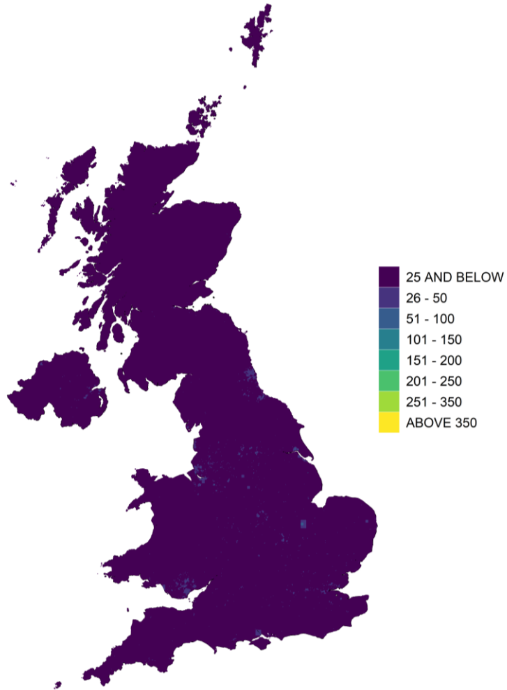
Figure 4.4 - 99.73 percentile of 1-hour mean SO 2 concentration, 2022 ( \mu\text{g m}^{-3} )
