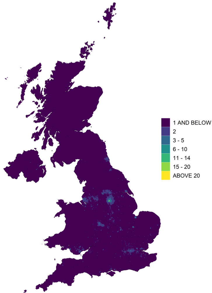
Figure 10.4 - Annual mean background Ni concentration, 2022 ( \text{ng m}^{-3} )
