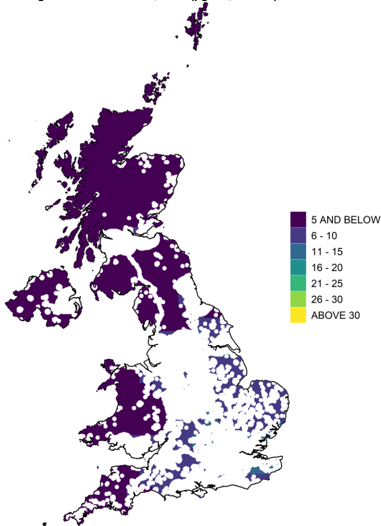
Figure 3.3 - Annual mean map of NO x concentrations for comparison with the NO x vegetation critical level, 2022 ( \mu\text{g m}^{-3} , as NO 2 )
