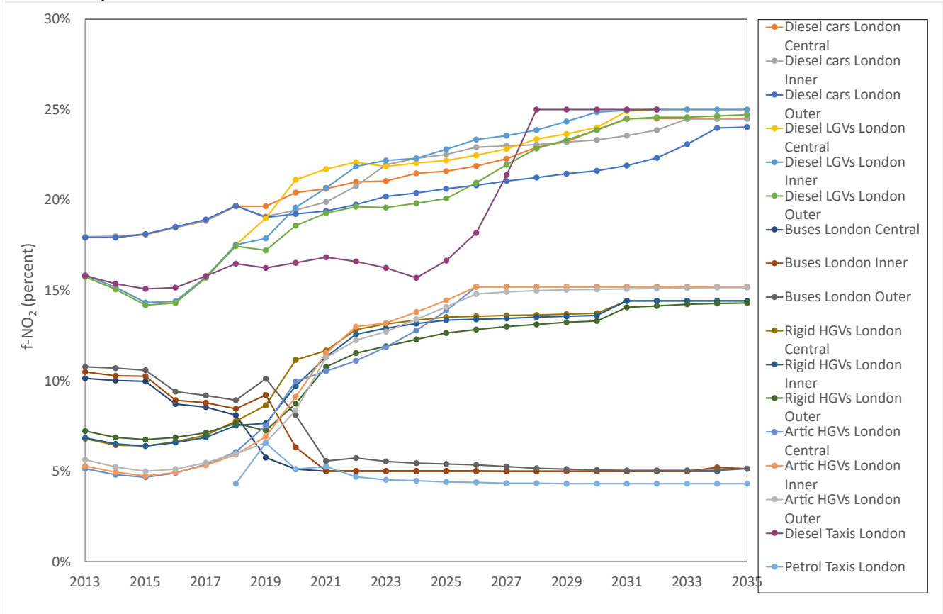
Figure 3.10 - Fleet average f -NO 2 projections by vehicle type for a) London and b) rest of the UK from NAEI
