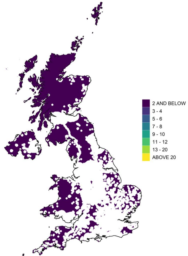
Figure 4.3 - Winter mean SO 2 concentration, 2021-2022 (µg m -3 ) in vegetation areas
