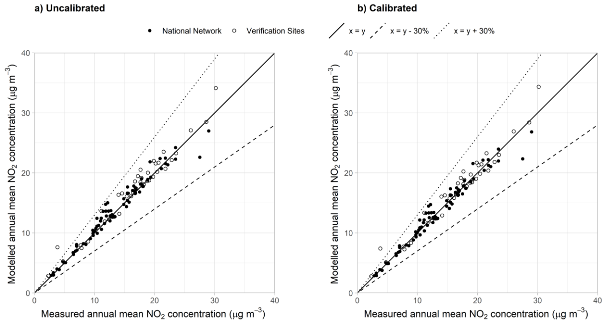
Figure 3.13 - Verification of background relationship at background locations in 2022
