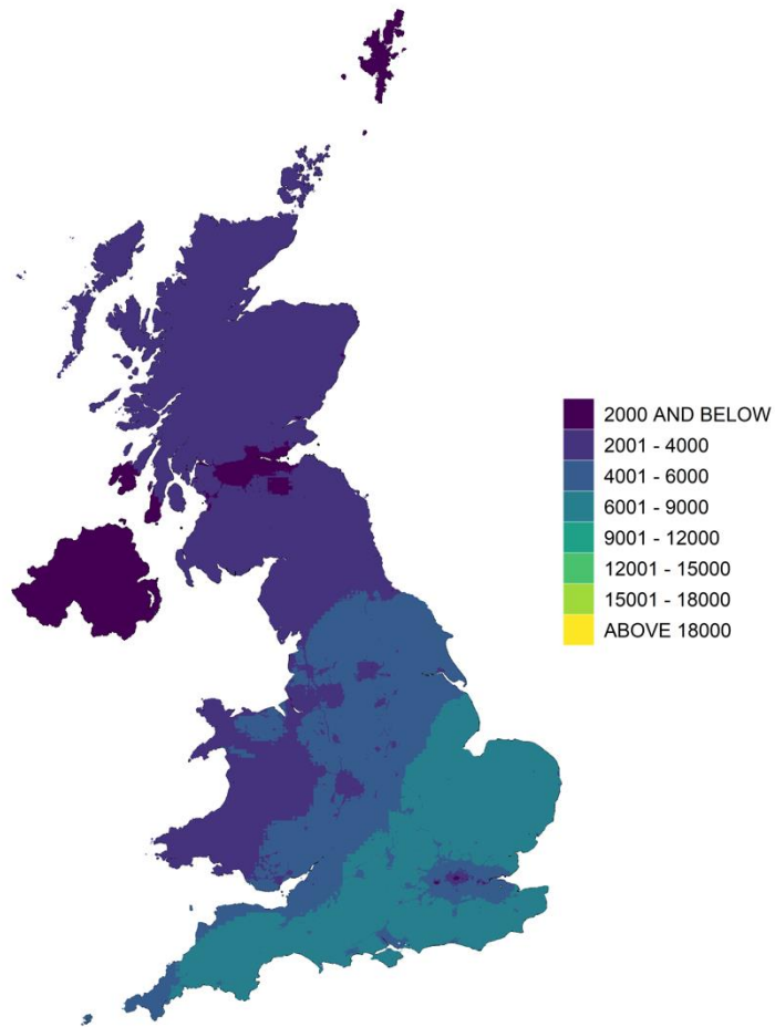
Figure 9.8 - Estimated AOT40 vegetation metric, 2022 ( \mu\text{g m}^{-3} hours)
