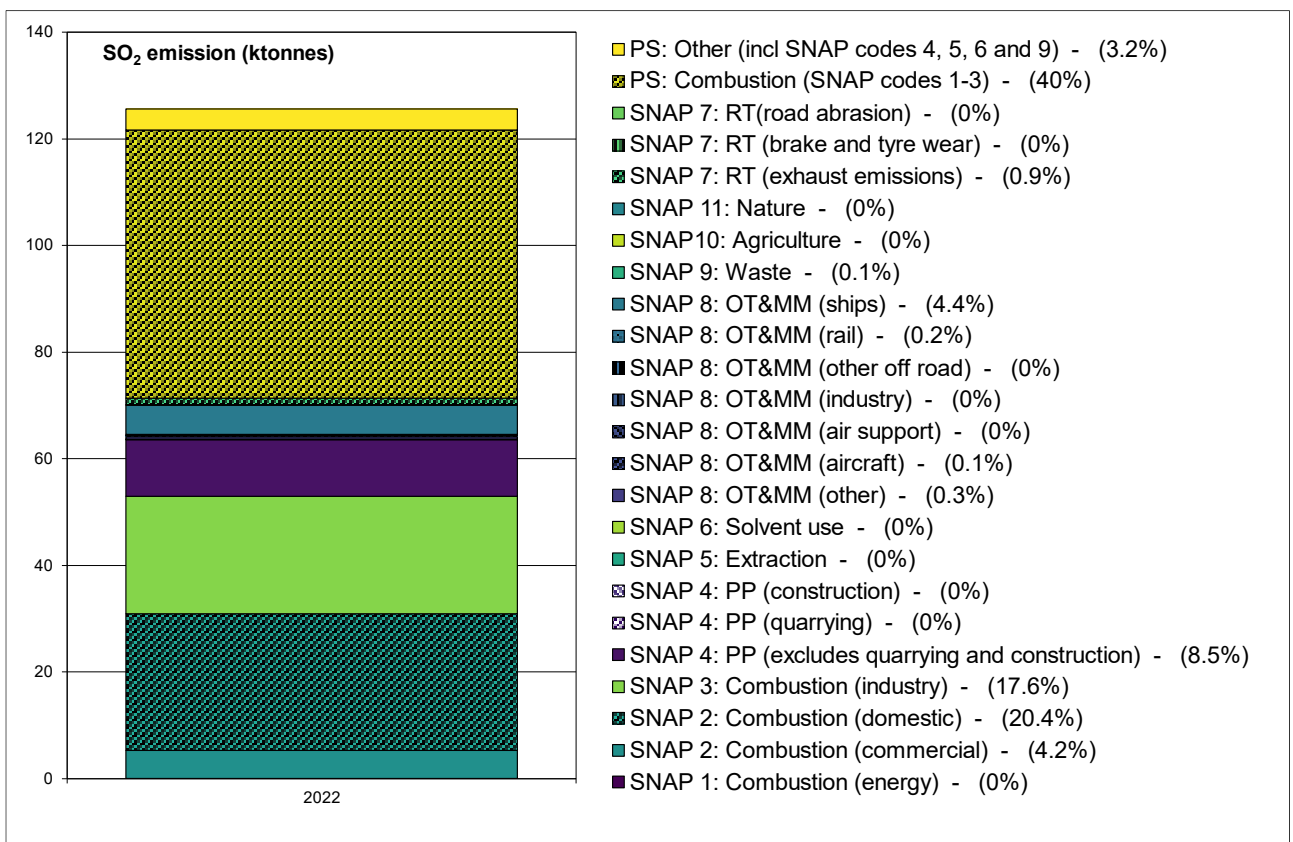
Figure 4.6 - Total UK SO 2 emissions for 2022 by SNAP code scaled from NAEI 2021
