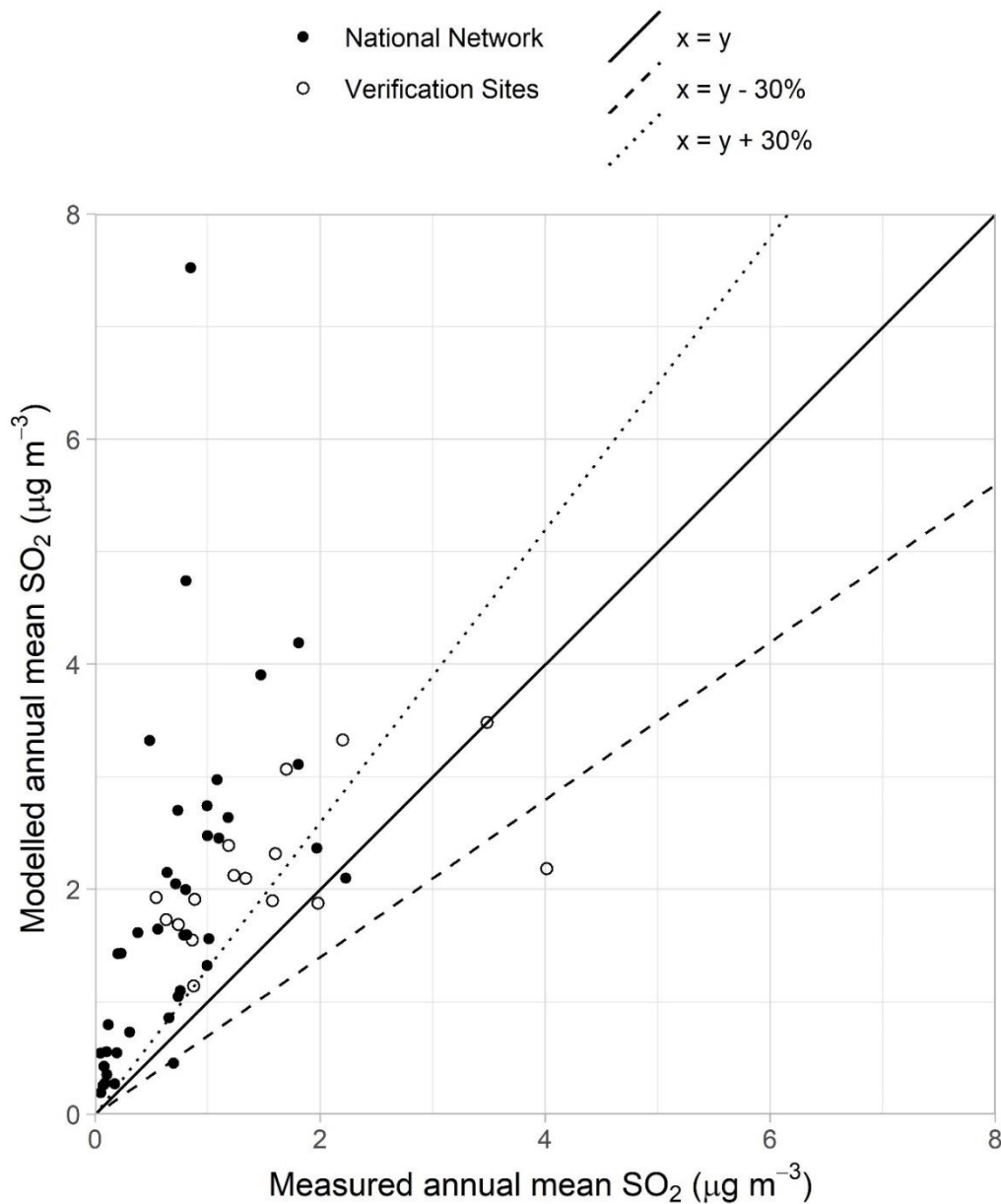
Figure 4.9 – Verification plot for 2022 annual mean SO 2 concentrations
