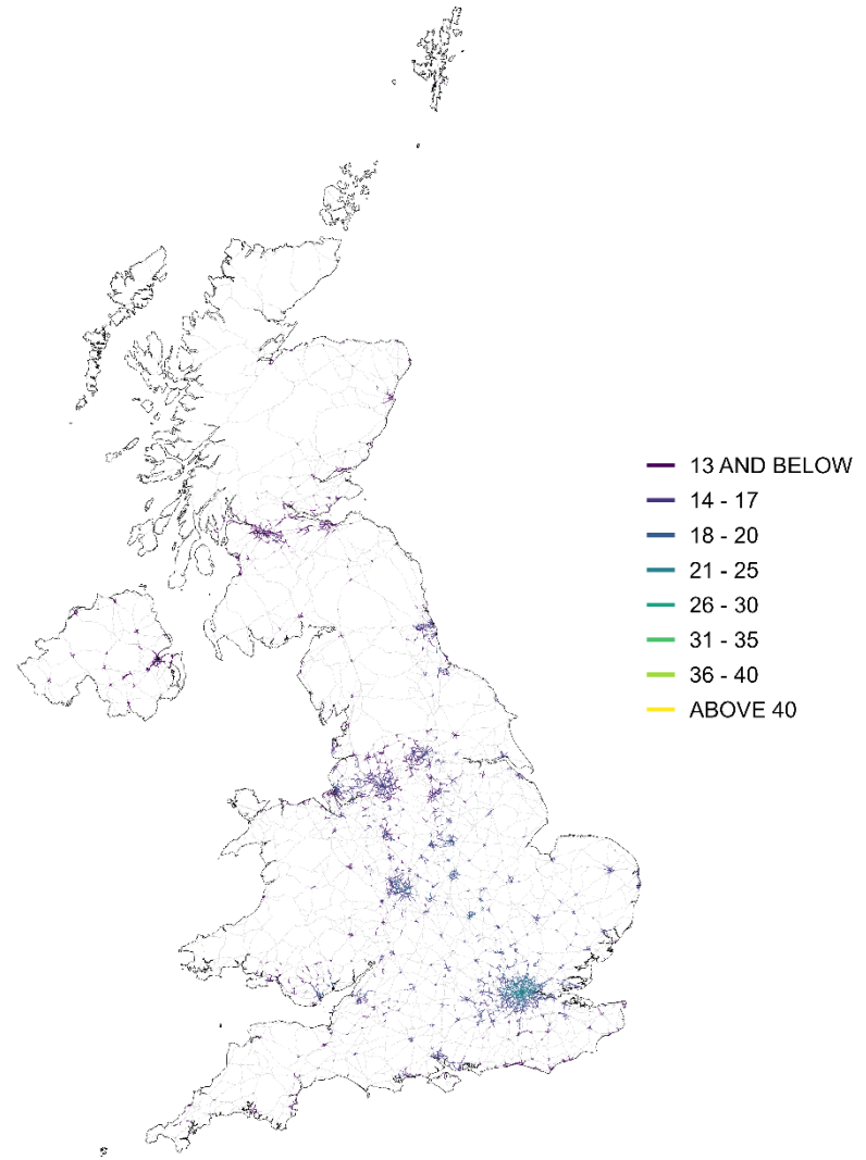
Figure 5.2 - Urban major roads, annual mean roadside PM 10 concentration, 2022 ( \mu\text{g m}^{-3} , gravimetric)
