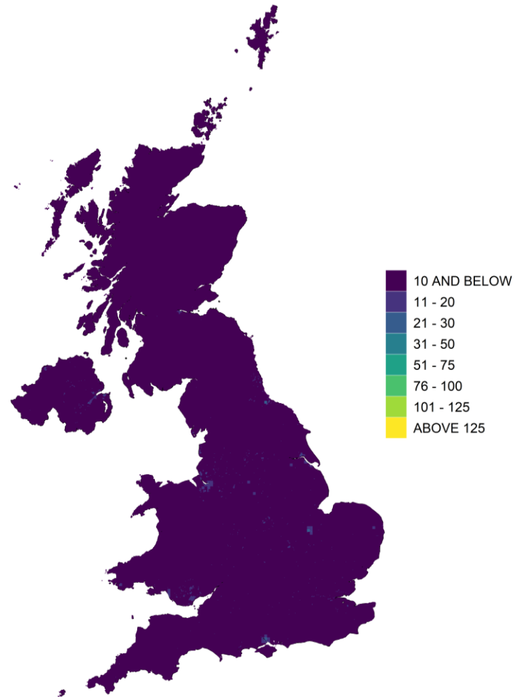
Figure 4.5 - 99.18 percentile of 24-hour mean SO 2 concentration, 2022 ( \mu\text{g m}^{-3} )
