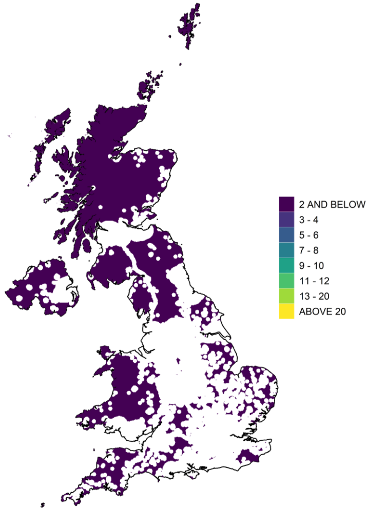
Figure 4.2 - Annual mean SO 2 concentration, 2022 (µg m -3 ) in vegetation areas
