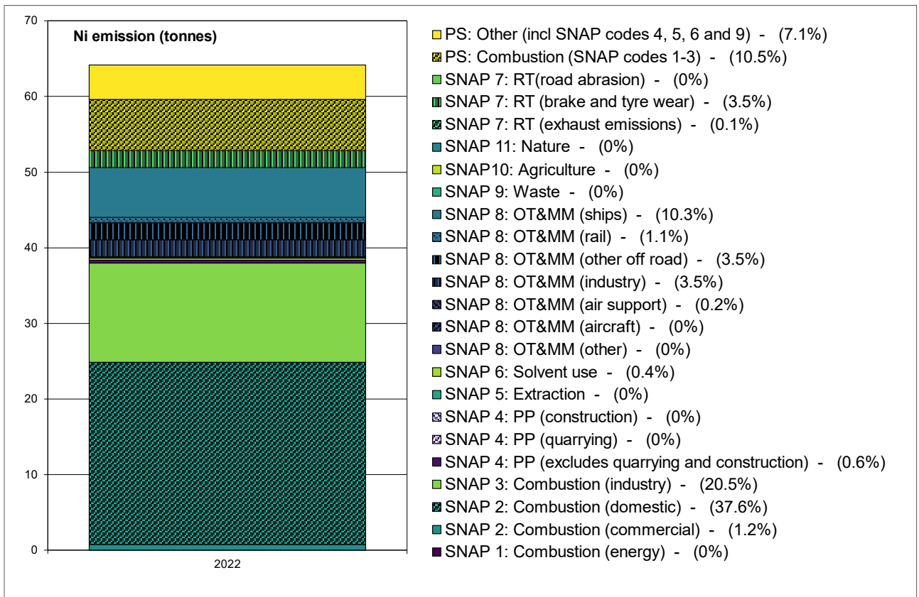
Figure 10.8 - Total UK Ni emissions for 2022 by SNAP code scaled from NAEI 2021
