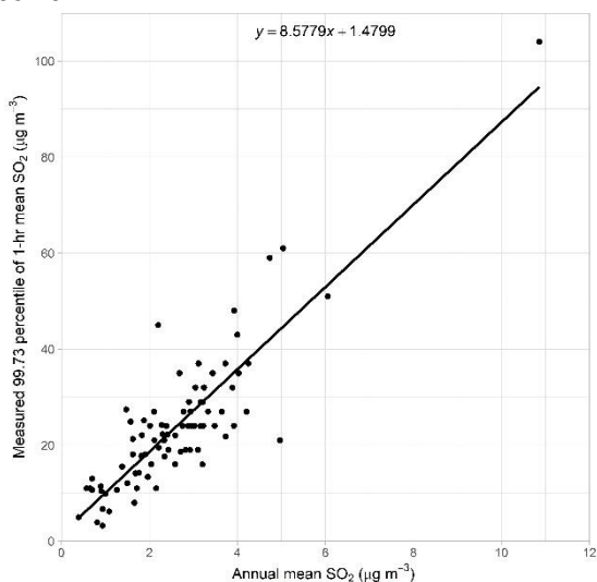
Figure 4.7 - Relationship between mean concentration and 99.73 percentile of 1 hour concentrations at sampling sites in Northern Ireland, 2008-2022
