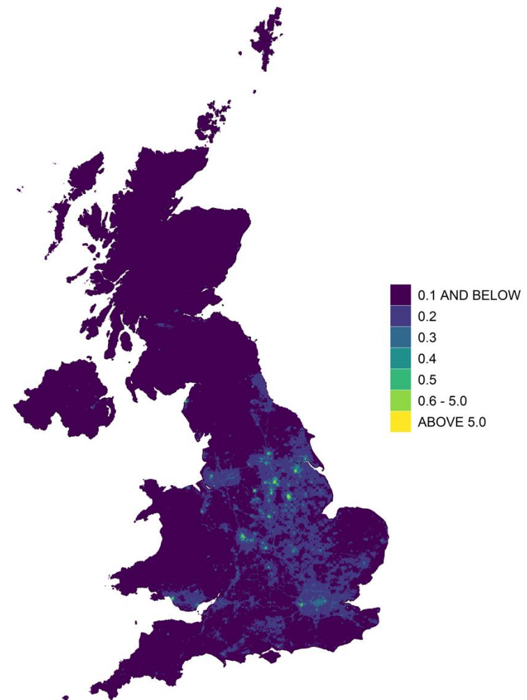
Figure 10.3 - Annual mean background Cd concentration, 2022 (ng m -3 )
