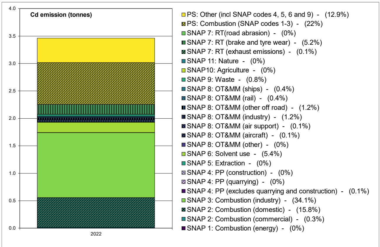
Figure 10.7 - Total UK Cd emissions for 2022 by SNAP code scaled from NAEI 2021
