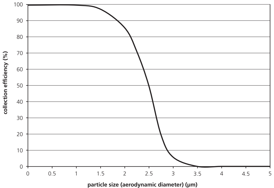
Figure 2.1: Indicative size-selection curve for a PM 2.5 inlet.
