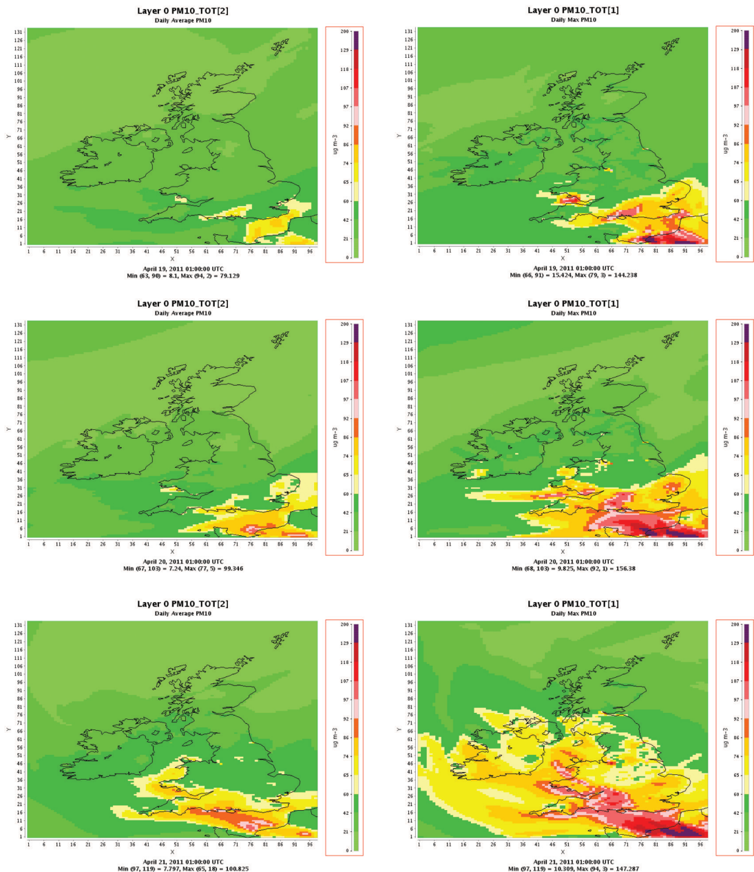
Daily Average PM 10
