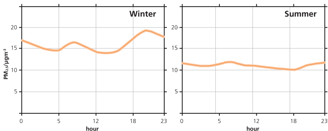
Figure 3.2: Variation of PM 2.5 concentrations ( \mu\text{g m}^{-3} ) at urban background sites by hour of the day in 2010 at southern UK sites ( n=10 ) in winter and summer. The shading represents the 95% confidence interval of the mean.
