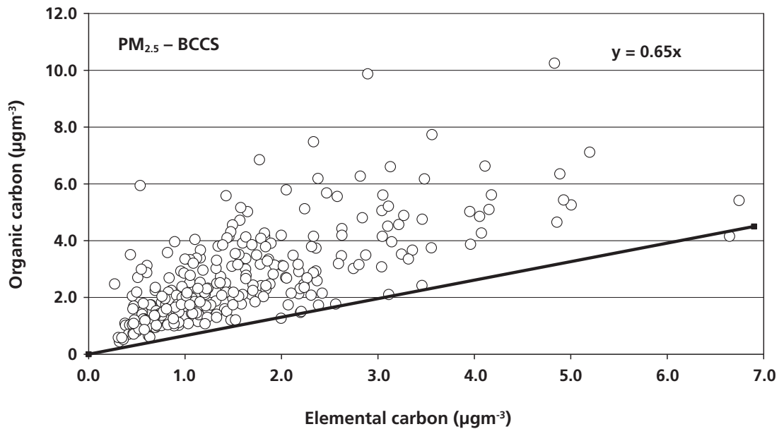
Figure 4.8: Relationship of organic carbon to elemental carbon in the PM 2.5 fraction at the Birmingham City Centre site (BCCS) (urban centre) showing the minimum ratio line.
