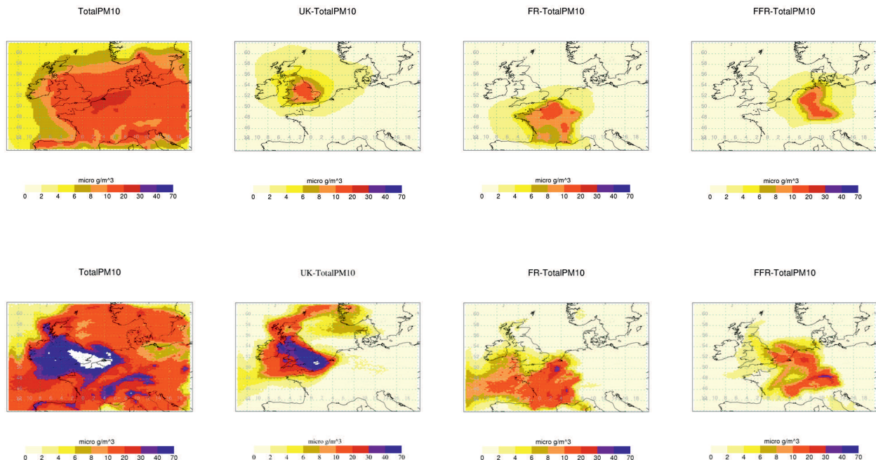
Figure A2.4.2: NAME-modelled total \text{PM}_{10} (sulphate, nitrate, ammonium, secondary organic aerosol and primary \text{PM}_{10} ). Top row from left, annual average total \text{PM}_{10} concentration for 2003 resulting from: emissions from all countries within the model domain, UK emissions, French emissions (FR) and western German emissions (FFR). Bottom row from left, daily average total \text{PM}_{10} on 8 August 2003 resulting from: emissions from all countries within the model domain, UK emissions, French emissions (FR) and western German emissions (FFR). The white areas indicate concentrations greater than 70 \mu\text{g m}^{-3} .
