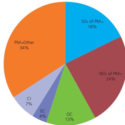
Figure A2.3.2: Average observed and CMAQ PM 10 components for 2008 at Harwell and London North Kensington.
