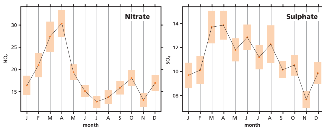
Figure 3.18: Variation of nitrate and sulphate concentrations ( \mu\text{g m}^{-3} ) by month of the year (data from 30 AGANet sites, 1999-2009). The shading represents the 95% confidence interval of the mean. Note different scales.
