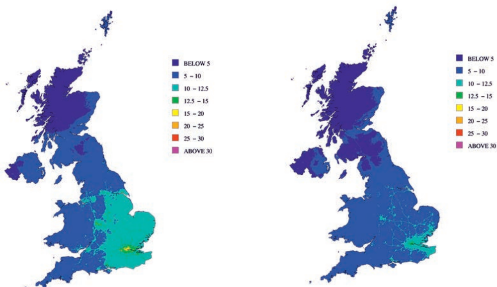
Figure 5.1: Concentrations of total annual mean PM 2.5 as calculated by the PCM model ( \mu\text{g m}^{-3} ) for 2009 (left) and 2020 (right).
