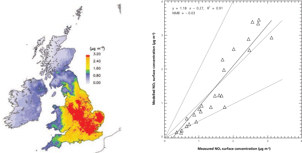
Figure A2.7.1: Left: Nitrate concentrations in air modelled with FRAME for the year 2008; Right: Comparison of modelled nitrate concentrations in air with measurements from AGANet.
