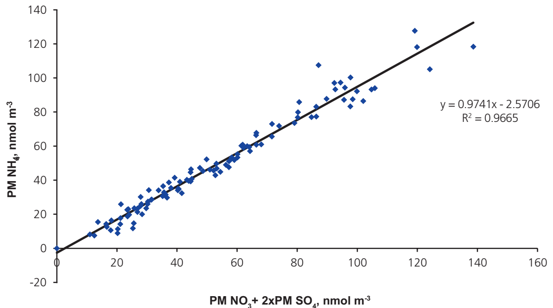
Figure 3.19: Ammonium concentrations versus nitrate plus two times sulphate concentrations in nmol m -3 (data from 30 AGANet sites, 1999-2009).
