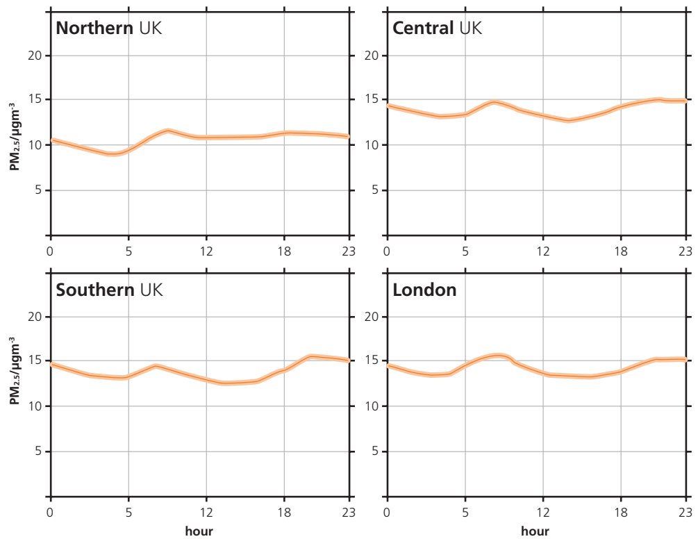
Figure 3.1a: Variation of PM 2.5 concentrations ( \mu\text{g m}^{-3} ) at urban background sites by hour of the day in 2010 at sites in northern UK (n=6), central UK (n=17), southern UK (n=10) and London (n=8). The shading represents the 95% confidence interval of the mean.
