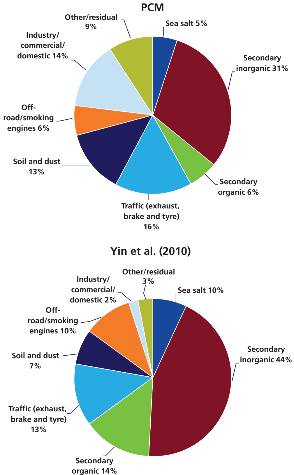
Figure 4.11: Comparison of PCM model outputs for 2009 (top) with CMB model output for 2007-2008 (bottom) (Yin et al. , 2010) for source apportionment of PM 2.5 in Birmingham.
