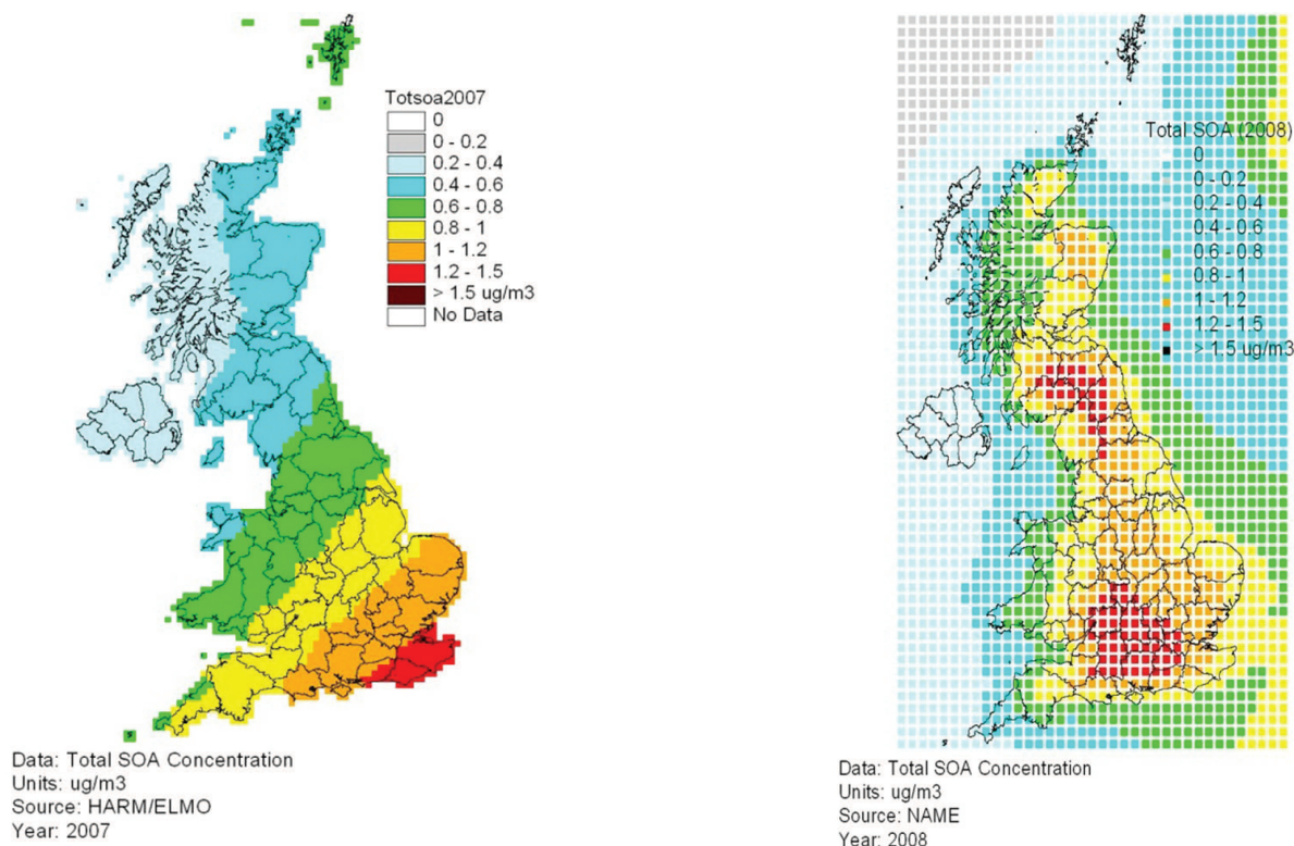
Figure 5.9: Comparison of total SOA concentrations from HARM/ELMO model (left) and the NAME model (right).
