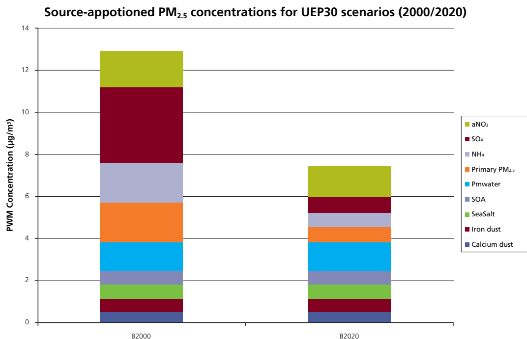
Figure A2.9.1: Breakdown of PM 2.5 concentrations by component for 2000 and 2020.
