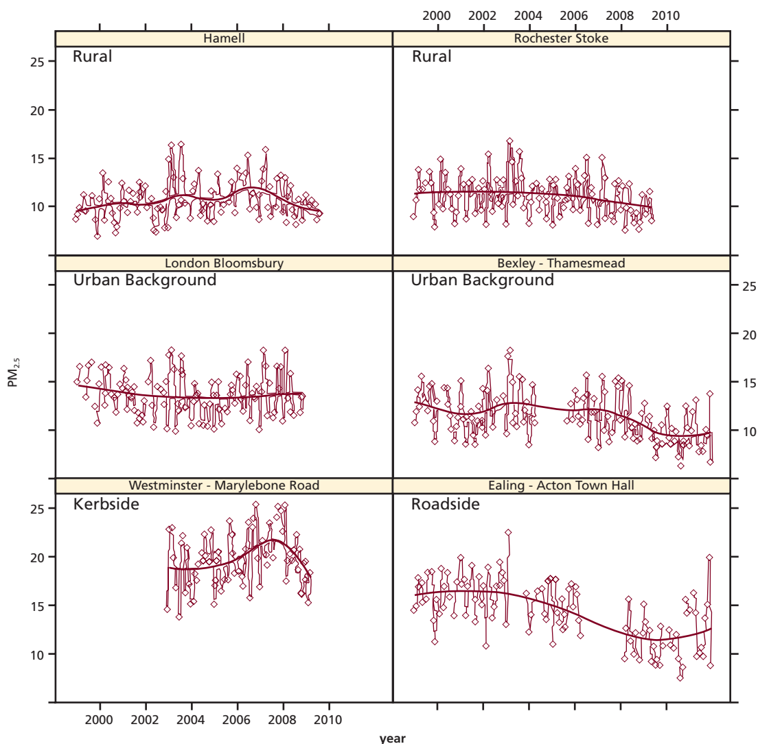
Figure 3.6: PM 2.5 concentrations (TEOM \mu\text{g m}^{-3} unadjusted) at rural, urban background and roadside/kerbside sites in southern England. A smoothed trendline has been fitted with the shading representing the 95% confidence interval.
