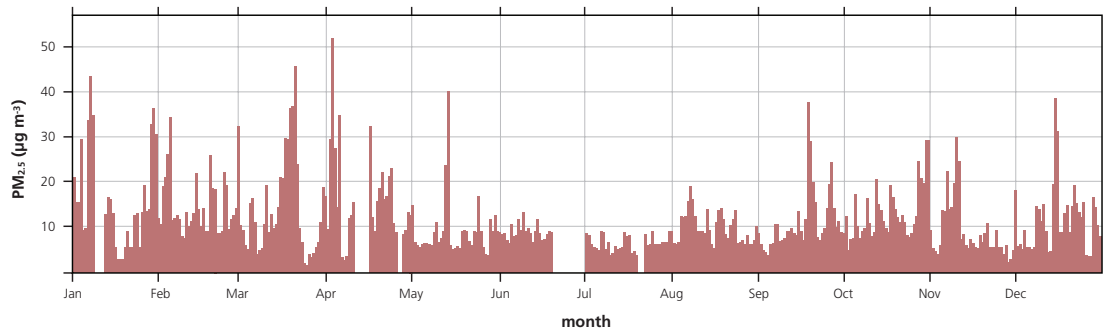
Figure 3.12a: Daily mean PM 2.5 concentration at the London Bexley Slade Green site for 2009.
