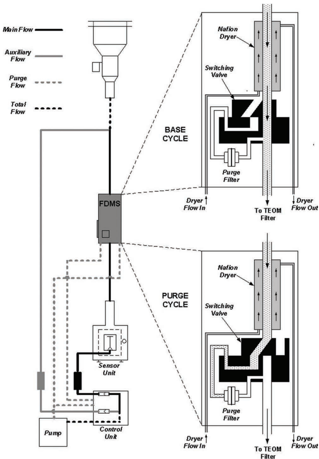
Figure 2.3: FDMS design (diagram courtesy of Dr David Green, King's College London).
