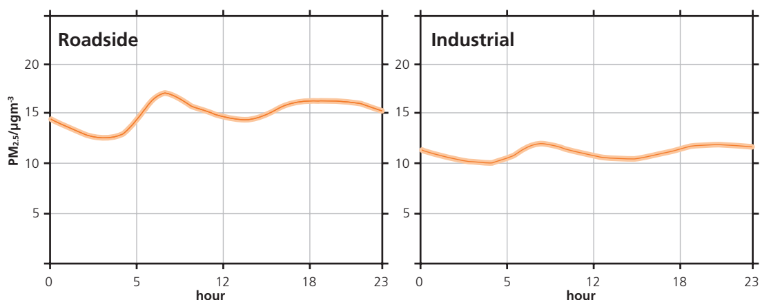
Figure 3.3: Variation of PM 2.5 concentrations ( \mu\text{g m}^{-3} ) by hour of the day at roadside ( n=9 ) and industrial sites ( n=4 ) in 2010. The shading represents the 95% confidence interval of the mean.
