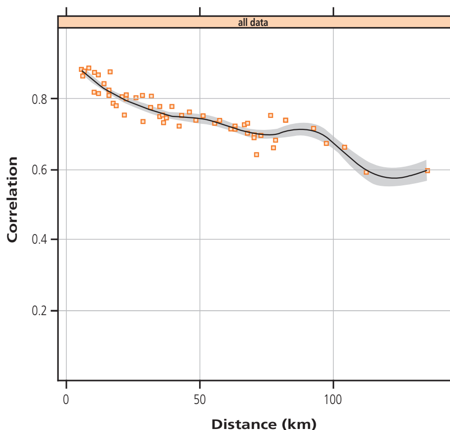
Figure 3.10: Correlation coefficients of hourly mean PM 2.5 concentrations ( \mu\text{g m}^{-3} ) at 11 urban background sites in the Thames Valley area of southern England as a function of distance between the sites (Laxen et al. , 2010). The shading represents 95% confidence interval.
