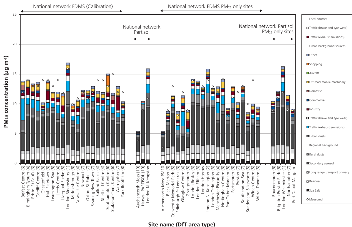
Figure 5.10: Source apportionment for background sites in 2009 from PCM model.
