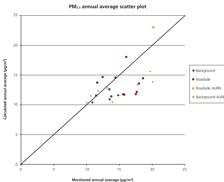
Figure A2.10.1: Scatter plot of calculated and monitored annual average concentrations of PM 2.5 for 2008.
