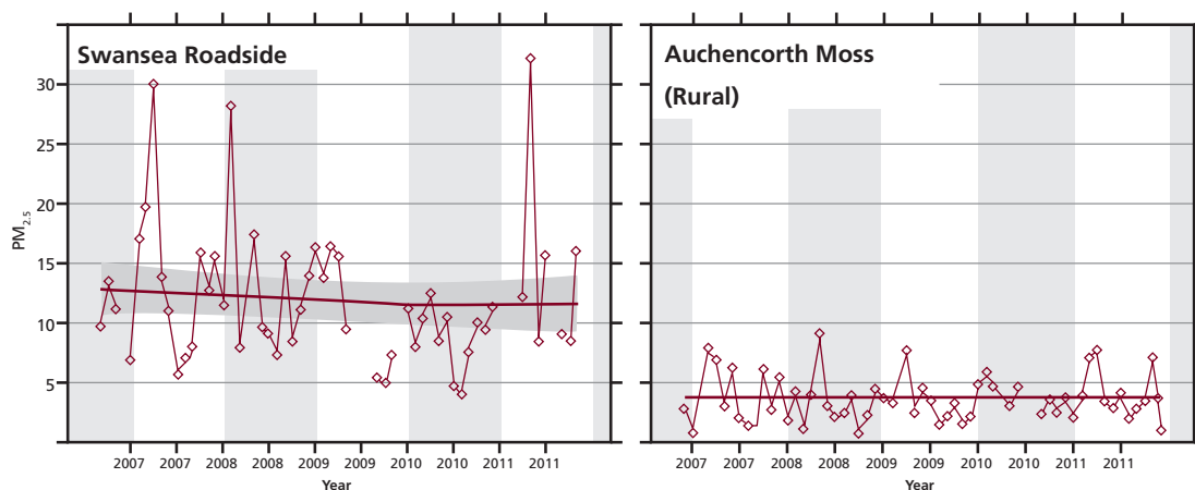
Figure 3.7: PM 2.5 concentrations (FDMS, µg m -3 ), 2006-2011, at Swansea roadside site in Wales and Auchencorth Moss rural site in Scotland. A smoothed trendline has been fitted with the shading representing the 95% confidence interval.
