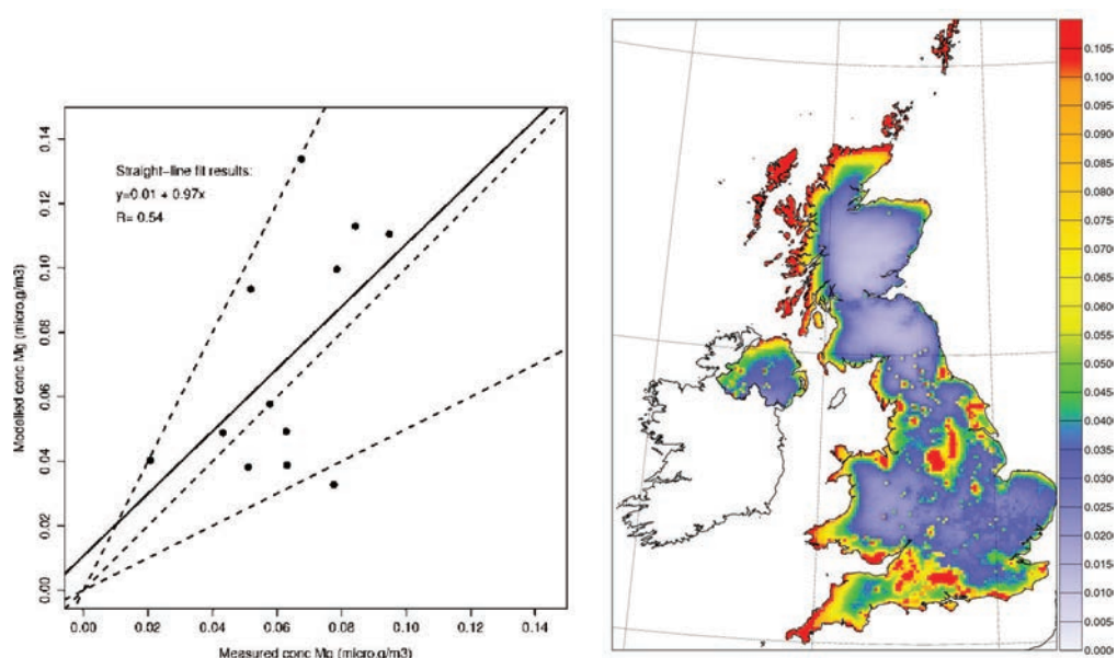
Figure A2.7.2: Left: Comparison of modelled \text{Mg}^{2+} concentrations in air with measurements from AGANet; Right: \text{Ca}^{2+} concentrations in air modelled with FRAME (all \mu\text{g m}^{-3} ).
