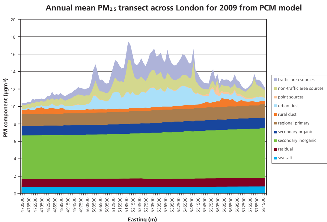
Figure 5.6: Transect through the PM 2.5 concentration distribution in London, showing a number of individual PM components from Henley-on-Thames in the west to Southend-on-Sea in the east (derived from PCM model). The transect is coincident with but extends further than that shown in Figure 5.5.
