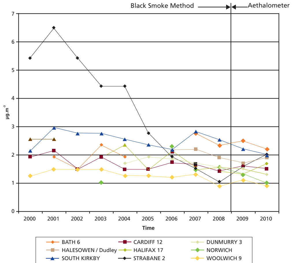
Figure 3.22: Trends in black carbon and converted black smoke concentrations 2000 to 2010.
