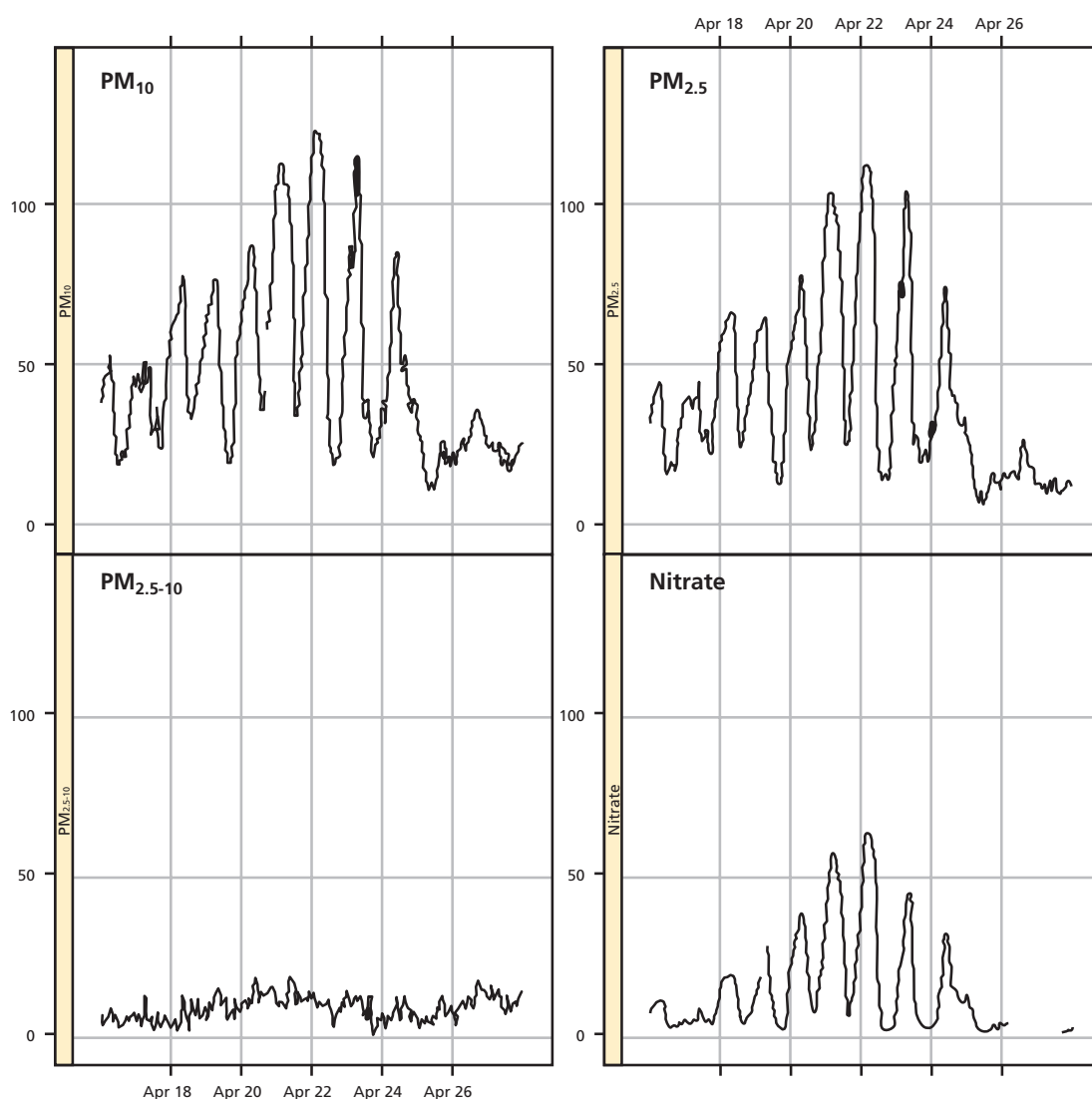
Figure 3.15: PM 10 , PM 2.5 , PM 2.5-10 and nitrate concentrations ( \mu\text{g m}^{-3} ) over 15 days in April 2011 at London North Kensington.
