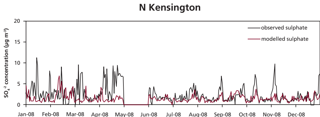
Figure A2.3.5: Time series of measures and CMAQ daily SO 4 2- at London North Kensington, 2008.
