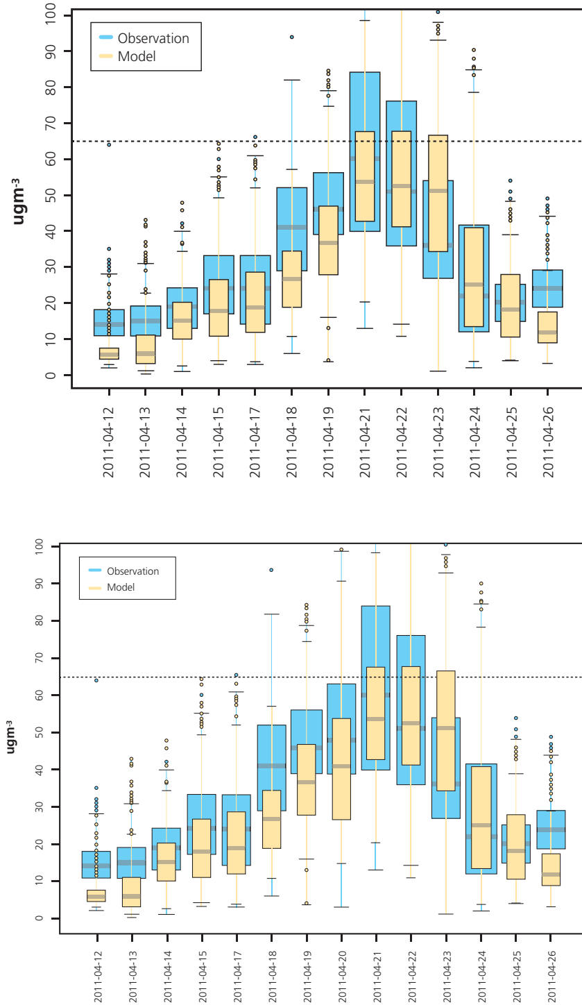
Figure A2.1.2: Evaluation of CMAQ forecast with hourly PM 10 provisional data from 16 AURN urban background sites, 12-26 April 2011.
