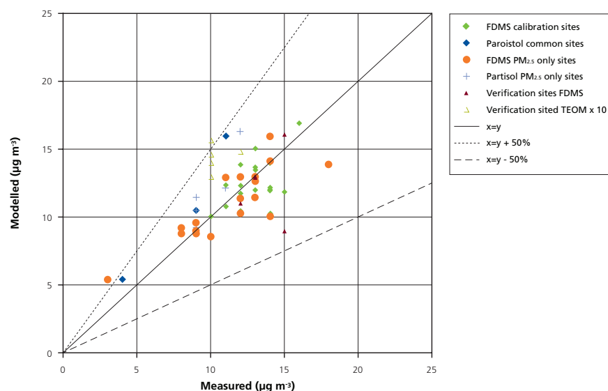
Figure A2.8.1: Verification plot for the PCM model estimates of PM 2.5 for background sites in 2009.
