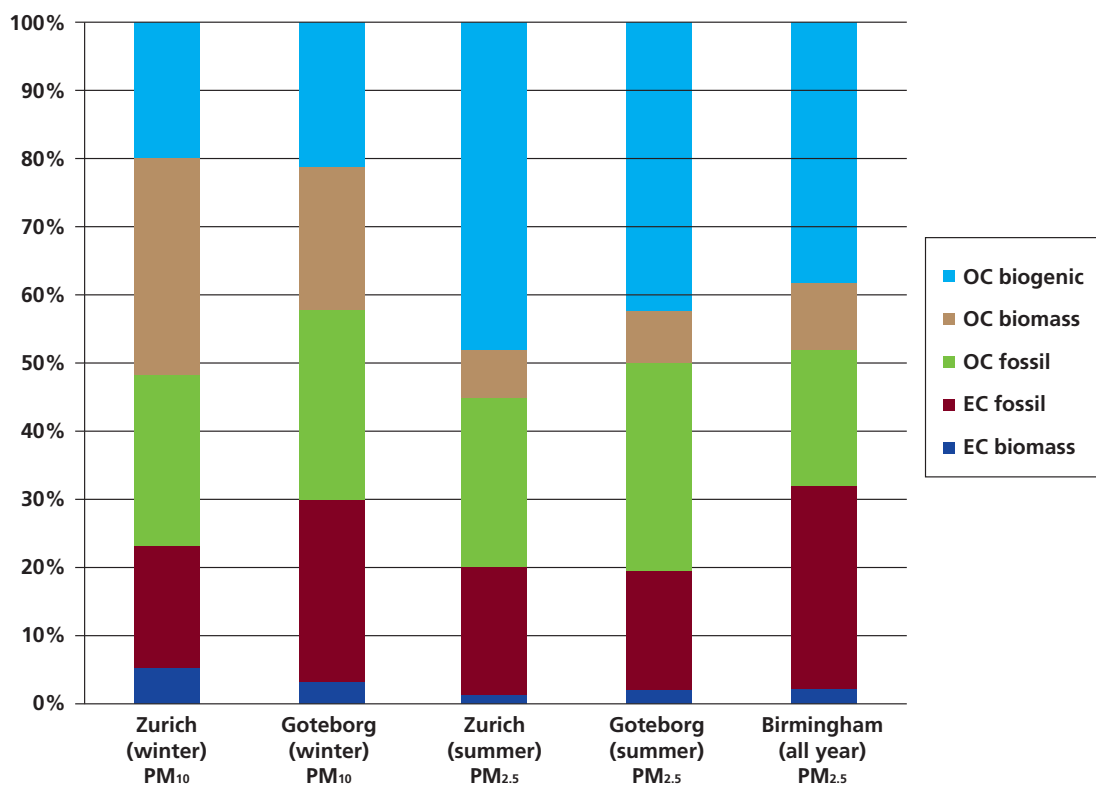
Figure 4.12: Mean five-source apportionment of Total Carbon in Birmingham (Heal et al. , 2011) compared with similar work from Zurich (Szidat et al. , 2006) and Göteborg (Szidat et al. , 2009). OC biomass is POC from combustion of biofuels/biomass, OC fossil is both fossil-derived POC and any SOC from fossil-derived VOC, and OC biogenic is SOC formed from BVOC oxidation together with any other contemporary OC material not explicitly accounted for elsewhere, for example spores, vegetative detritus, tyre rubber, etc.
