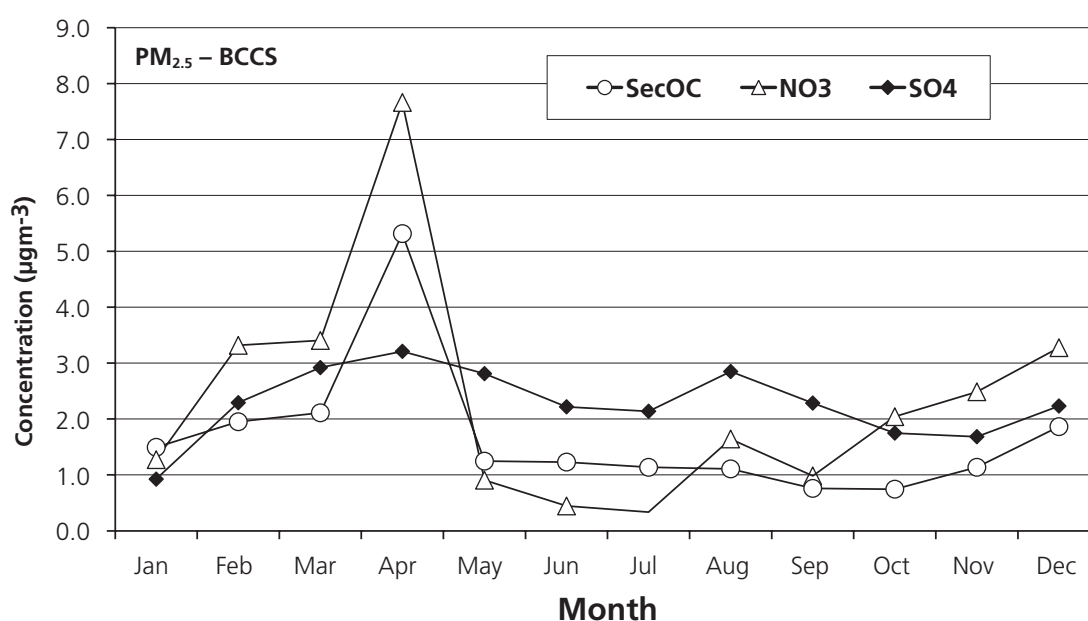
Figure 4.9: Monthly mean concentrations of secondary OC, nitrate and sulphate in PM 2.5 at the Birmingham City Centre site (BCSS) (urban centre) (Yin et al. , 2010).
