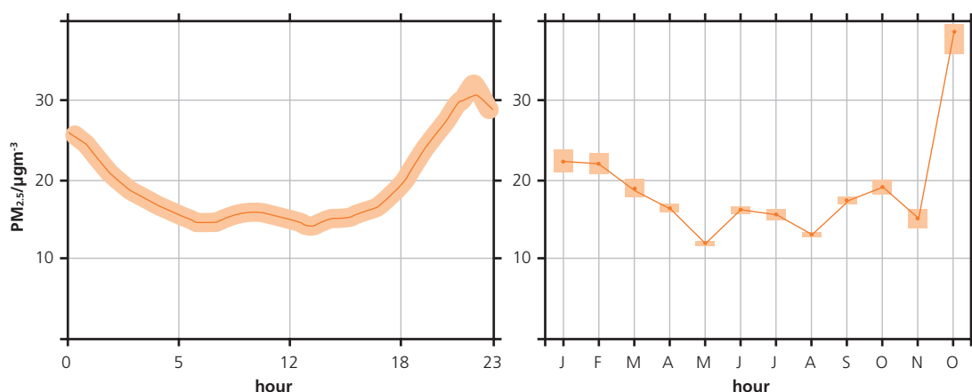
Figure 3.4: Variation of PM 2.5 concentrations ( \mu\text{g m}^{-3} ) by hour of the day and month of the year at the Lisburn site in Northern Ireland in 2010. The shading represents the 95% confidence interval of the mean. Note the different scale to the other figures.
