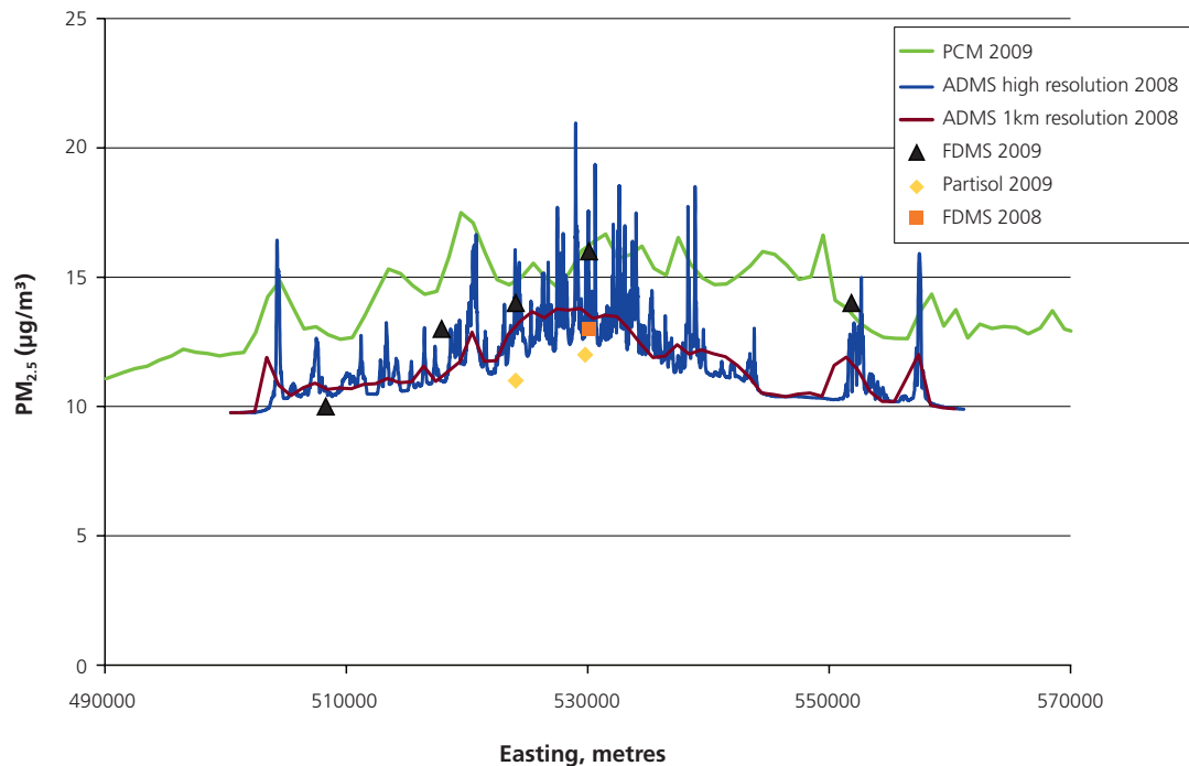
Figure 5.5: Annual mean PM 2.5 concentrations predicted using the ADMS-Urban (2008) and PCM (2009) models together with observations from FDMS and Partisol instruments (mainly 2009) through Central London. The ADMS-Urban predictions are shown at 10 m x 10 m resolution (blue line) and at 1 km x 1 km resolution (red line).
