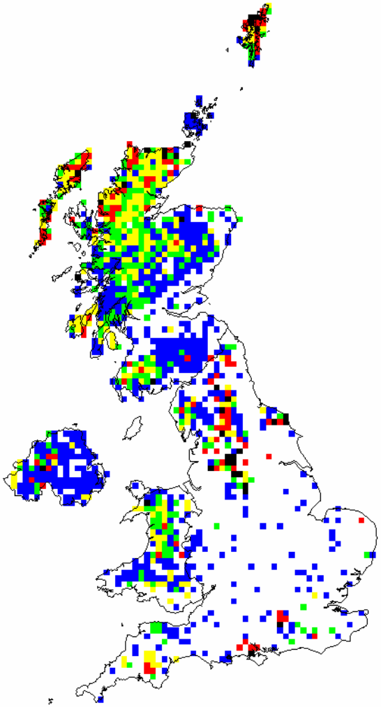
Maximum critical load of sulphur ( CL_{max} S )
