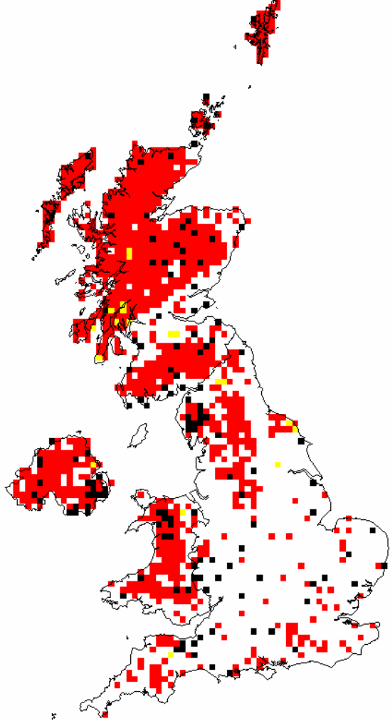
Minimum critical load of nitrogen ( CL_{min} N )
