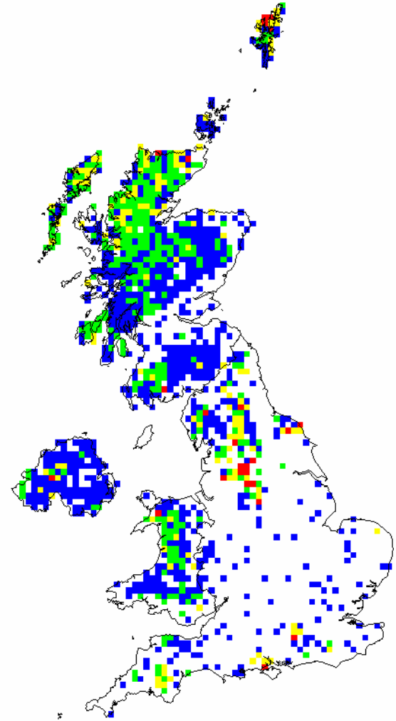
Maximum critical load of nitrogen ( CL_{max} N )
