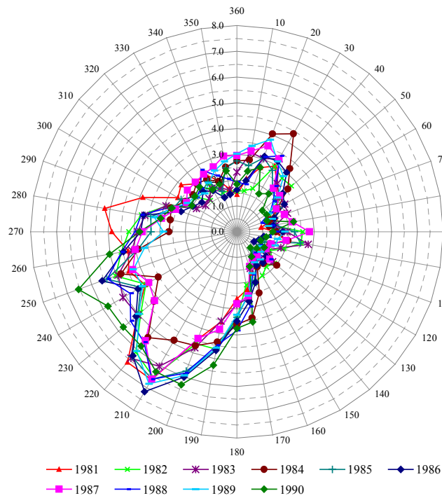
Figure 14 Rose plot showing the frequency, %, of wind directions, 1981-90
