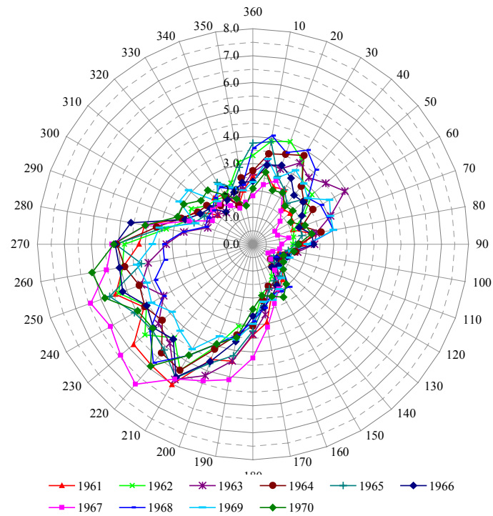
Figure 12 Rose plot showing the frequency, %, of wind directions, 1961-70
