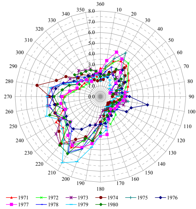
Figure 13 Rose plot showing the frequency, %, of wind directions, 1971-80
