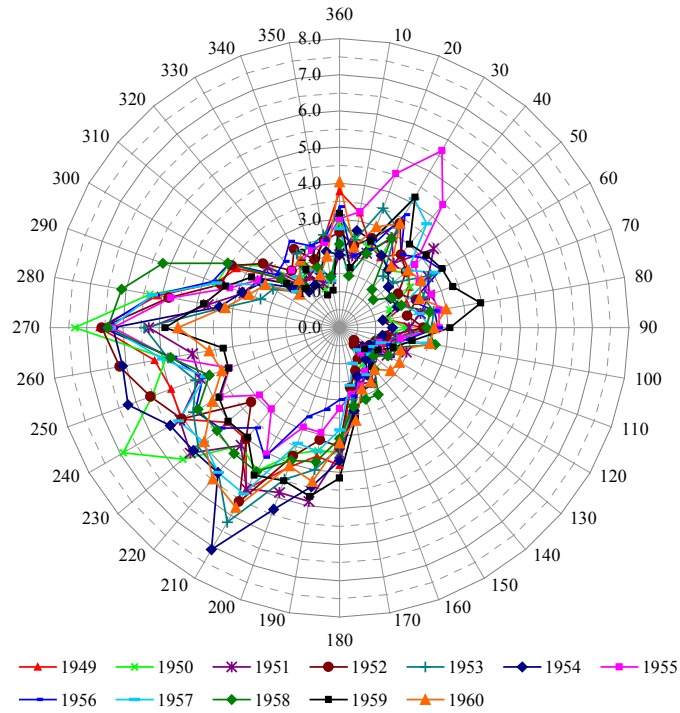
Figure 11 Rose plot showing the frequency, %, of wind directions, 1949-60
