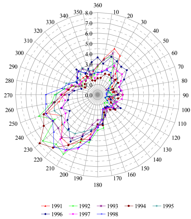
Figure 15 Rose plot showing the frequency, %, of wind directions, 1991-98
