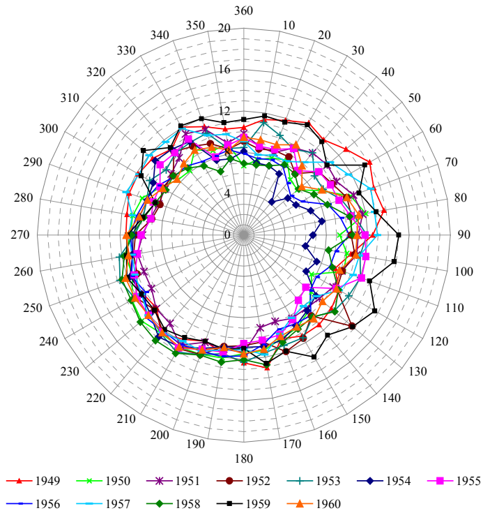
Figure 16 Rose plot showing the average temperature, °C, from each direction, 1949-60
