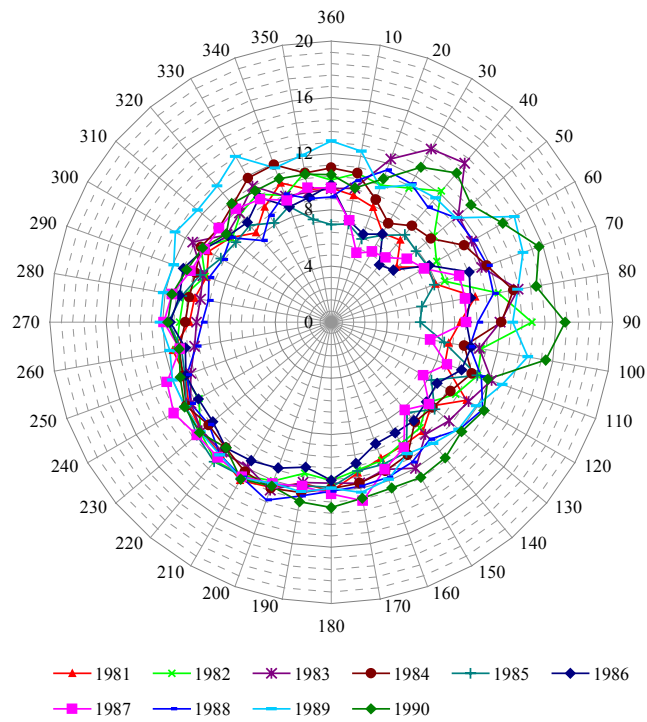
Figure 19 Rose plot showing the average temperature, °C, from each direction, 1981-90
