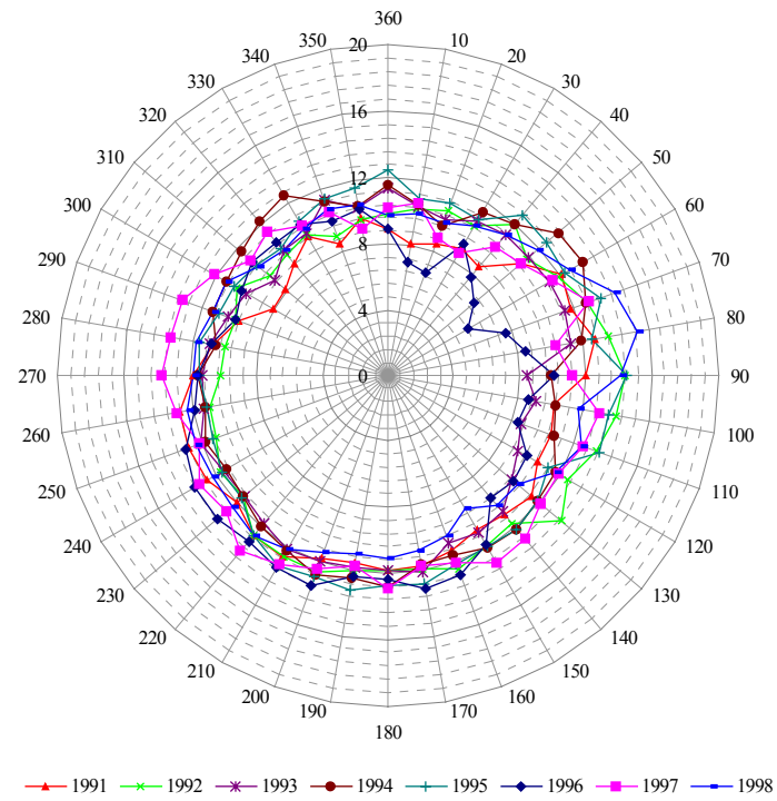
Figure 20 Rose plot showing the average temperature, °C, from each direction, 1991-98
