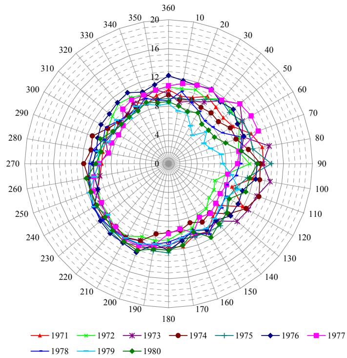
Figure 18 Rose plot showing the average temperature, °C, from each direction, 1971-80
