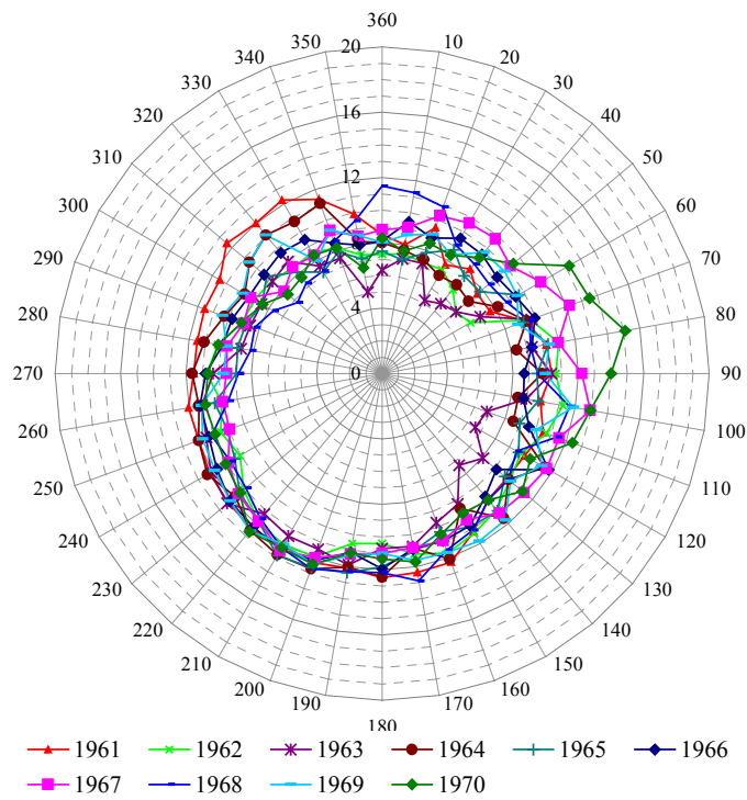
Figure 17 Rose plot showing the average temperature, °C, from each direction, 1961-70
