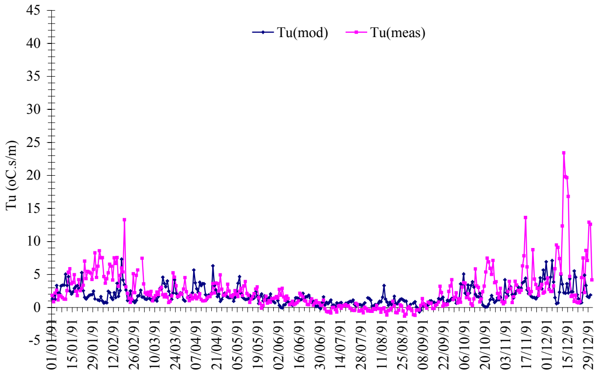
Figure 41 Results for the winter index Tu based on climate model 360 day year for 1991.
