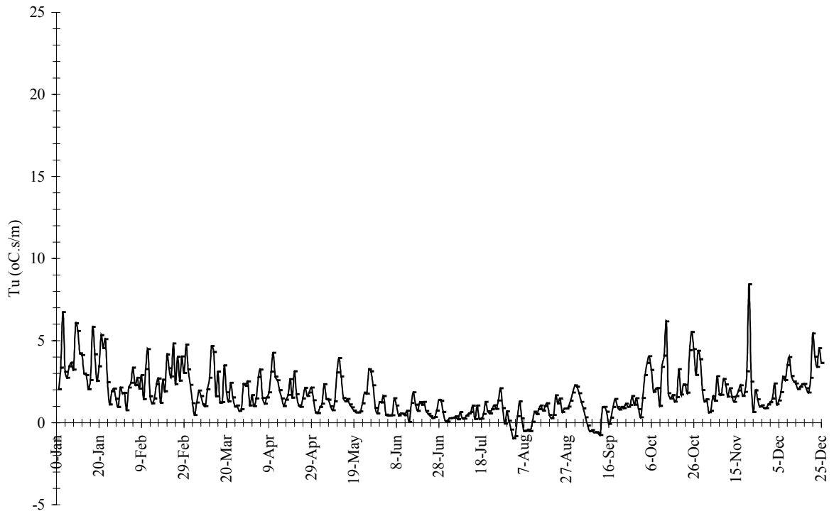
Figure 45 Results for the winter index Tu based on climate model 360 day year for 2020.
