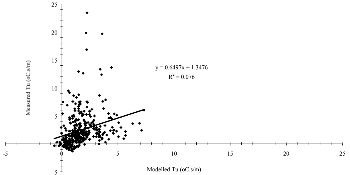
Figure 41 Results for the winter index Tu based on climate model 360 day year for 1991.
