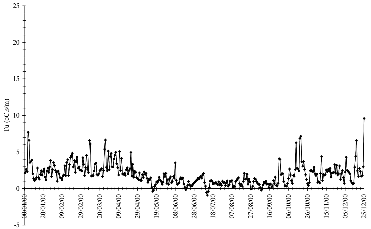
Figure 43 Results for the winter index Tu based on climate model 360 day year for 2000.
