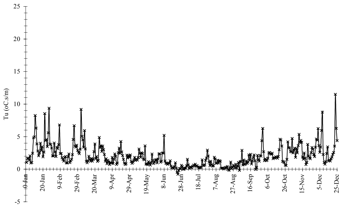
Figure 44 Results for the winter index Tu based on climate model 360 day year for 2010.
