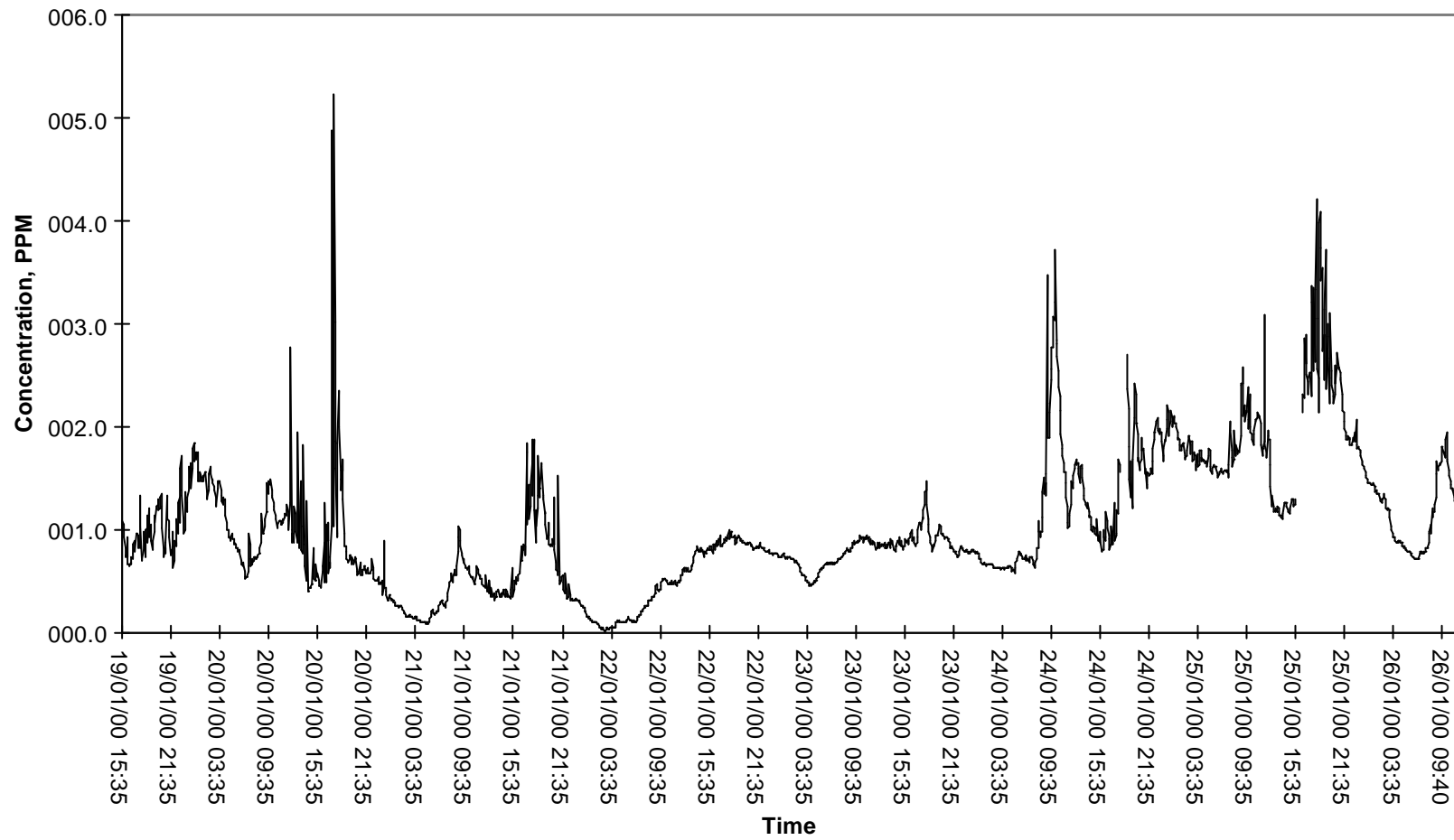
Figure 8 - Time series of CO measurements at Teddington.
