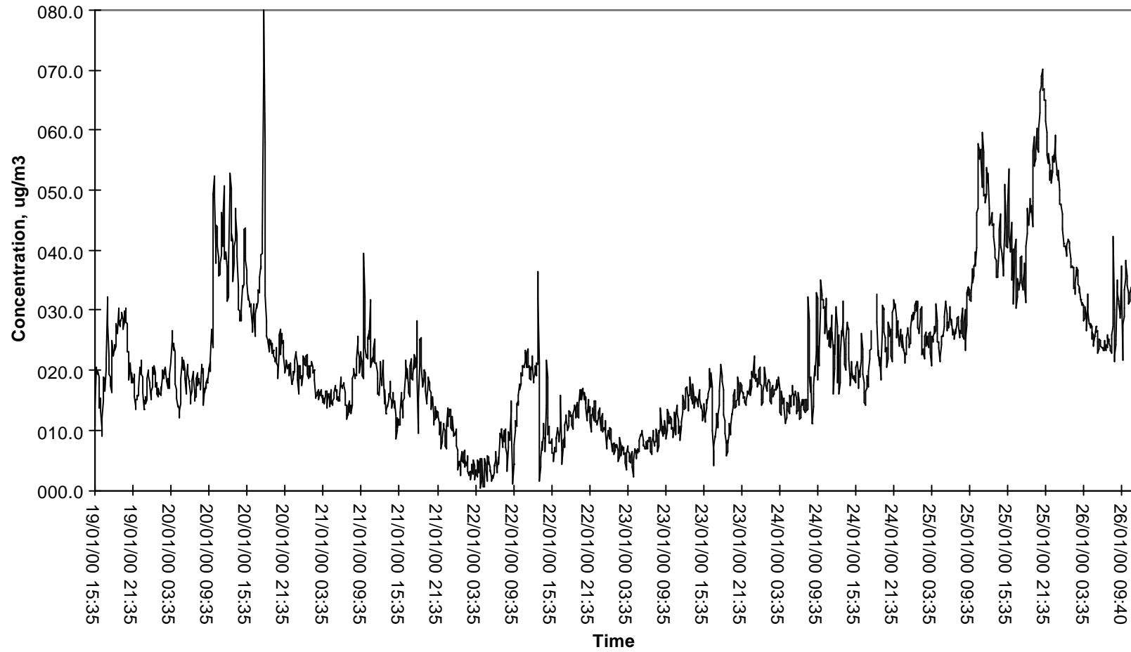
Figure 9 - Time series of PM10 measurements at Teddington.
