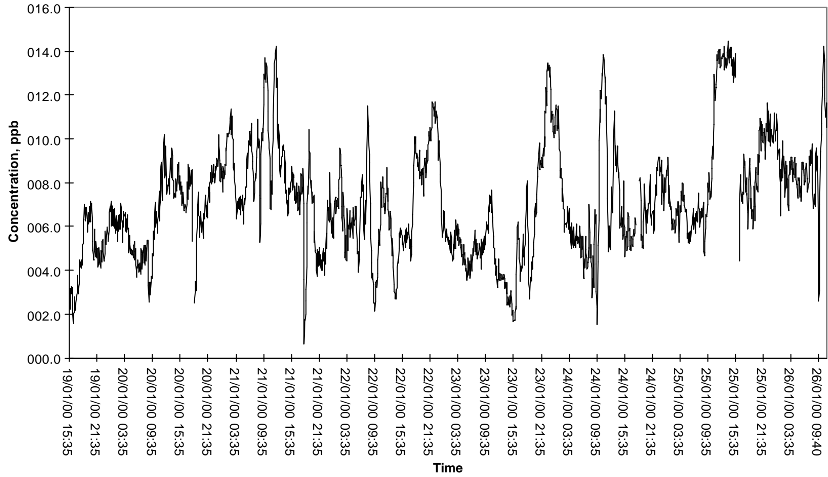
Figure 7 - Time series of SO 2 measurements at Teddington.
