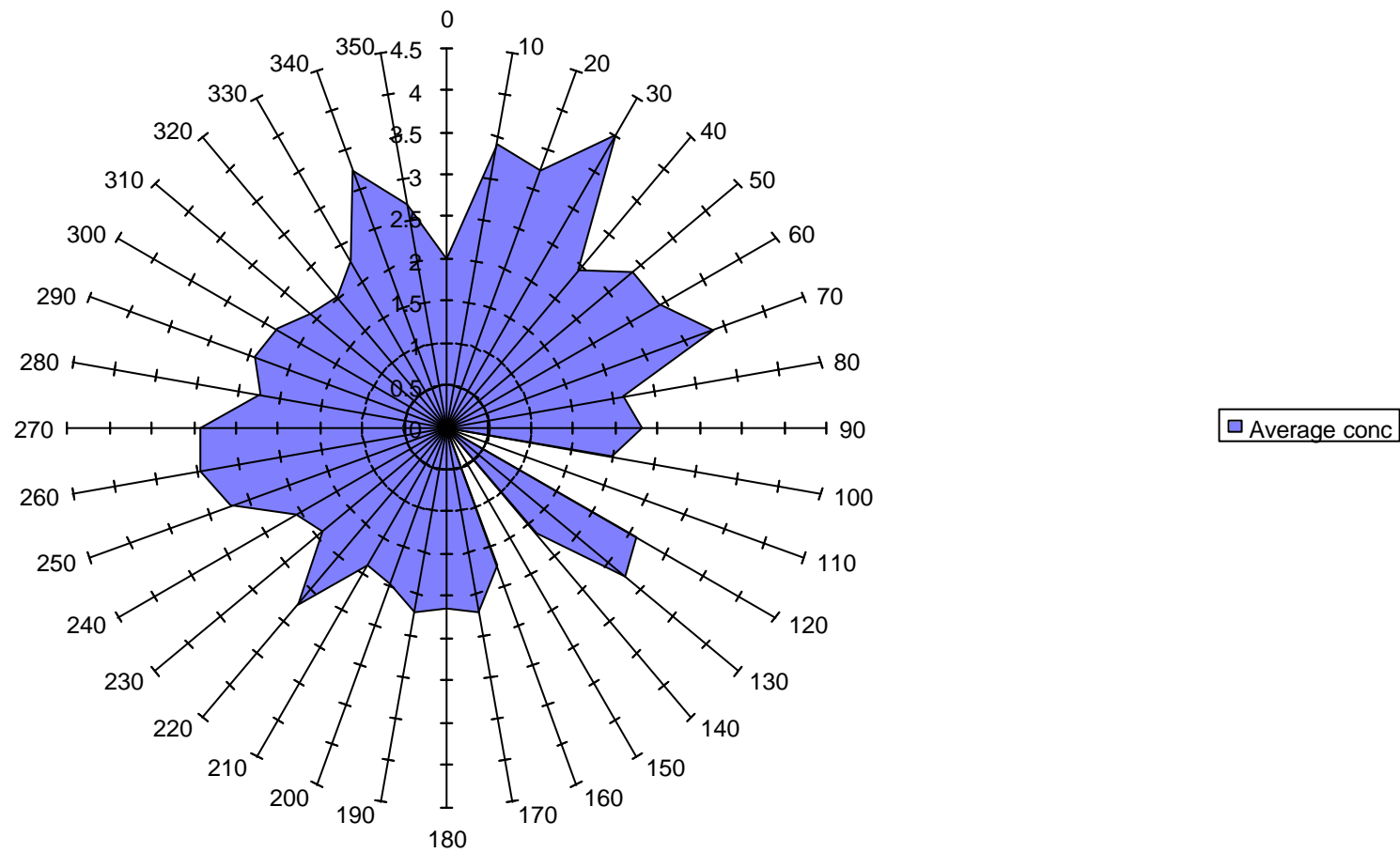
Figure 12 - Wind rose plot for formaldehyde data at Teddington.
