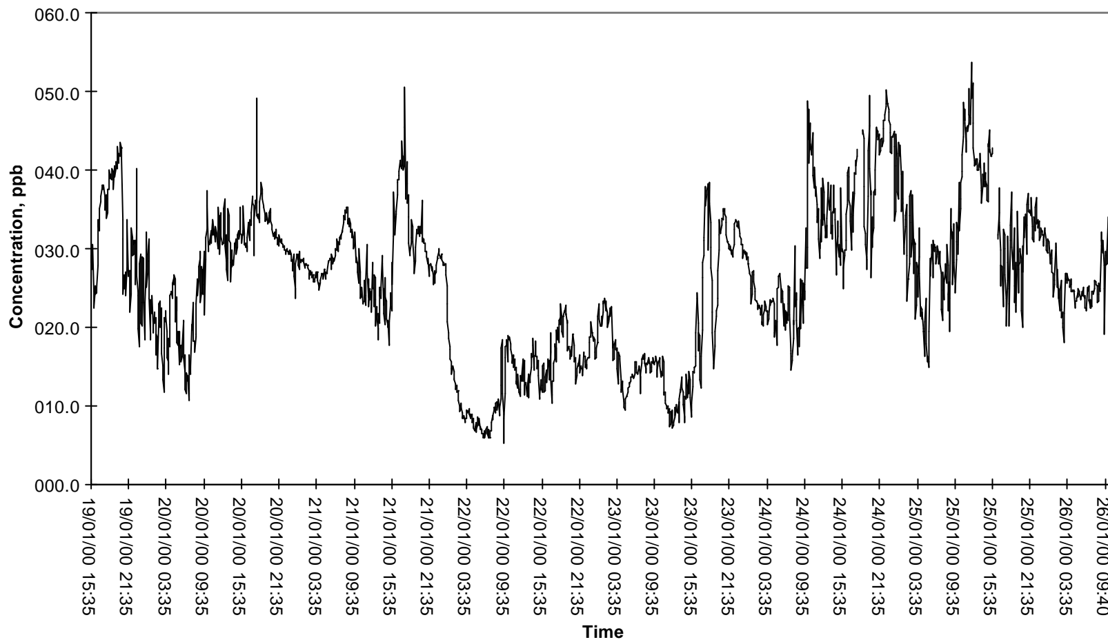
Figure 5 - Time series of NO 2 measurements at Teddington.
