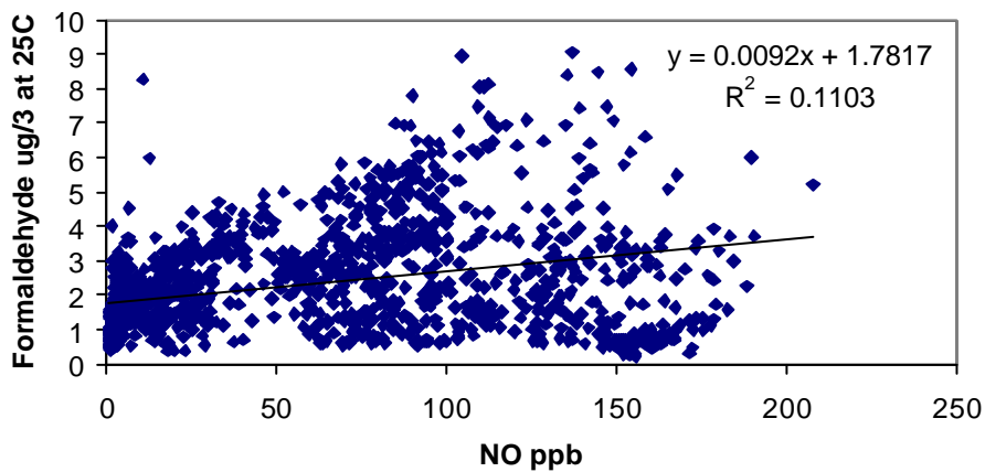
Figure 13 - Correlation between formaldehyde and CO, NO, and NO 2 at Teddington.
