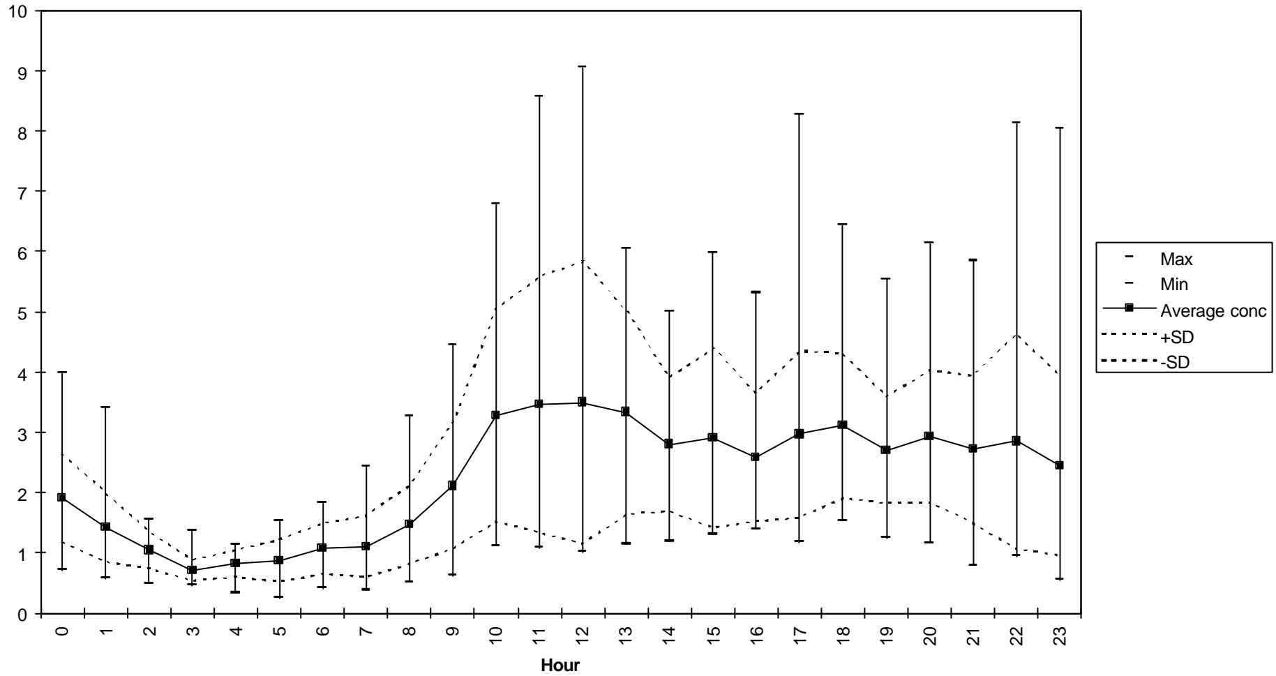
Figure 10 - Diurnal variation in formaldehyde measurements at Teddington.
