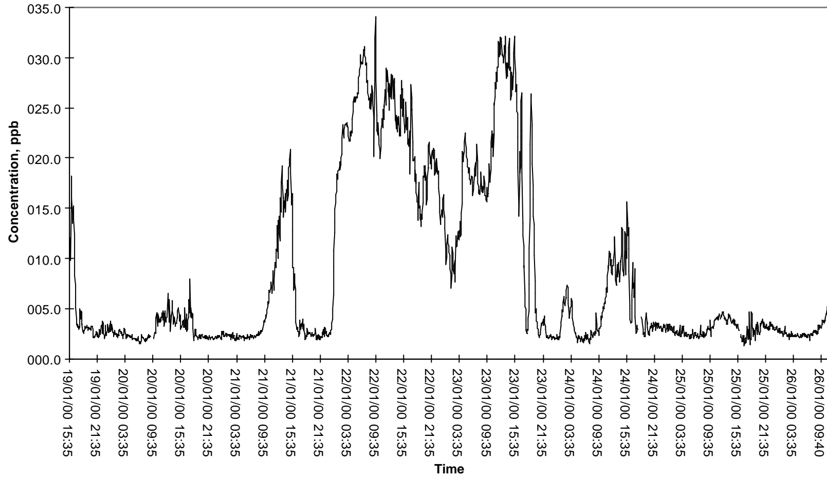
Figure 6 - Time series of O 3 measurements at Teddington.
